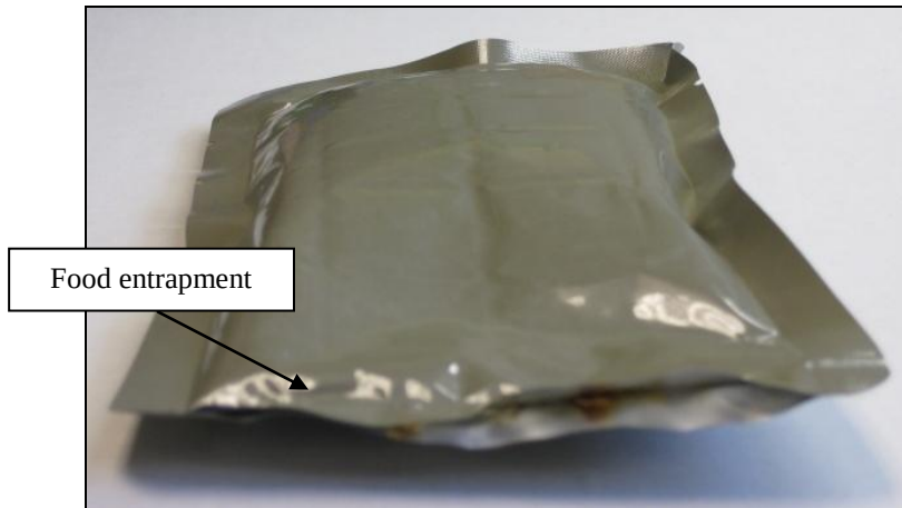
Figure 76. Food Entrapment in Manufactured Seal Resulting in Weakened Seal or Failure.
