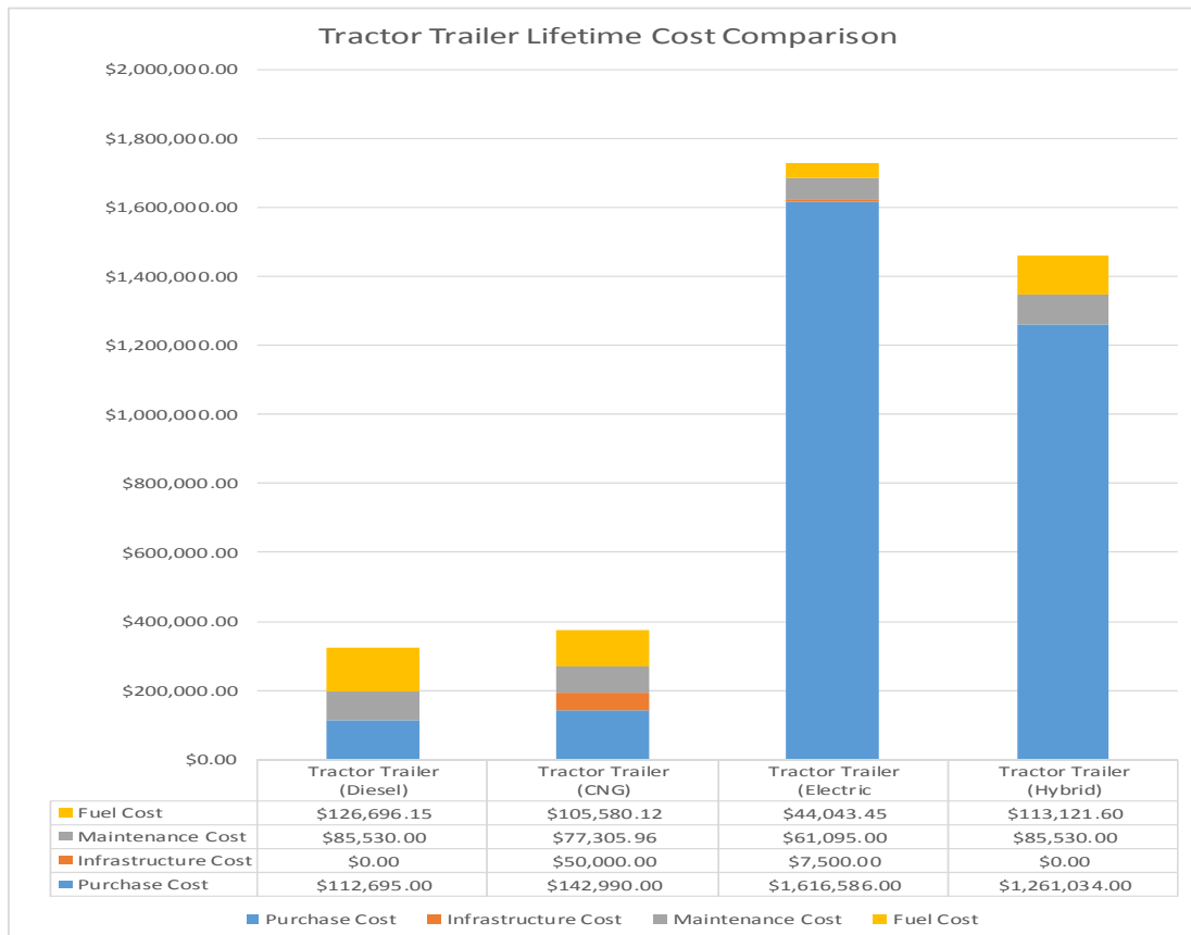
Figure 64. Tractor-trailer Lifetime Cost Comparison
