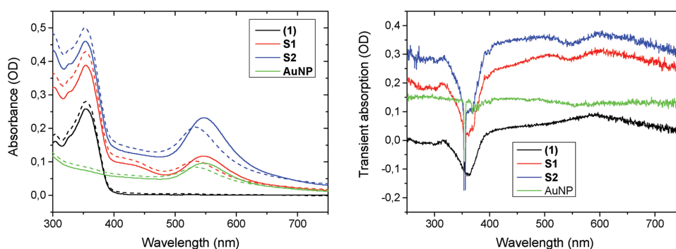
Figure 6. Left: Absorbance of samples for ESA series. (1) denotes solvent with compound (1) only. S1 and S2 had progressively increased AuNP concentration as indicated from the absorption spectra. AuNP denotes solvent with AuNP only (45 nm). Dashed lines are for measurements made after ESA measurements (see comment in text). Right: ESA of the solutes in left panel recorded at 0 s time-delay. The negative spike at 355 nm is residual from the pump-source.
