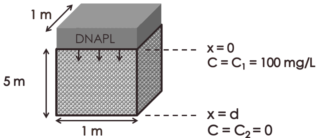
Figure 2.11. DNAPL pool on a unit area of a hypothetical aquitard.
