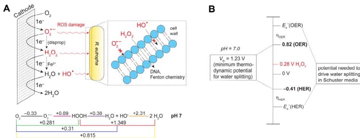
Figure 13 | ROS production. A Schematic of major oxygen reduction reactions at a cathode. The potentials (in volts vs NHE at pH 7.0) for formation of the reactive oxygen species are provided on the Latimer diagram shown in the bottom panel. Generated ROS may cause cell damage at the cell surface or intracellularly (inset). B Water splitting potential shown in the context of additional cell potentials and relative to the potential for H_2O_2 generation. The additional potential associated with solution resistance is not shown.
