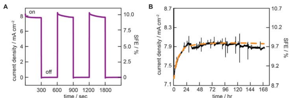
Figure 6 | A Current under chopped illumination representing J_{OP} for the PV-EC device (0.5 M K 2 SO 4 , pH 9.2). The chopped illumination illustrates the recovery in SFE and illustrates the reproducibility in measuring J_{OP} . B J_{OP} measured for over 7 days of operation showing no decrease in SFE over operation time. Spikes J_{OP} are due to addition of solution to maintain the solution level and pH. The orange dashed line is a smoothed curve of the data.
