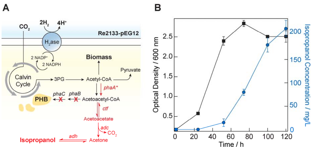
Figure 12 | Bioelectrochemical production of isopropanol. A Schematic diagram of R. eutropha strain Re2133-pEG12 containing an engineered pathway for isopropanol production (red lines, text) and grown on electrochemically produced H_2 and CO_2 . The CoA transferase (ctf) reaction is reversible and coupled to production of succinyl-CoA from succinate. The alcohol dehydrogenase reaction (adh) is also reversible and coupled to proton transfer and NADPH oxidation (not shown). B Growth and isopropanol production in Re2133-pEG12 grown at 3.0 V with a 4 cm^2 CoPi and 4 cm^2 SS304 anode and cathode, respectively. Error bars represent S.E.M., N = 3 independent experiments.
