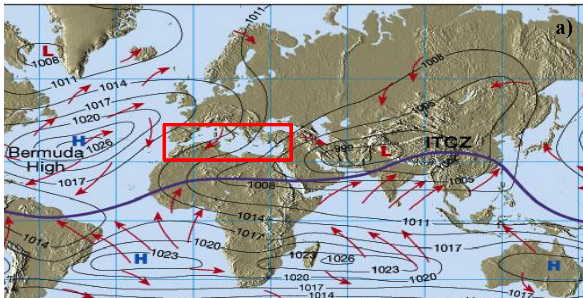
Figure 5. a) Pressure Systems and Associated Circulation Patterns in July, b) 1,000 mb Level Specific Humidity (g/kg) for Summer 1981–2010.
