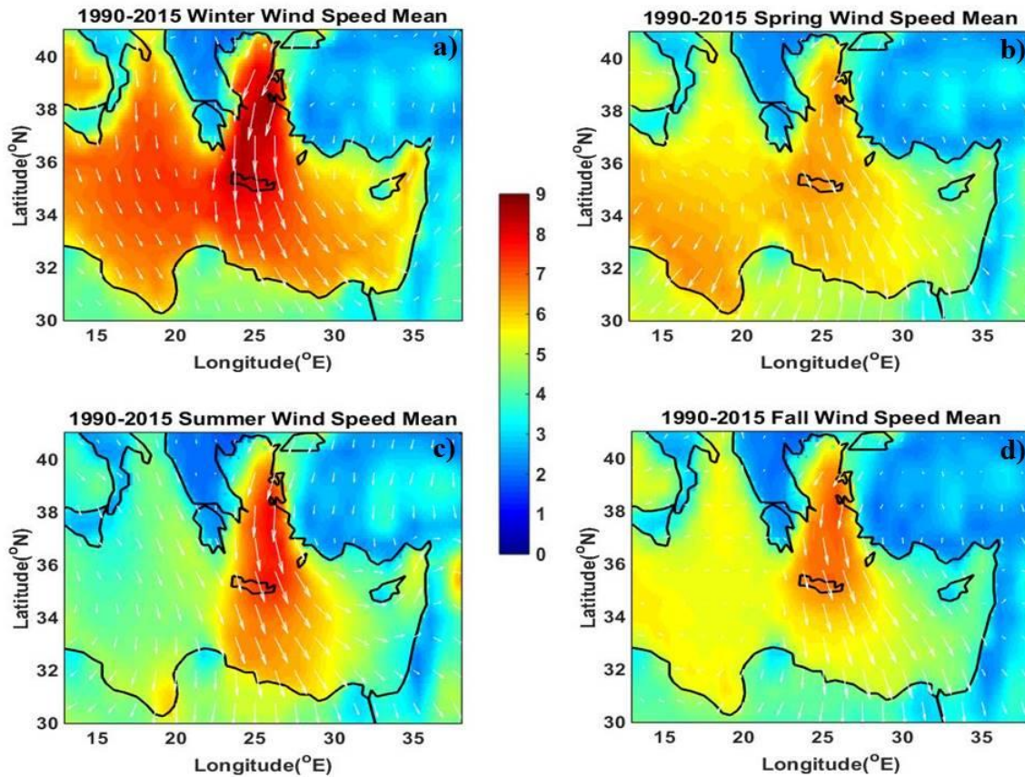
Figure 24. 1990–2015 Seasonal Means of Wind Speed in m/s for a) Winter, b) Spring, c) Summer, and d) Fall.
