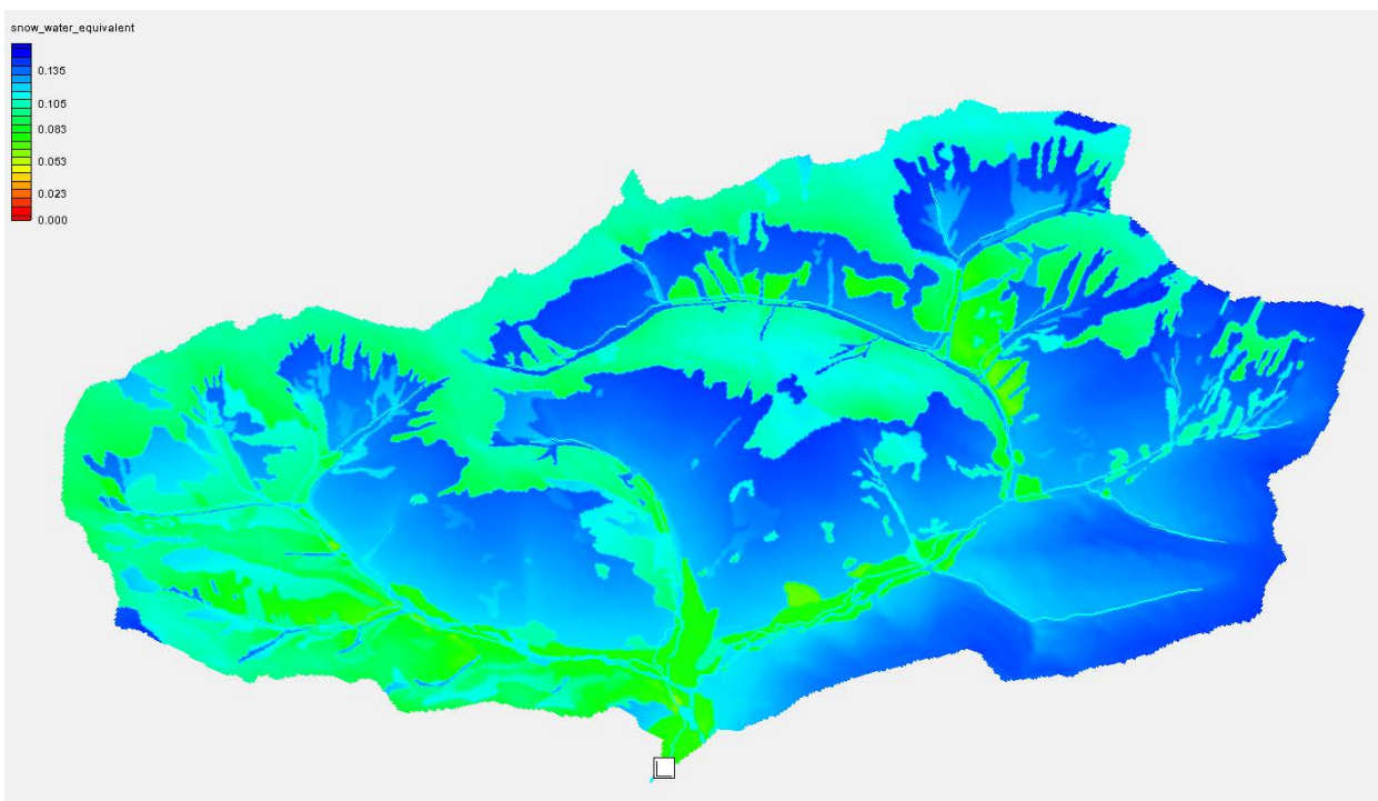
Figure 53. Simulated SWE distribution on 4 April 2011 at the Caribou-Poker Creek Research Watershed.
