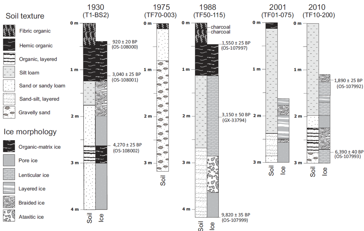
Figure 20. Soil texture, permafrost ice morphology, and radiocarbon dates with depth at one representative borehole from each fire scar. Site and radiocarbon sample IDs are in parentheses.
