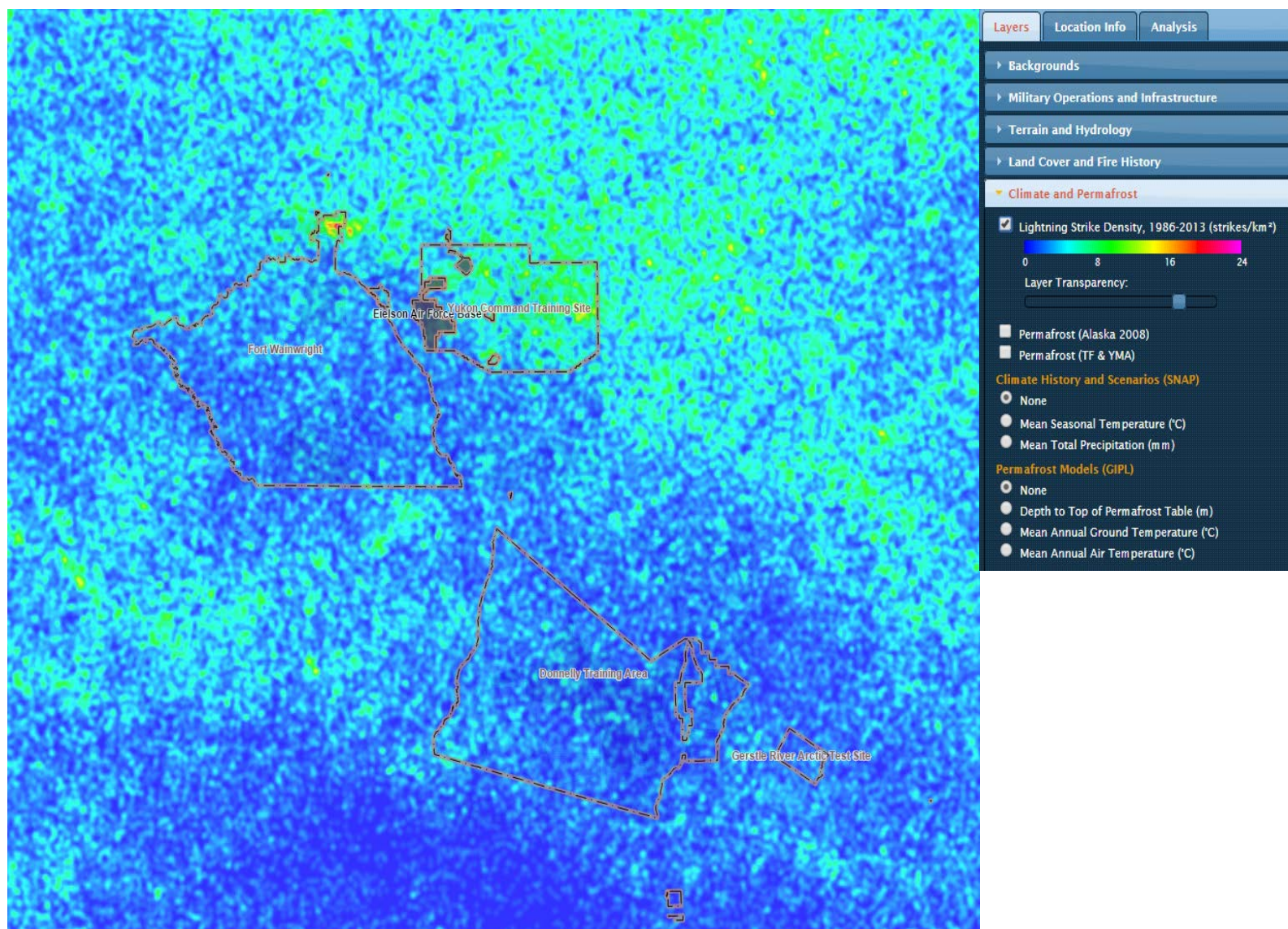
Figure 72. Lightning strike density from 1986 to 2013.
