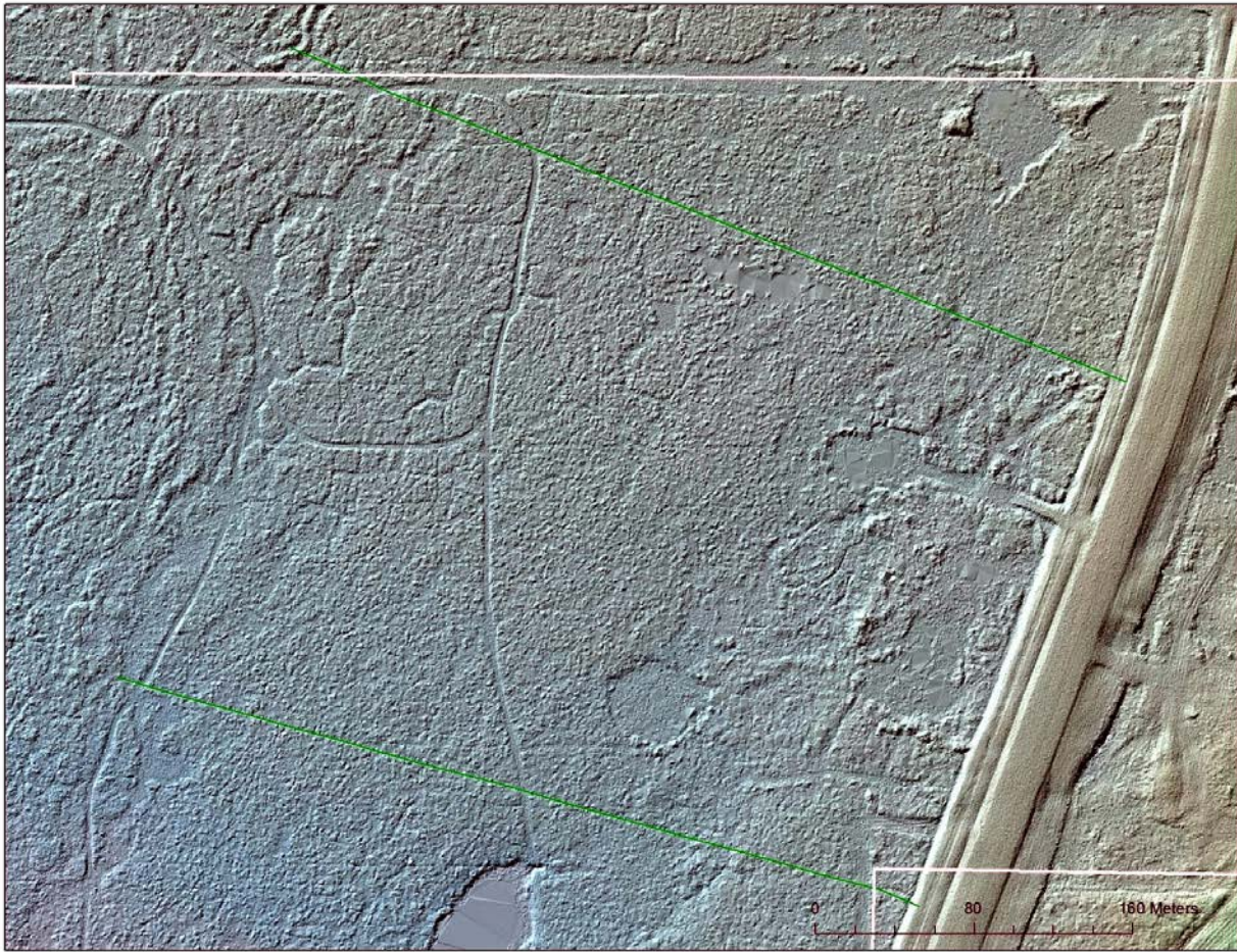
Figure 78. Airborne LiDAR at a permafrost monitoring transect near Fairbanks, Alaska.
