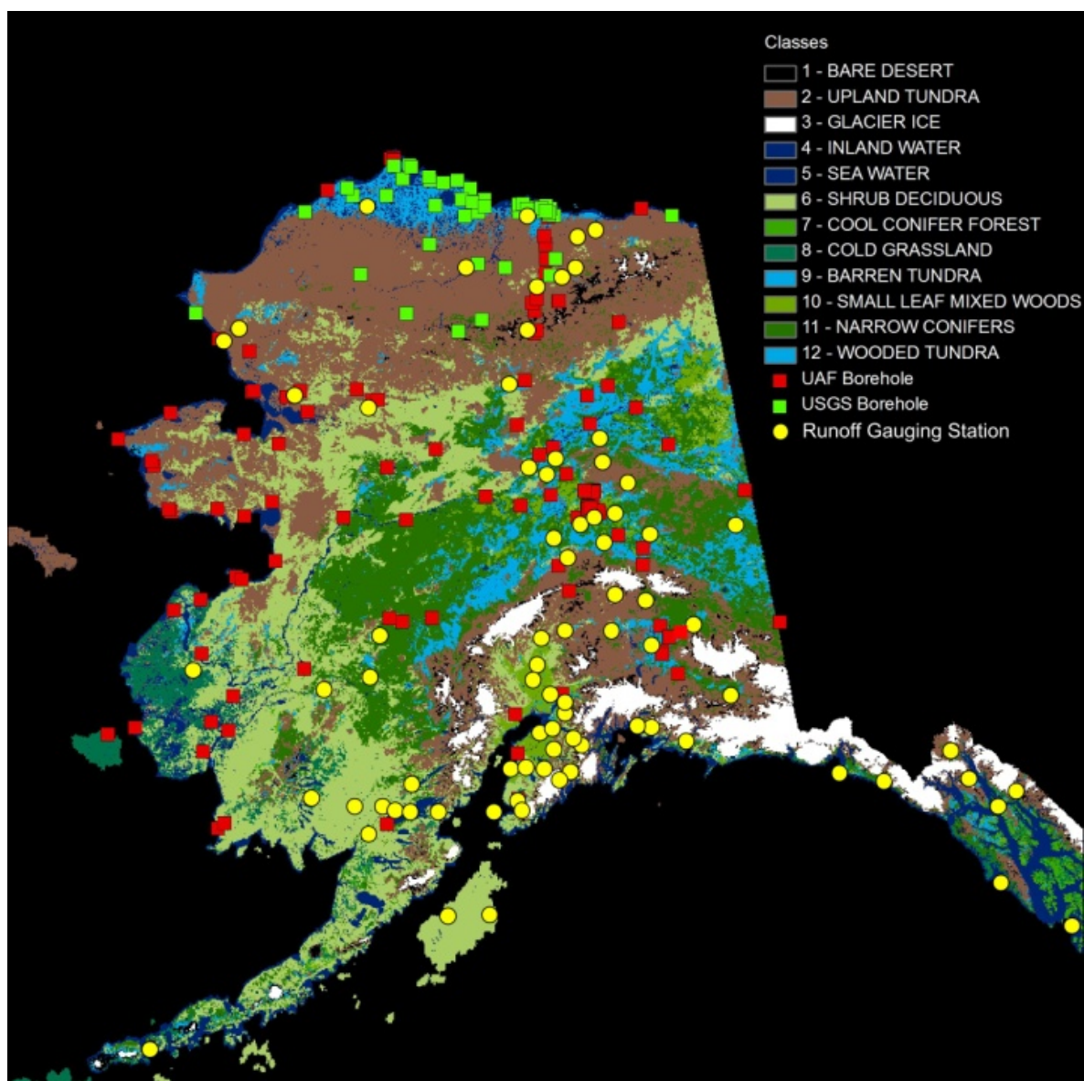
Figure 43. Landscape types and locations of available data used to calibrate the GIPL model.
