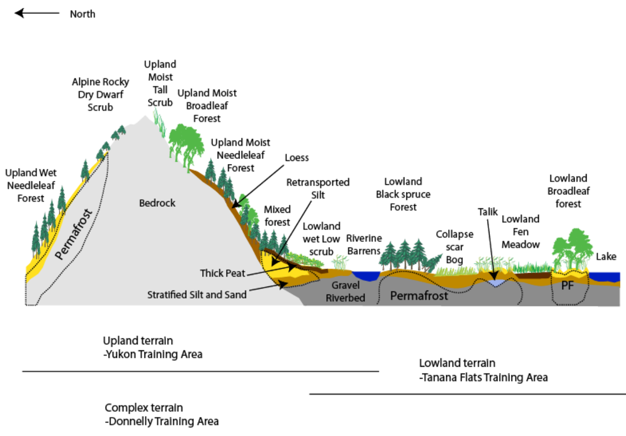
Figure 8. A cross section illustrating the physiographic variety of land forms, hydrologic features, and vegetation in interior Alaska and their relationship to permafrost. Adapted from Jorgenson et al., 2010 as published in Douglas et al., 2014.
