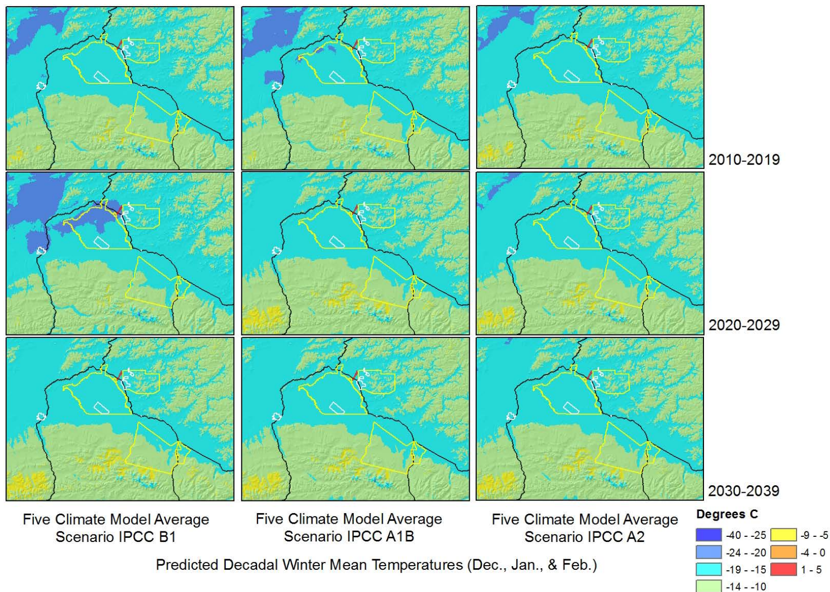
Figure 66. Downscaled projected decadal winter (December-February) mean temperatures for interior Alaska. U.S. Army Corps of Engineers project lands are outlined in red, Army lands are delineated by yellow, and Air Force lands are marked by white.
