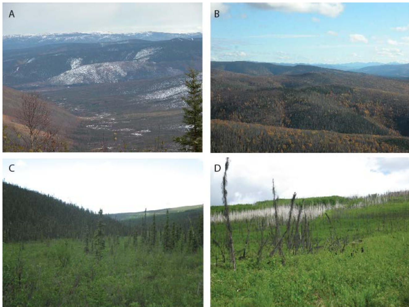
Figure 6. Photographs representing the vegetation typical of upland ecosystems found in the Yukon Training Area and in the Caribou-Poker Creeks research Watersheds (CPCRW). A) A winter view of the Stuart Creek impact area on Yukon Training Area showing the rolling hills and elevation gradients. B) A close up of the hills above Stuart Creek in late fall. C) A valley bottom underlain by discontinuous permafrost with a spruce forest at the CPRW. D) A side hill in upland terrain that shows standing dead trees (white colored crowns) from a fire in 1999 in the CPRW.
