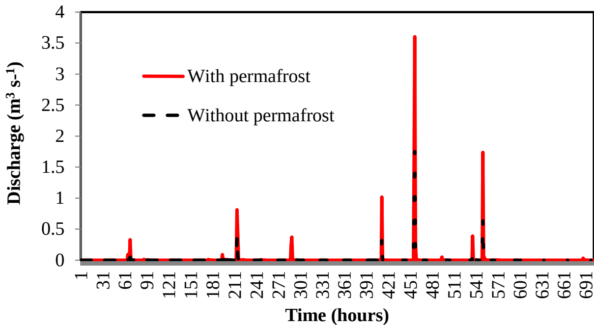
Figure 57. Hydrograph with and without active permafrost.
