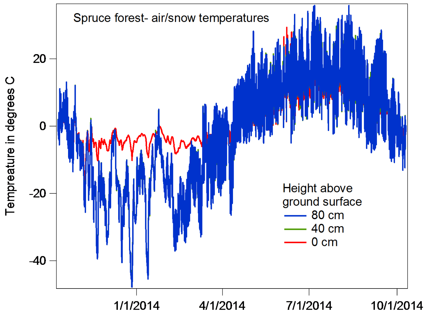
Figure 82. A full year of air and snow temperature measurements at a permafrost monitoring transect near Fairbanks, Alaska. The measurements are made from a rod extending above the ground surface. When there is no snow the measurements are of ambient air. When the snow reaches the height of the thermistor location on the rod the snowpack temperature is measured at that depth.
