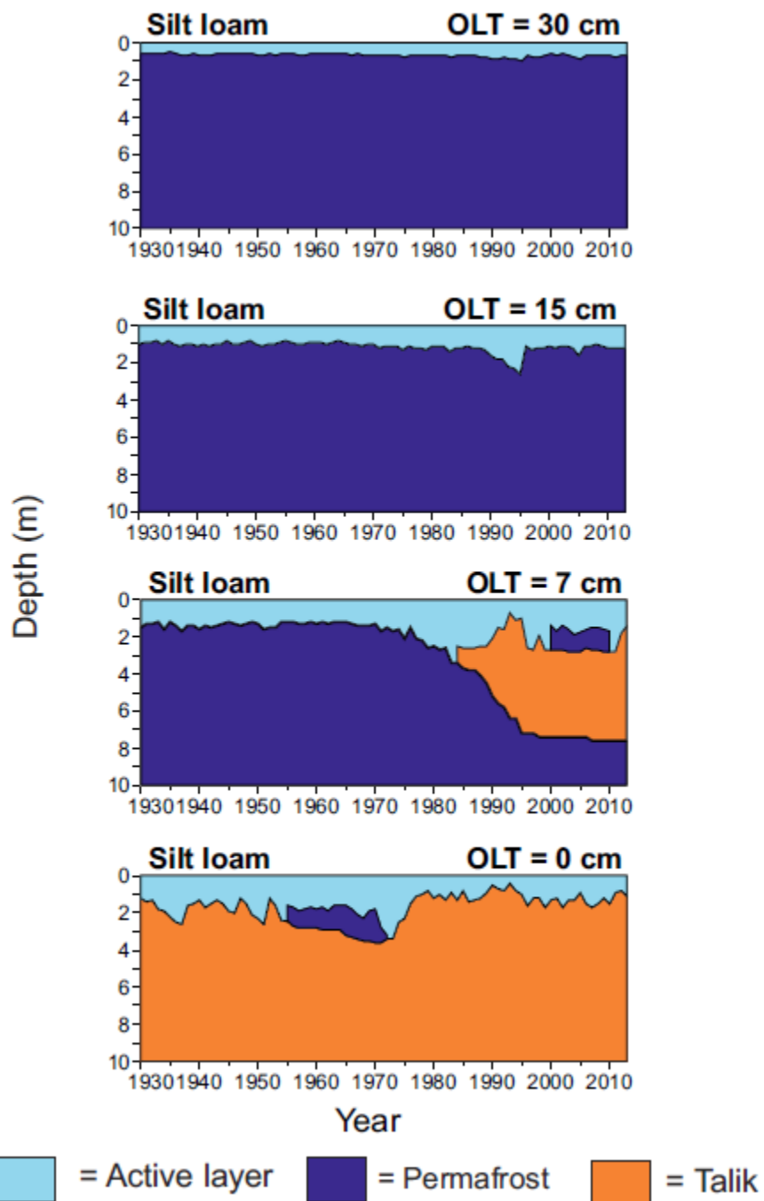
Figure 27. Simulated active layer, permafrost, and talik depths from 1930 - 2013 in silt loam-dominated sites with varying levels of organic layer thickness (OLT).
