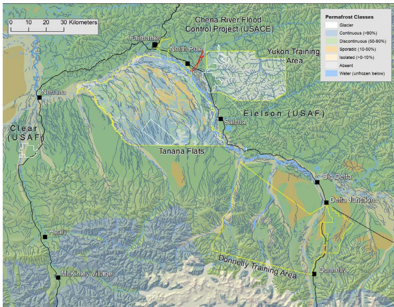
Figure 4. The extent and type of permafrost for interior Alaska DoD lands. U.S. Army Corps of Engineers project lands are outlined in red, Army lands are delineated by yellow, and Air Force lands are marked by white. Permafrost classes range from continuous to absent. Data sources for permafrost are varied with the majority from Jorgenson et al. (2008a) and from the fine scale maps of Tanana Flats and the Yukon Training area in Jorgenson et al. (1999). The spatial distribution of permafrost outside of the Tanana Flats and Yukon Training areas is not well mapped and is largely uncertain. Map from Douglas et al., 2014.
