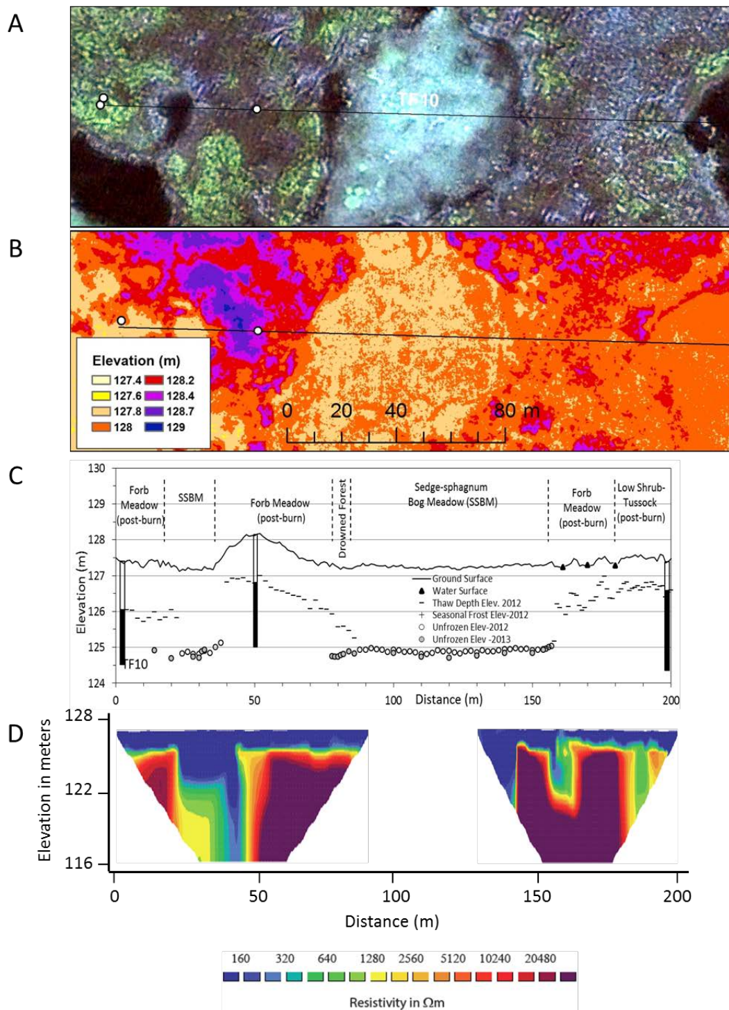
Figure 33. A: An aerial image of the 2010 fire scar. B: airborne LiDAR imagery, shaded by elevation, for the same region presented in the upper panel. The bold line indicates the location and length of the transect at the site while circles denote locations where SIPRE cores were collected. C: A detailed cross section of the vegetation, ground elevation, SIPRE core depths, seasonal thaw depths, and elevations of unfrozen material across the transect. D: electrical resistivity tomography survey results across the transect.
