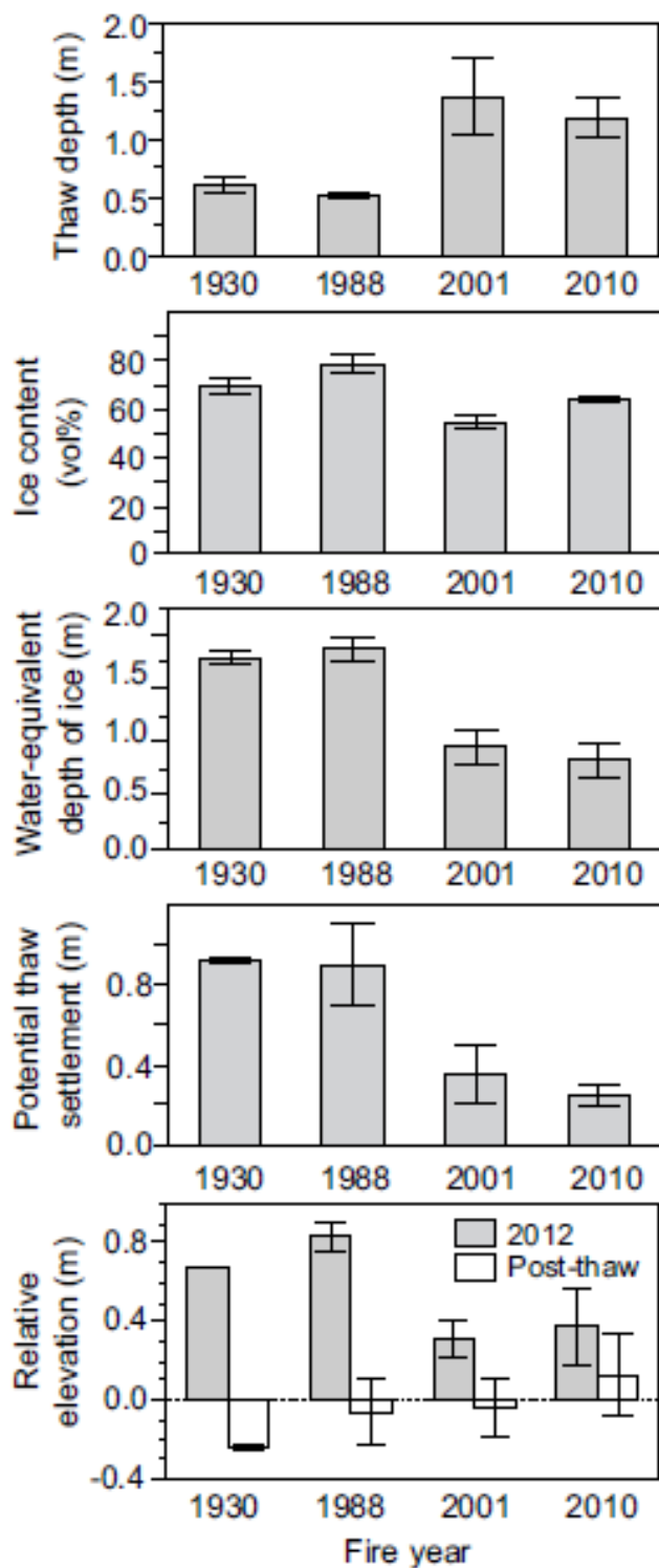
Figure 22. Thaw depth, permafrost ice content, water equivalent depth of ice in permafrost, potential thaw settlement, and elevation at time of sampling (2012) and predicted post-thaw elevation of the ground surface relative to the surface water level. Values represent means \pm SE ( n = 12 ). Permafrost characteristics and subsequent calculations of thaw settlement and relative elevation changes are based on the upper 3 m of the soil column.
