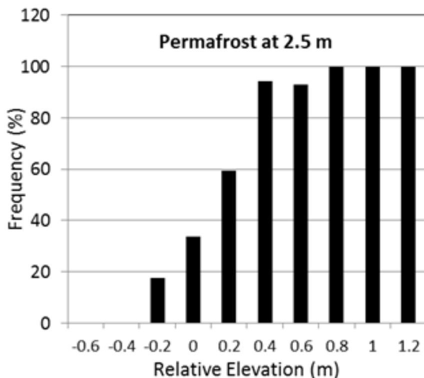
Figure 42. A histogram of the percentage frequency of permafrost extent and the relative elevation across the 11 ecotypes present at the fire scars.
