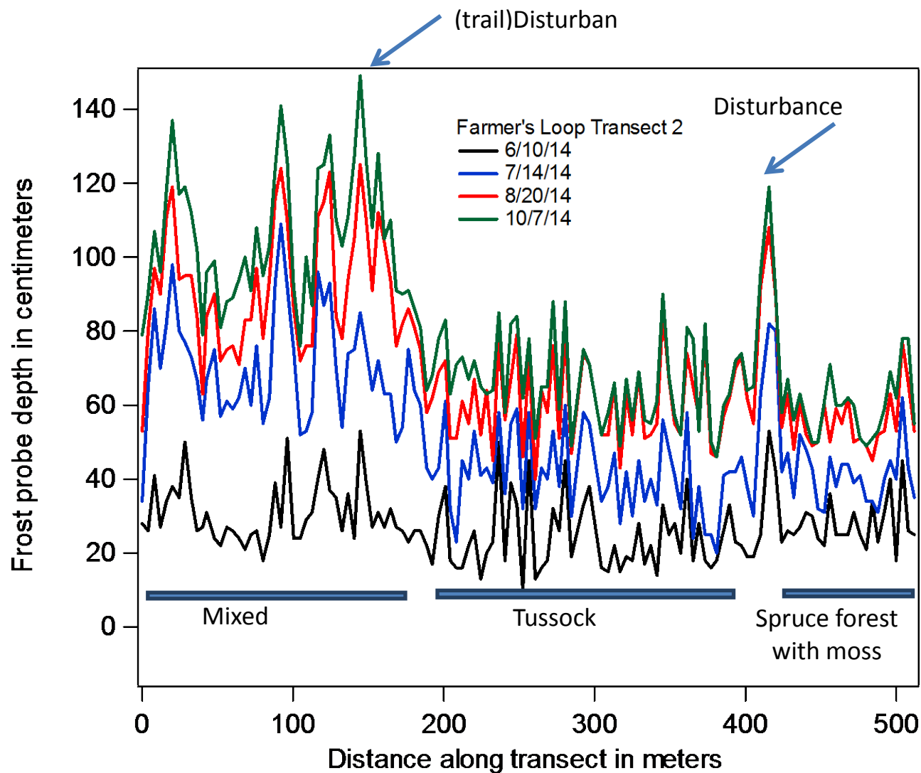
Figure 79. Repeat seasonal thaw depth measurements at a permafrost monitoring transect near Fairbanks, Alaska. Note the downward movement of the seasonal thaw (i.e. increasing depth values) over time. Also note the relationship between vegetation cover and seasonal thaw. The two locations where disturbance is noted are trails that have been cleared of vegetation and this has caused extensive seasonal thaw.
