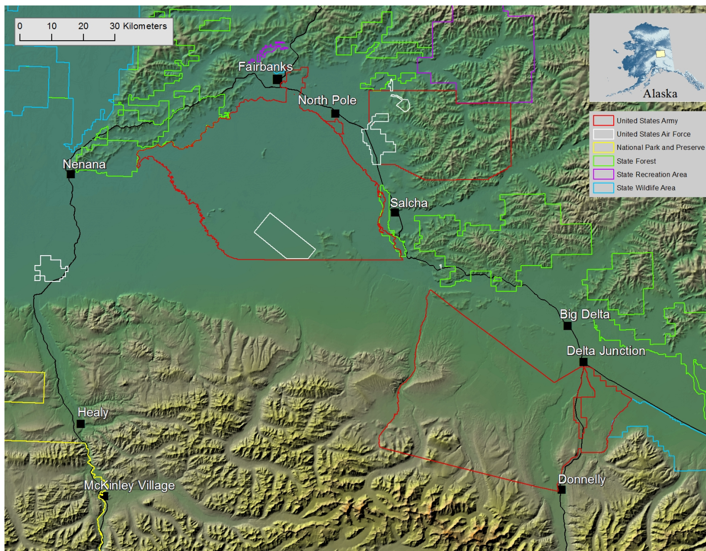
Figure 2.A terrain elevation map of interior Alaska with boundaries for the major Federal and State land managers.
