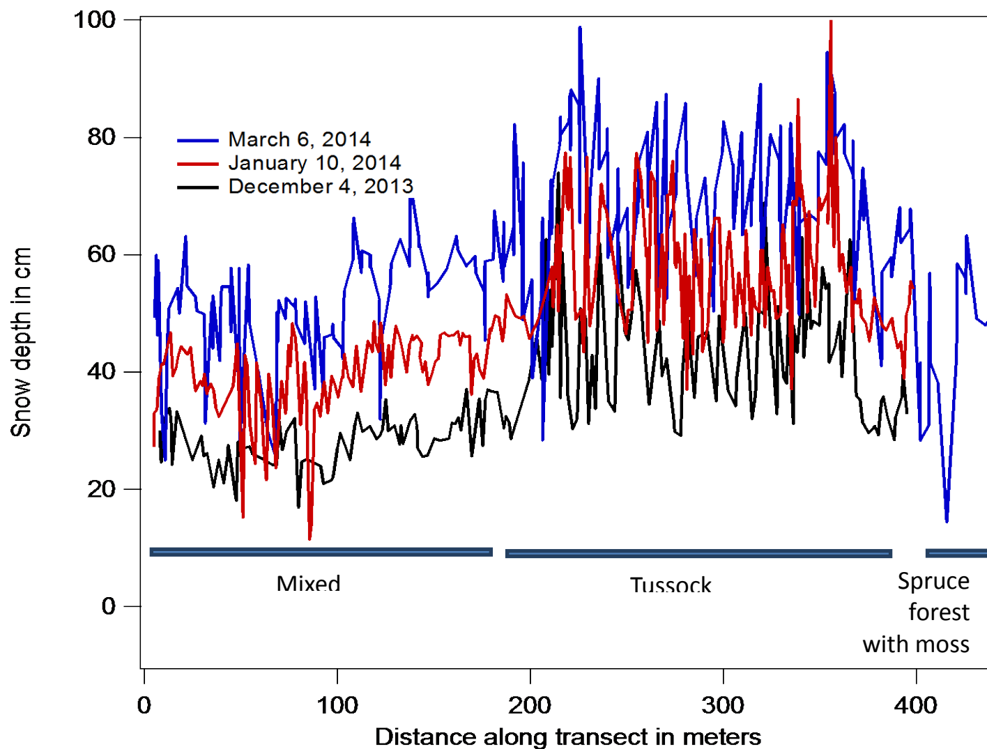
Figure 83. Repeat snow depth measurements at a permafrost monitoring transect near Fairbanks, Alaska. Note the strong relationship to vegetation cover.
