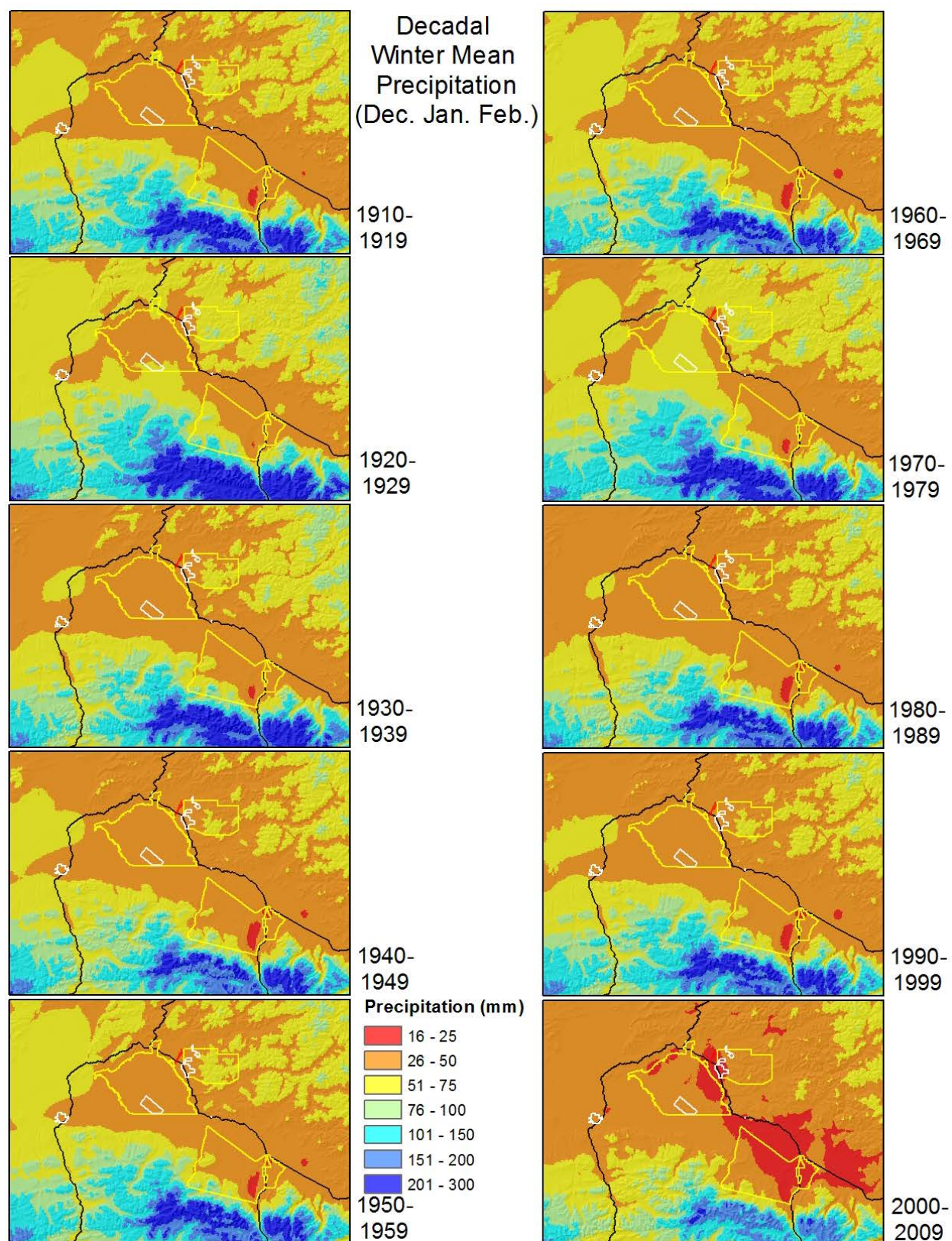
Figure 67. Decadal winter (December-February) total precipitation for interior Alaska shows a general decline from one decade to another. U.S. Army Corps of Engineers project lands are outlined in red, Army lands are delineated by yellow, and Air Force lands are marked by white.
