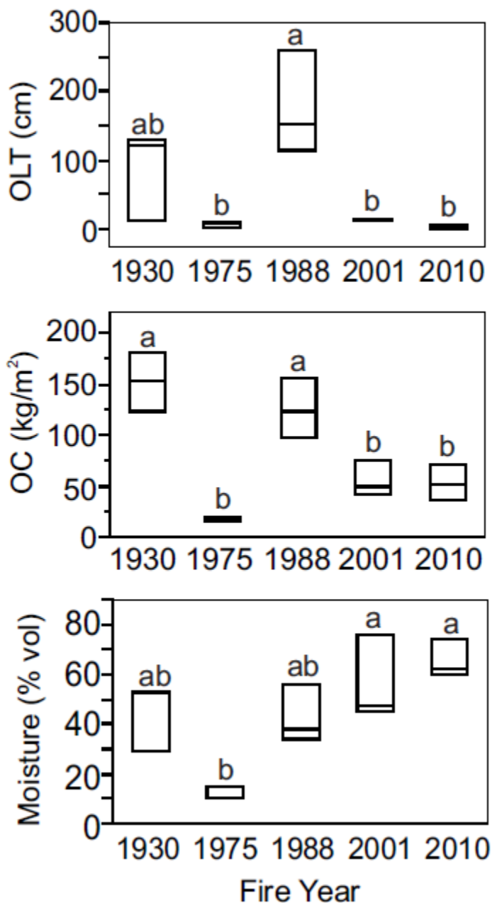
Figure 21. Box plots of organic layer thickness, organic carbon stocks (to 3 m depth), and active layer soil moisture by fire year ( n = 14 ) with Tukey-Kramer post-hoc results of significant differences ( p < 0.05 ) depicted by lettering.
