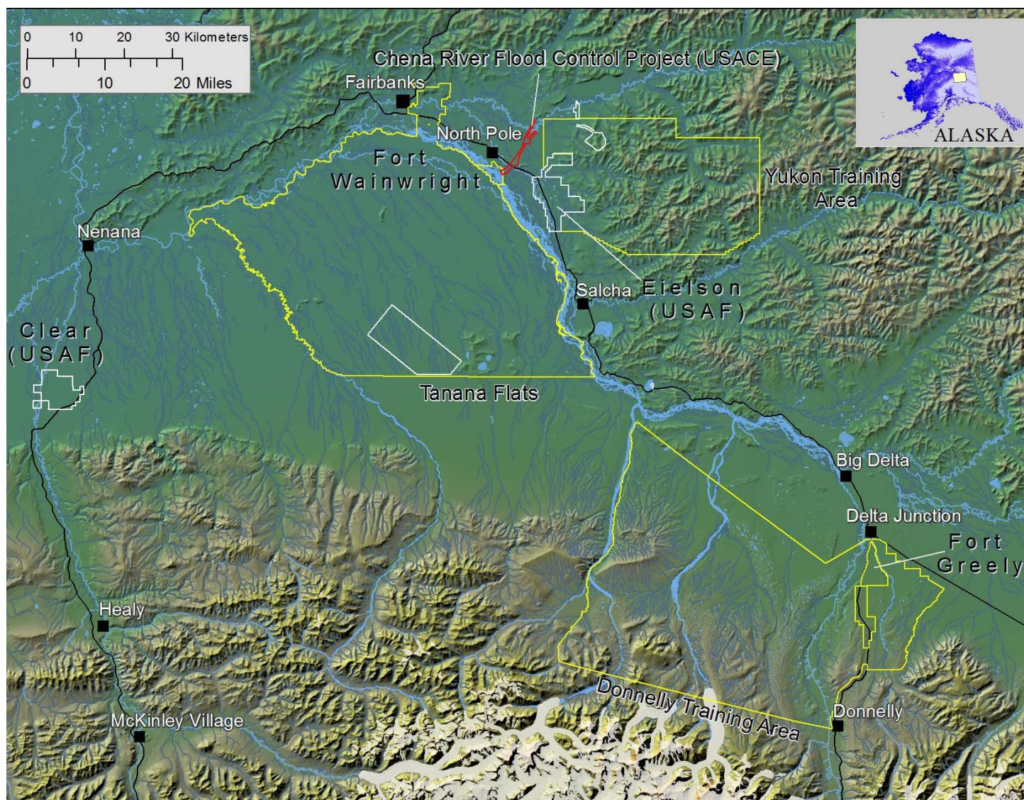
Figure 1. A terrain elevation map of interior Alaska with boundaries for the major Department of Defense facilities. U.S. Army cantonments and training lands (yellow outline), Air Force facilities (white outline) and U.S. Army Corps of Engineers project land (red outline) are identified.
