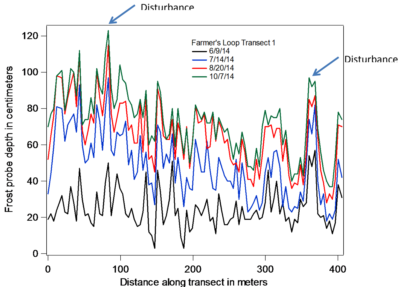
Figure 80. Repeat seasonal thaw depth measurements at a permafrost monitoring transect near Fairbanks, Alaska. Note the downward movement of the seasonal thaw (i.e. increasing depth values) over time. The two locations where disturbance is noted are trails that have been cleared of vegetation and this has caused extensive seasonal thaw.
