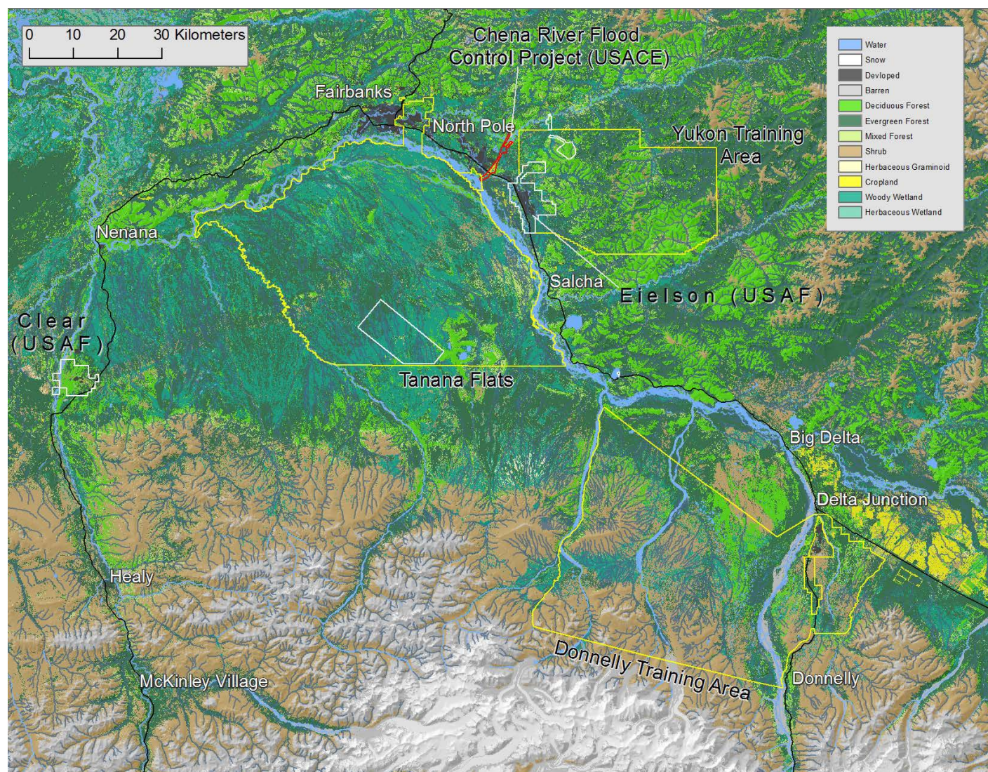
Figure 3. Predominant land cover classes for the Tanana Flats and surrounding areas of interior Alaska from the Alaska 2001 National Land Cover Database(Homer et al., 2007) include evergreen (34%) and deciduous (12%) forest, shrubland (24%), woody wetland (13%), and barren (7%). Percentages are calculated from DoD-owned lands within the visible domain. U.S. Army Corps of Engineers project lands are outlined in red, Army lands are delineated by yellow, and Air Force lands are marked by white.
