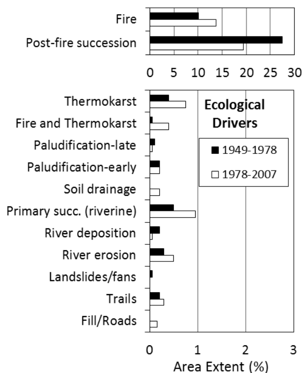
Figure 60. Comparison of the areal extent affected by 13 drivers of ecotype changes. Note difference in scales between charts.
