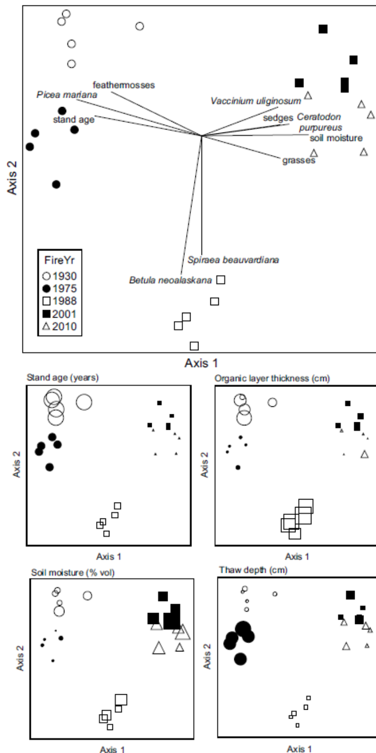
Figure 19. Nonmetric multidimensional scaling ordination of vegetation plots by fire year (upper large panel) and correlations of ordination axes with cover of plant species/functional type and site variables (lower small panels). The direction and length of a given vector represents the direction and strength of correlations. Symbols in the lower panels are scaled to individual site variables.
