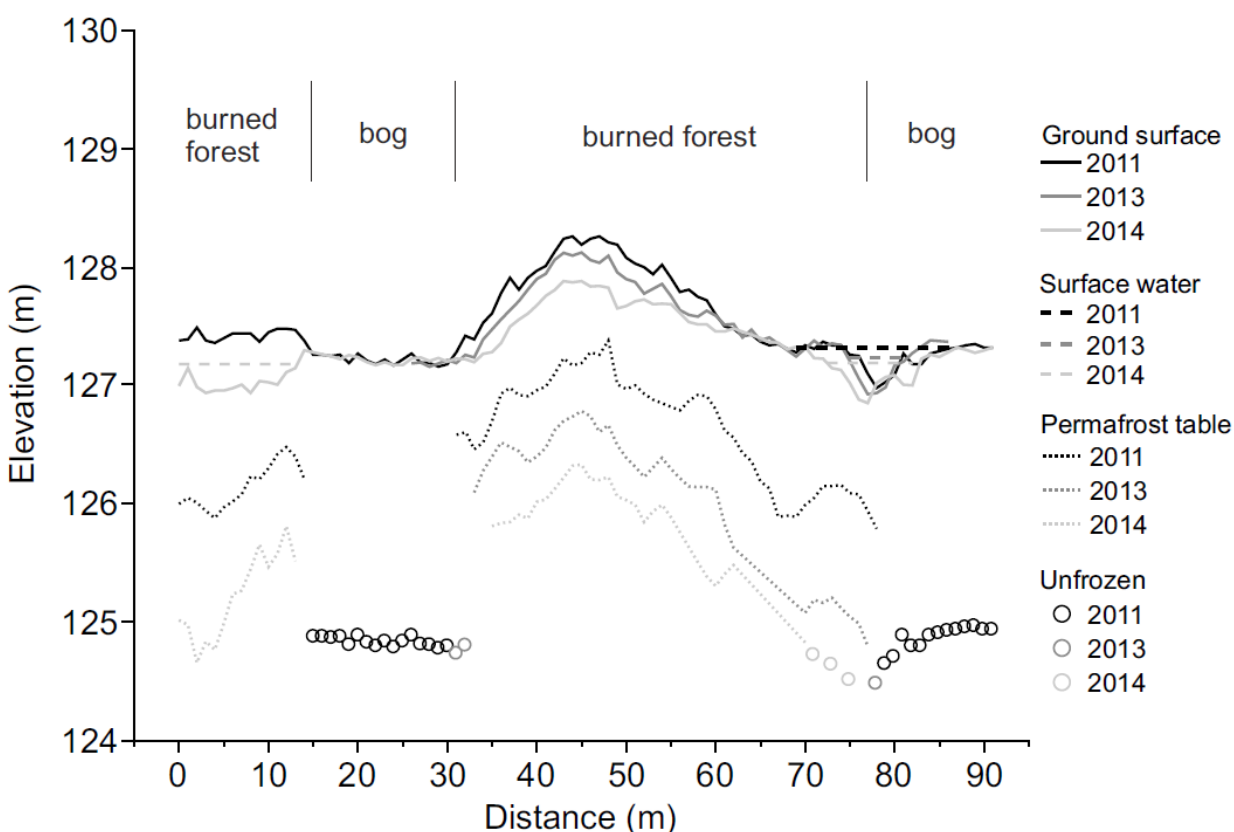
Figure 23. Cross-section of the 2010 fire transect through burned black spruce forest and collapse-scar bogs, showing the elevations (m) of the ground surface, surface water, permafrost table, and maximum observed depths of unfrozen ground in 2011, 2013, and 2014. Note that there is a data gap from 0-35 m for 2013. Another collapse-scar bog is present ~10 m before the beginning of the transect.
