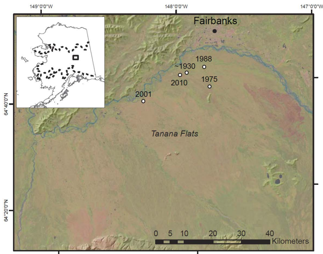
Figure 11. Map of the study sites (named by fire year) overlain on satellite image and digital elevation model, with inset showing location of the Tanana Flats study area within the discontinuous permafrost zone of Alaska (dashed lines; Jorgenson et al. 2008a). The Landsat 8 image (acquired June 18, 2013) is displayed as a color composite of bands 6 (SWIR), 5 (NIR), and 4 (red).
