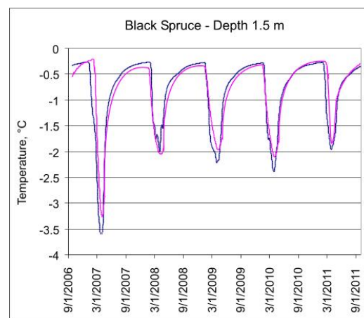
Figure 44. Landscape settings (A, B) and examples of the temporal calibration of the GIPL model (C, D, E, F) for one specific site in a black spruce forest interior Alaska. In D, E, and F the blue and pink lines represent measurements from two locations at the site.
