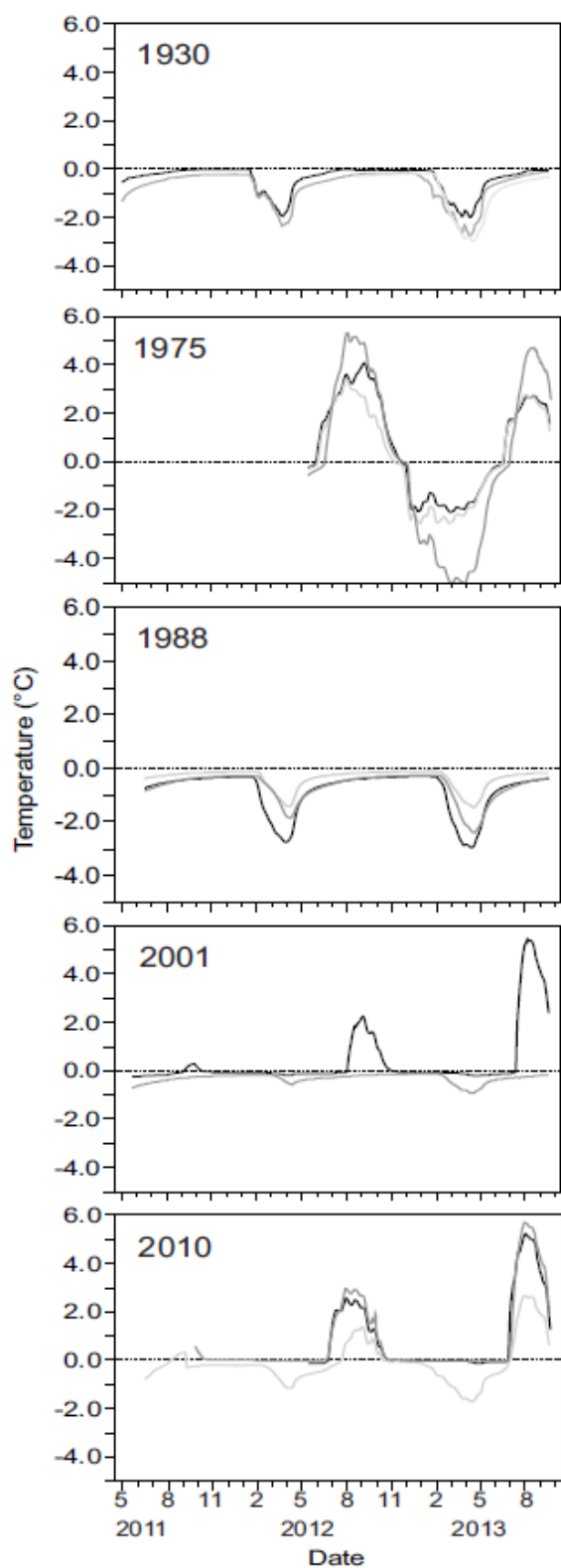
Figure 26. Measured daily soil temperatures at 1 m depth for all sites within each fire scar. The x-axis tick marks depict the first day of each month. The dotted reference line shows 0°C.
