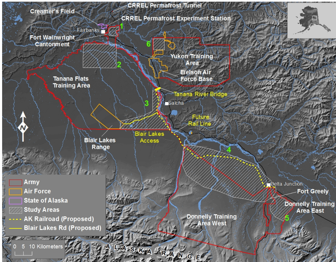
Figure 7. A terrain elevation map delineating Army, Air Force, and State of Alaska lands in interior Alaska with a focus on proposed JPARC infrastructure investments. The Alaska Railroad's recently constructed $185M Tanana River Bridge, the planned access road to the Air Force Blair Lakes site, and a future road and rail corridor to Fort Greely are denoted.
