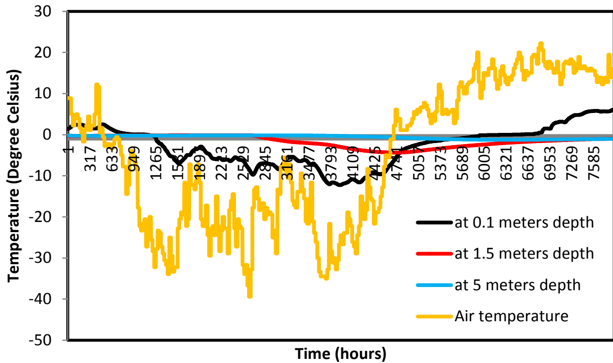
Figure 56. Time series of temperature at various depths.
