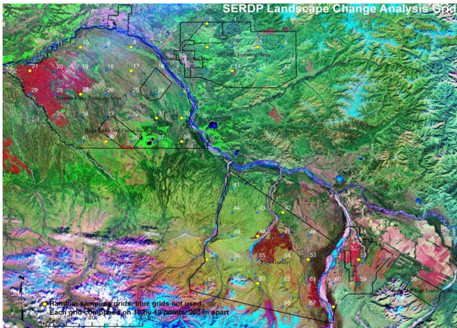
Figure 15. Sampling grid used for assessing landscape change within the Tanana Flats Training Area, Yukon Training Area, and Fort Greely. Blue and yellow circles denote the centers of the grid cells that comprise all interior Alaska DoD installation and training range lands. Yellow circles include a subset of locations where the landscape change measurements were focused.
