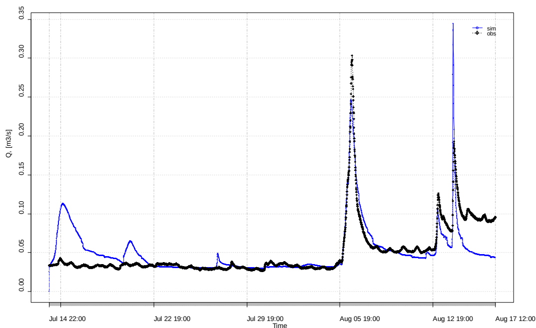
Figure 51. An example validation period for the C2 sub-basin discharge provides a comparison of simulated flow (blue line) with observed discharge over a month long period
