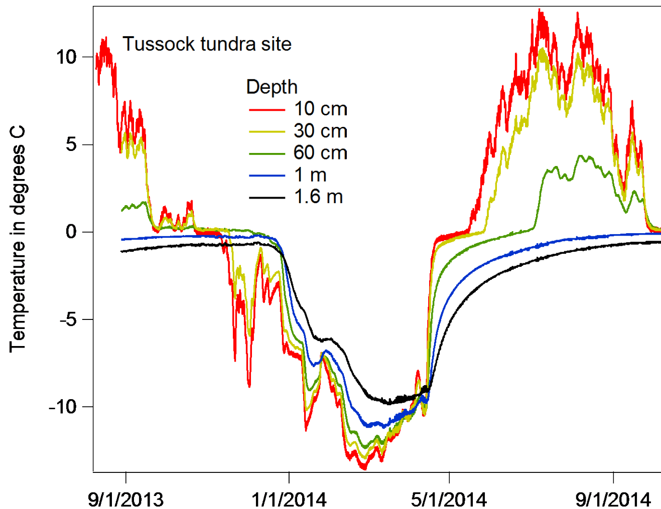
Figure 81. A full year of soil temperatures with depth measured at a permafrost monitoring transect near Fairbanks, Alaska. Seasonal thaw depths at this location is about 80 cm.
