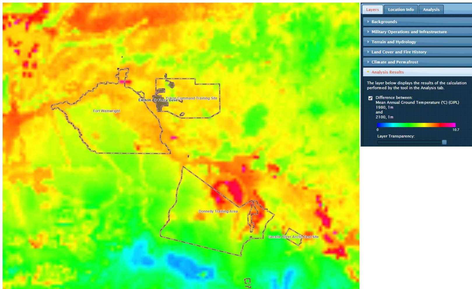
Figure 70. A comparison of mean annual ground temperature at 1 meter calculated for 1980 to projected mean annual ground temperatures in 2100 at 1 m depth. The resulting information shows the projected amount of warming from 1980 to 2100. Note that upland regions are projected to experience the greatest increase in ground temperatures (up to 10°C).
