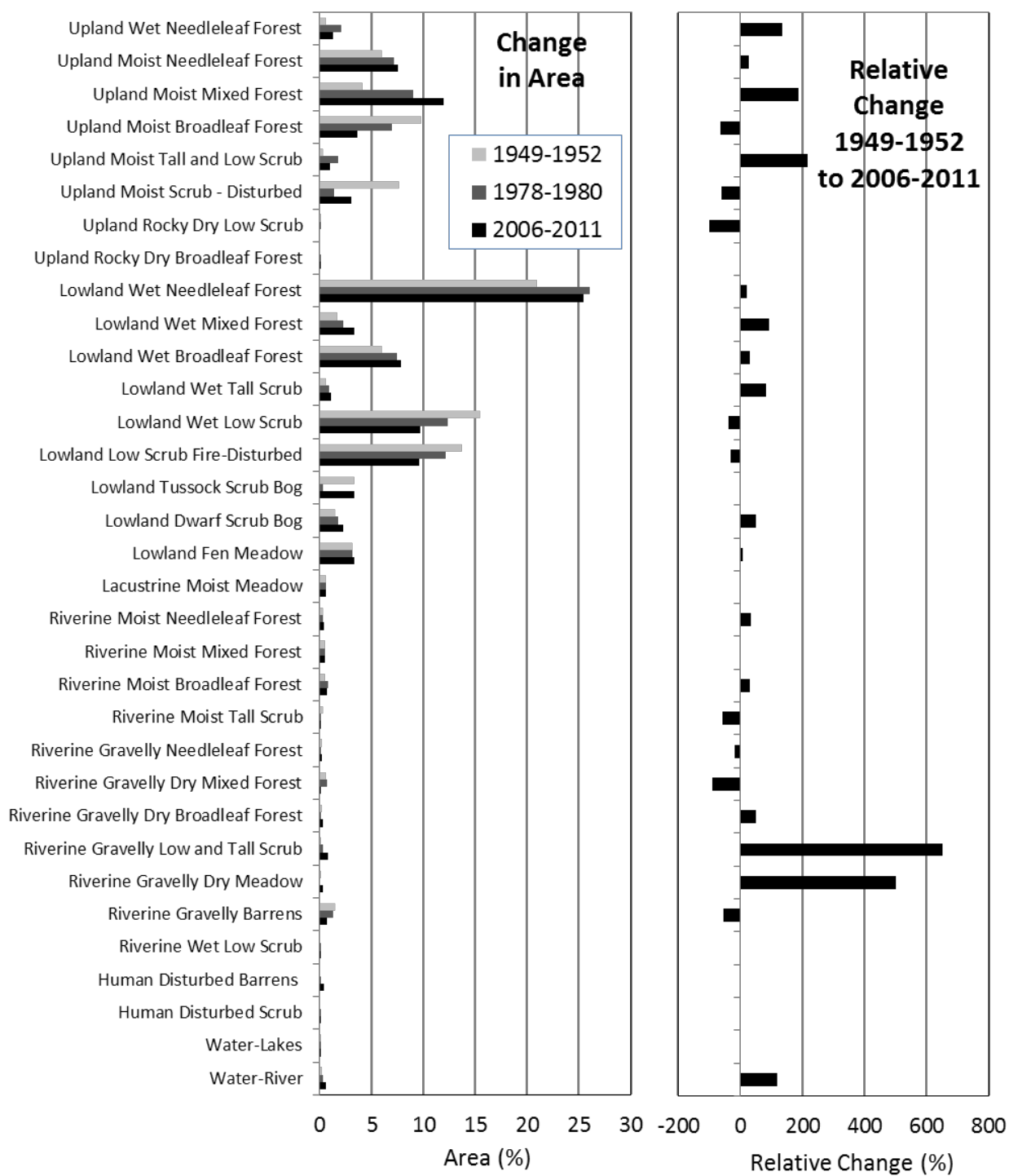
Figure 58. Changes in area (%) of ecotypes from 1949–1952 to 2006–2011.
