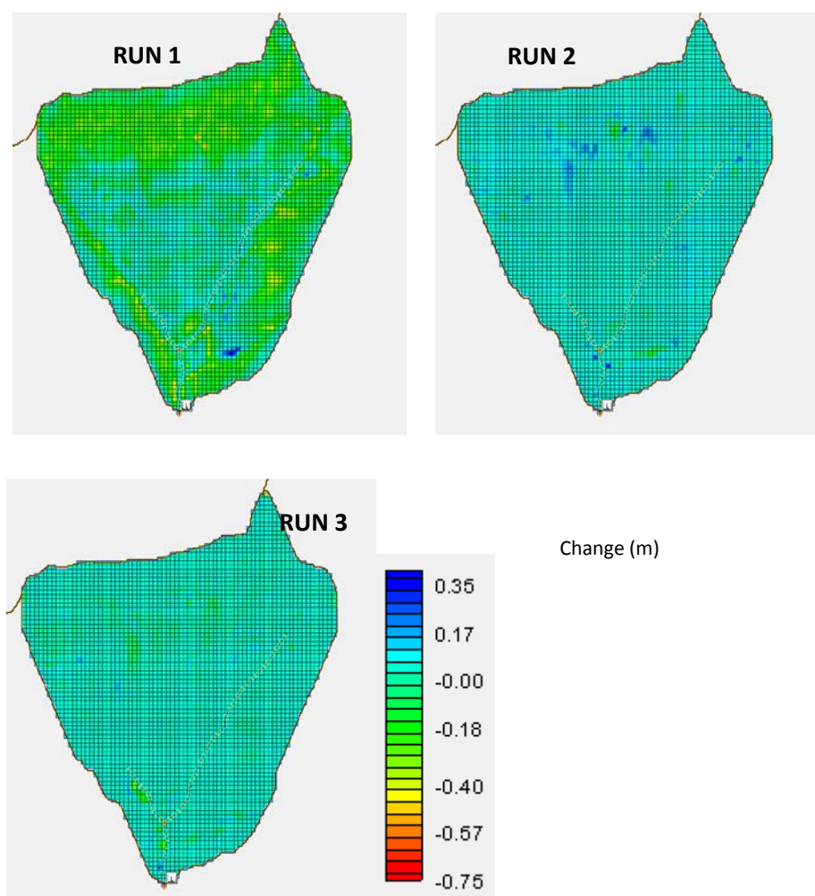
Figure 49. Changes in ground water table during each two-year initialization run.
