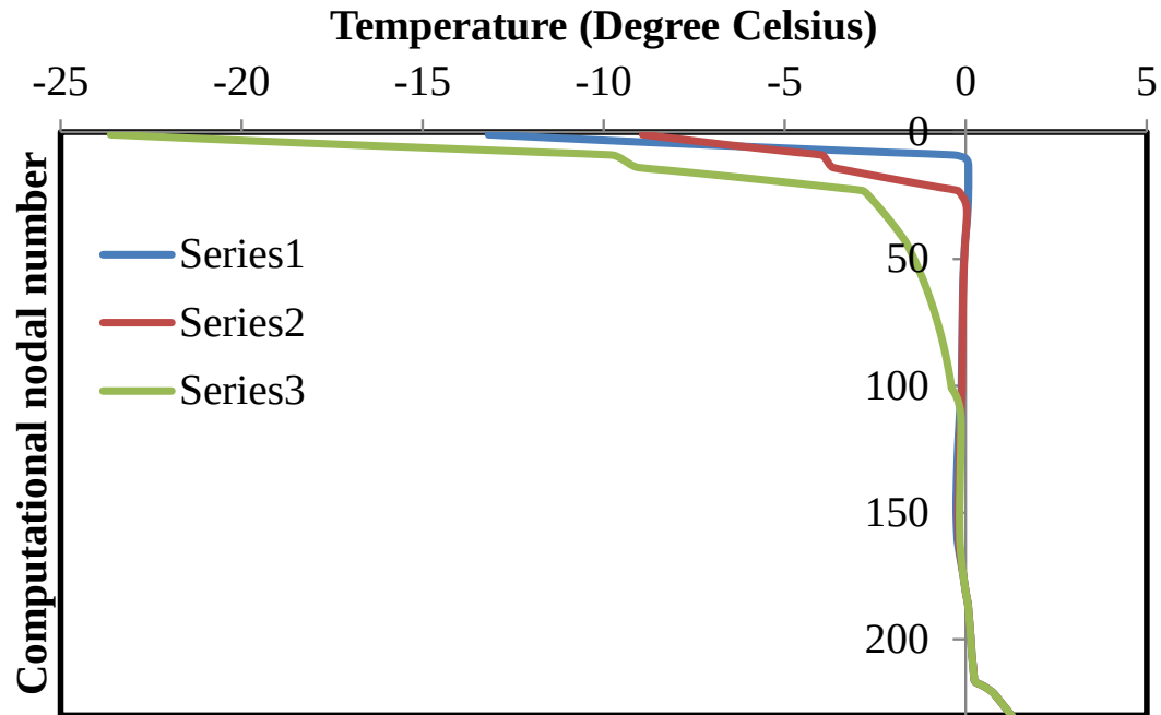
Figure 55. Soil temperature profiles.
