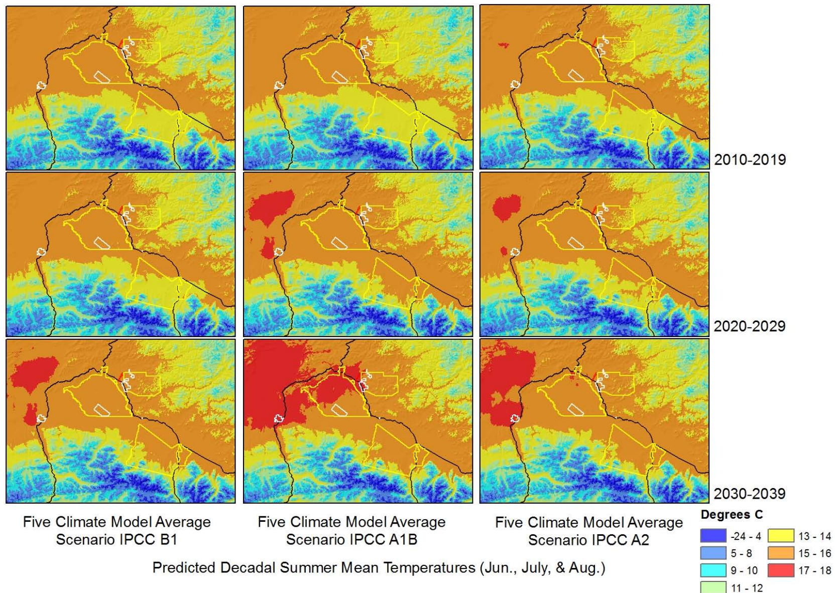
Figure 62. Downscaled projected decadal summer (June-August) mean temperatures for interior Alaska. U.S. Army Corps of Engineers project lands are outlined in red, Army lands are delineated by yellow, and Air Force lands are marked by white.
