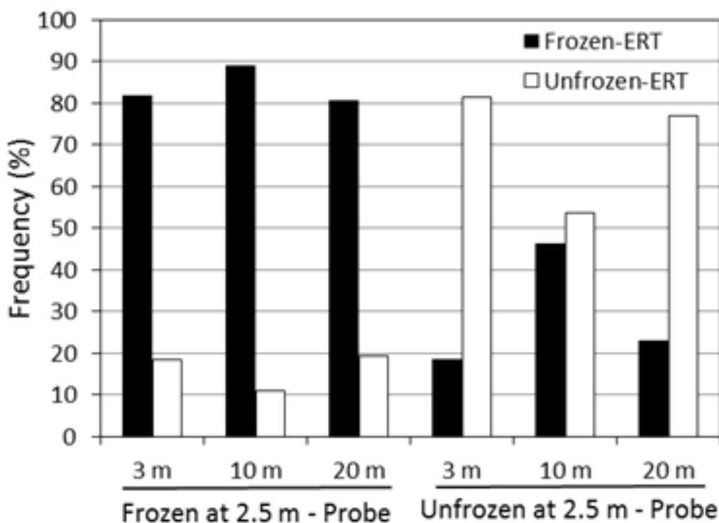
Figure 40. Correlation between permafrost status determined by thaw probing and by ERT across the 1930, 1988, 2001, and 2010 fire scar transects. The frequencies are grouped for locations where soil was frozen or unfrozen at 2.5 m by probing, with frequencies of frozen and unfrozen ground at 3, 10, and 20 m depths as determined by ERT (unfrozen when \Omega -m < 600, frozen when \Omega -m > 600).
