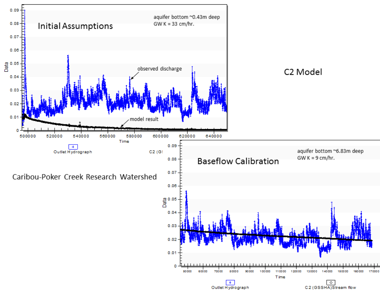
Figure 50. Example baseflow calibration results from the C2 sub basin.
