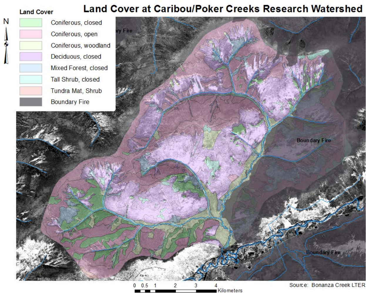
Figure 47. Land cover map of the Caribou/Poker Creek Research Watershed including extents of the 2004 Boundary Fire. Open and closed designations refer to canopy density. An open canopy permits a view of the sky through it.
