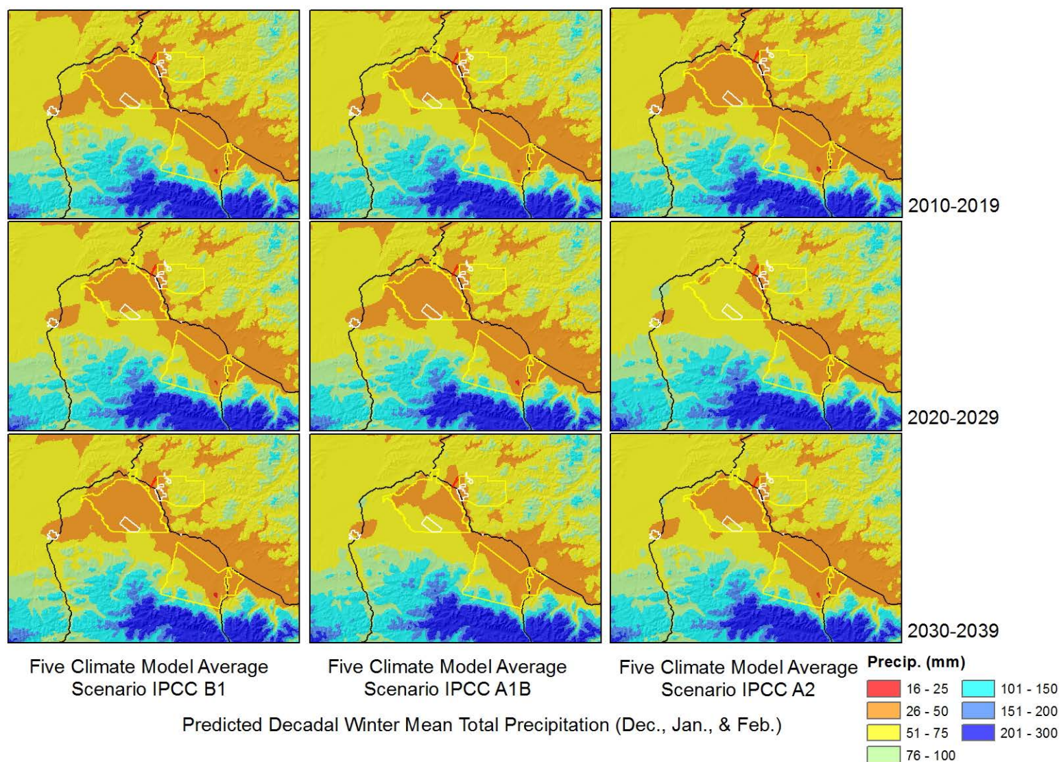
Figure 68. Downscaled projected decadal winter (December-February) average total precipitation for interior Alaska. U.S. Army Corps of Engineers project lands are outlined in red, Army lands are delineated by yellow, and Air Force lands are marked by white.
