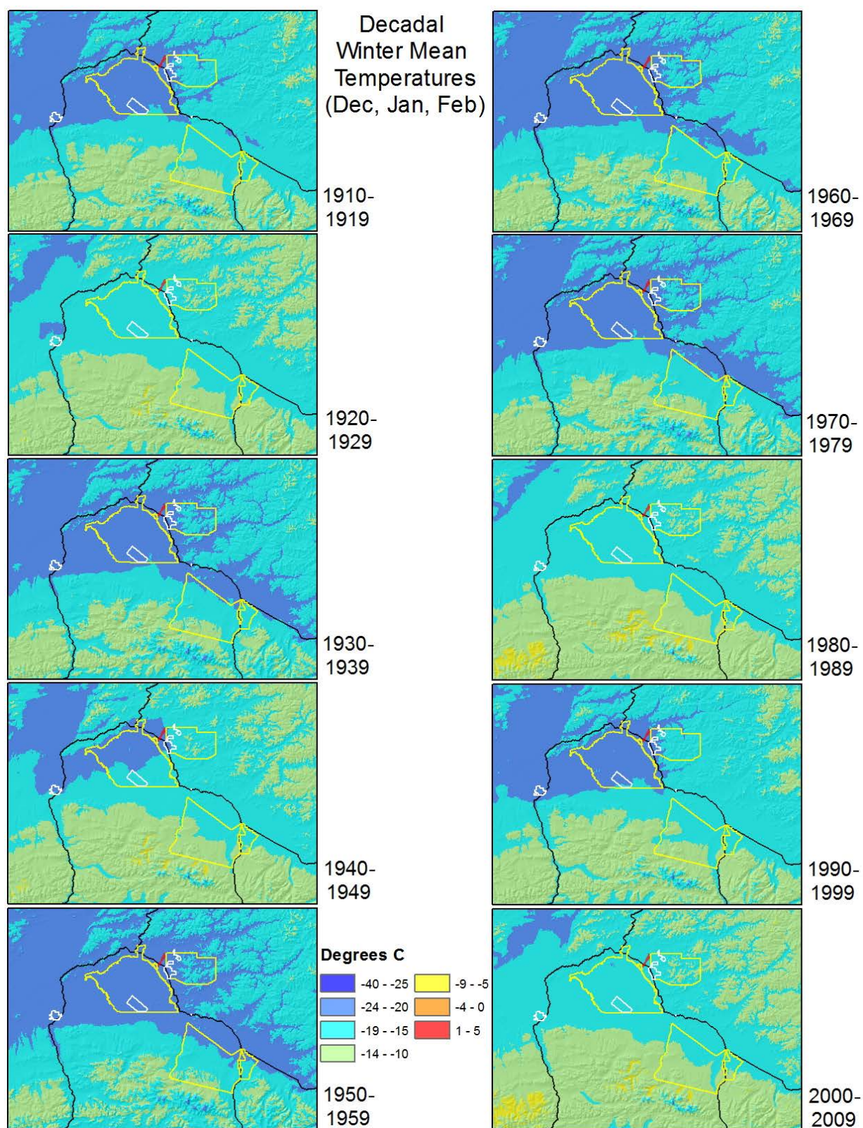
Figure 65. Decadal winter (December-February) mean temperatures show variability from one decade to another. U.S. Army Corps of Engineers project lands are outlined in red, Army lands are delineated by yellow, and Air Force lands are marked by white.
