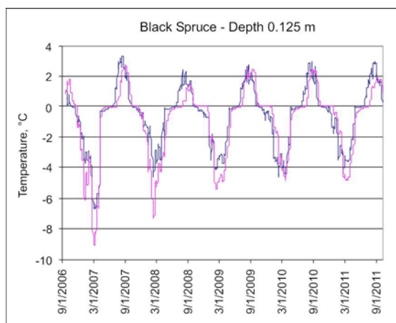
Figure 44. Landscape settings (A, B) and examples of the temporal calibration of the GIPL model (C, D, E, F) for one specific site in a black spruce forest interior Alaska. In D, E, and F the blue and pink lines represent measurements from two locations at the site.
