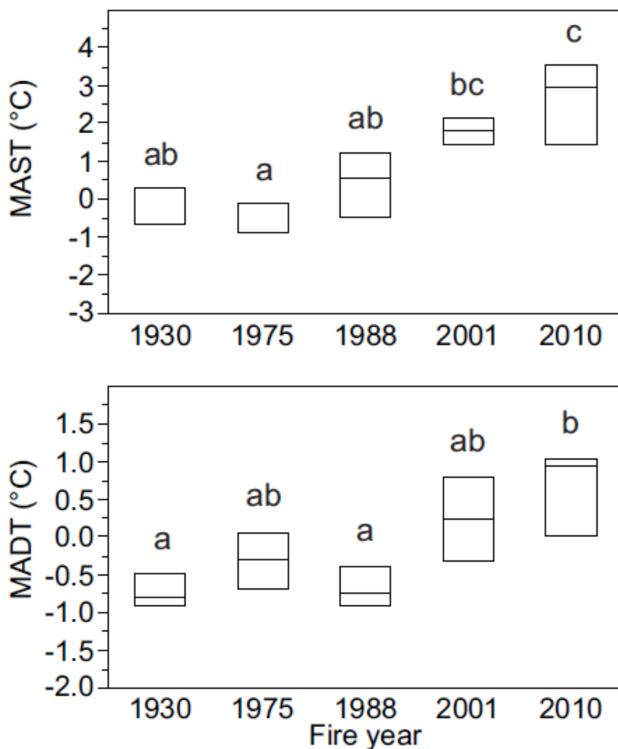
Figure 24. Box plots of MAST and MADT by fire year. Data are from hydrological year 2013 ( n = 14 ). Tukey-Kramer HSD post hoc tests were conducted following one-way ANOVAs. Factors not connected by the same letter are significantly different ( p < 0.05 ).
