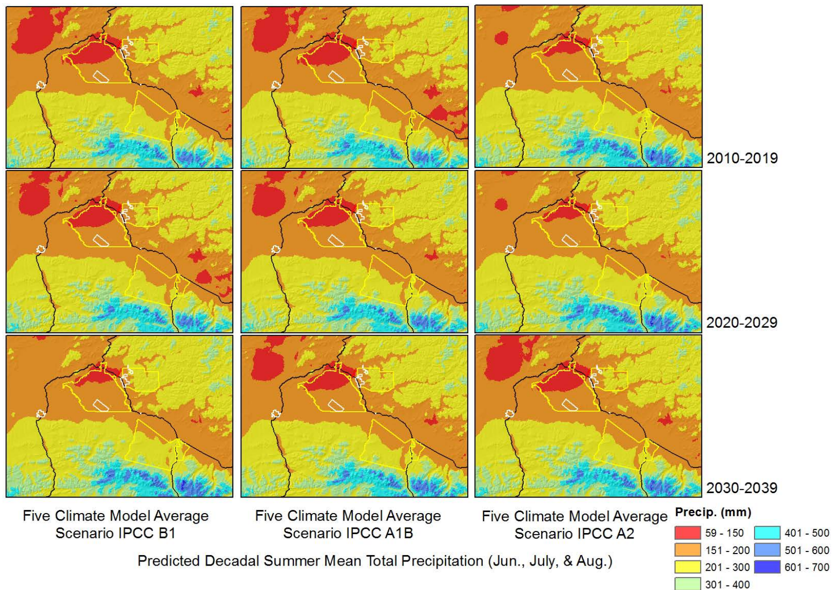
Figure 64. Downscaled projected decadal summer (June-August) average total precipitation for interior Alaska. U.S. Army Corps of Engineers project lands are outlined in red, Army lands are delineated by yellow, and Air Force lands are marked by white.
