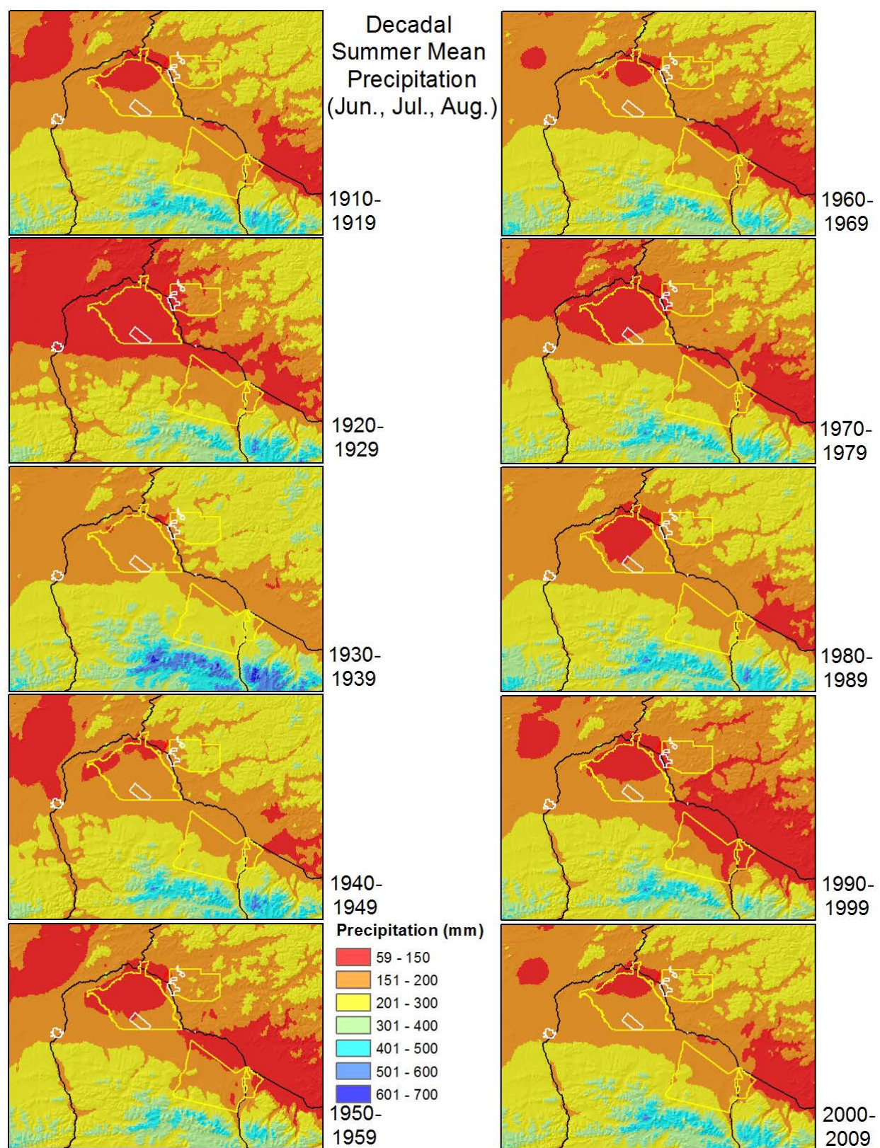
Figure 63. Decadal summer (June-August) total precipitation shows a general increase decrease from one decade to another for interior Alaska. U.S. Army Corps of Engineers project lands are outlined in red, Army lands are delineated by yellow, and Air Force lands are marked by white.
