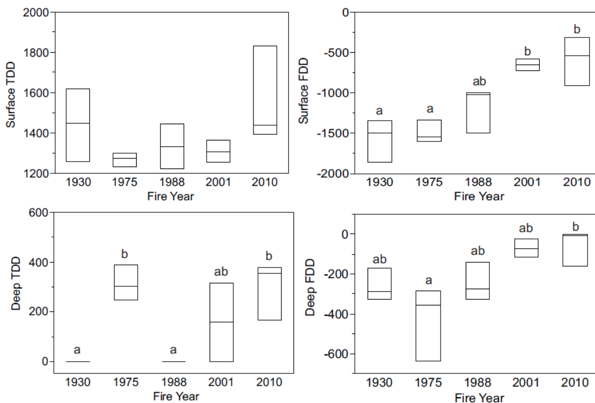
Figure 25. Box plots of surface and deep TDD and FDD by fire year. Data are from hydrological year 2013 ( n = 14 ). Tukey-Kramer HSD post hoc tests were conducted following one-way ANOVAs. Significant differences ( p < 0.05 ) are denoted by different letters.
