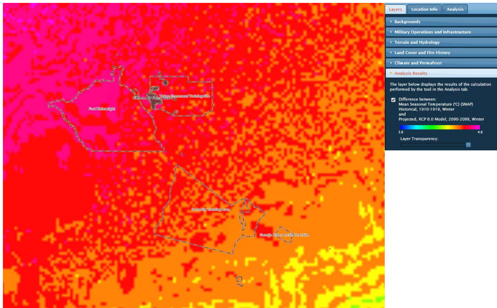
Figure 71. A comparison between mean winter season temperatures from the historical dataset (1910-1919) compared to projected 2090-2099 values using RCP scenario 6.0. The difference values plotted here are the degrees of warming for the interior Alaska training range domain
