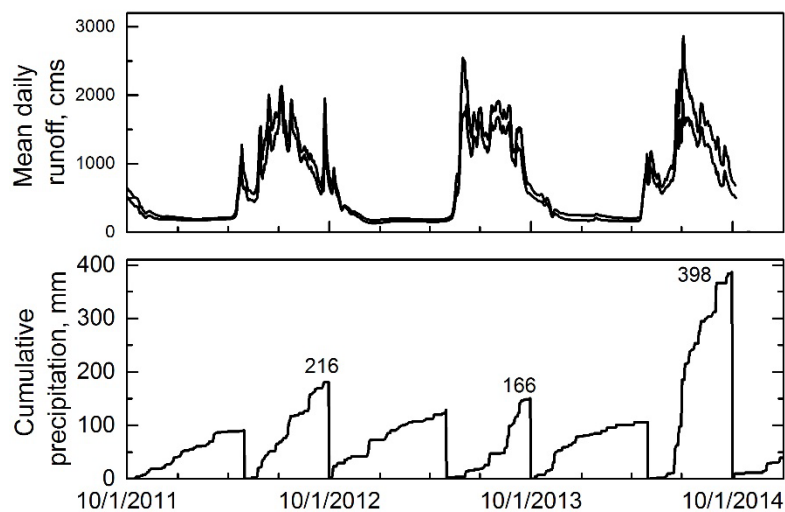
Figure 18. Mean daily runoff of the Tanana River near Fairbanks (top) and cumulative precipitation separated into winter (Oct-Apr) and summer (May-Sep) from Fairbanks International Airport. Noted are the total summer precipitation values in 2012, 2013 and 2014.
