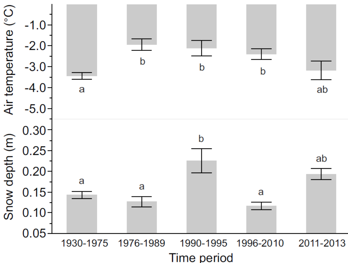
Figure 28. Mean annual air temperature and snow depth by time period. Time periods were chosen to represent dominant patterns in simulated permafrost dynamics. Values are means \pm SE and significant differences are depicted by lettering.
