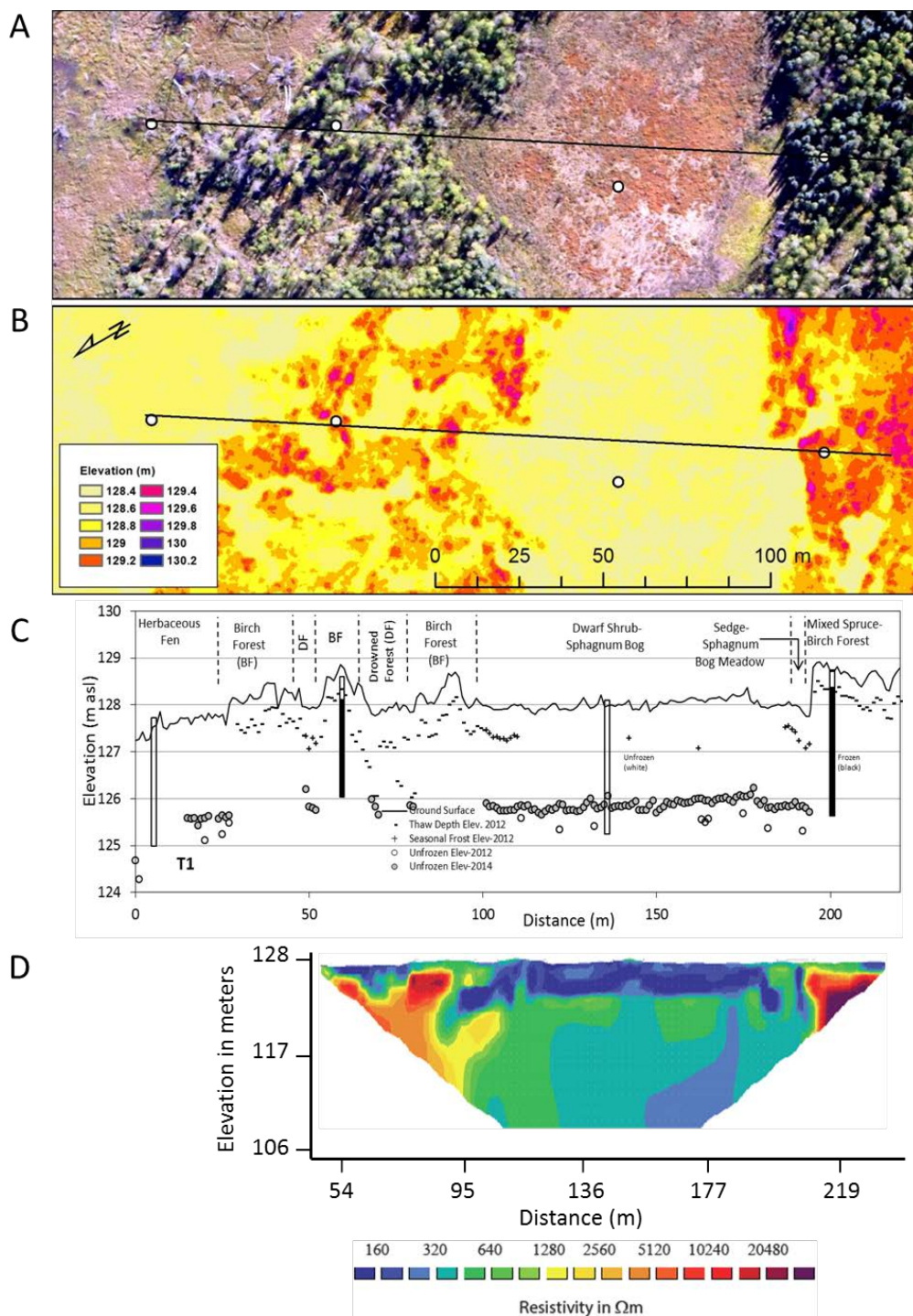
Figure 29. A: An aerial image of the 1930 fire scar. B: airborne LiDAR imagery, shaded by elevation, for the same region presented in the upper panel. The bold line indicates the location and length of the transect at the site while circles denote locations where SIPRE cores were collected. C: A detailed cross section of the vegetation, ground elevation, SIPRE core depths, seasonal thaw depths, and elevations of unfrozen material across the transect. D: electrical resistivity tomography survey results across the transect.
