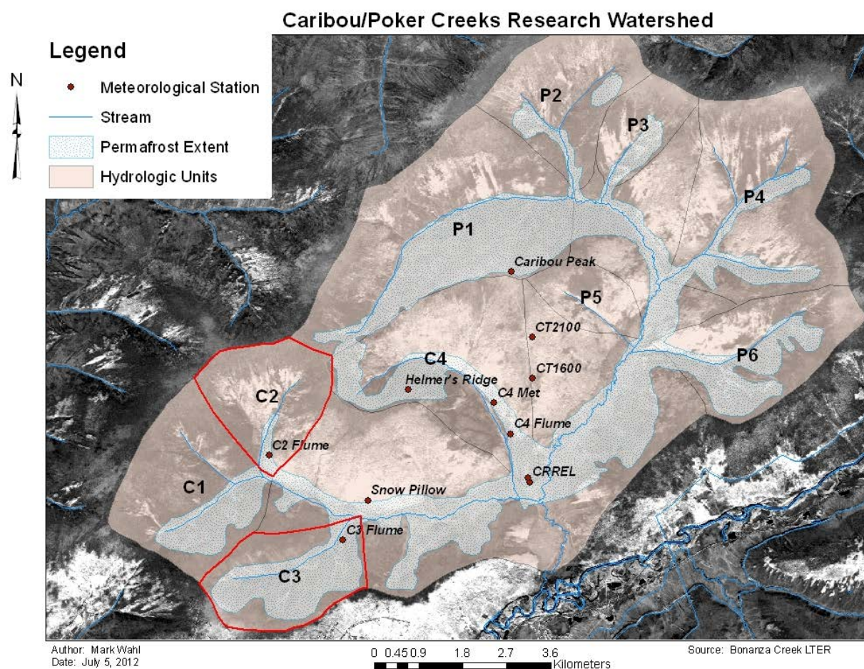
Figure 46. Hydrologic units of the Caribou/Poker Creeks Research Watershed (CPCRW) with locations of hydrometeorological stations and permafrost extents indicated (Chapin and Hollingsworth 2010a; b). Models of the C2 and C3 sub-watersheds compare the hydrologic effects from disparate expanses of permafrost.
