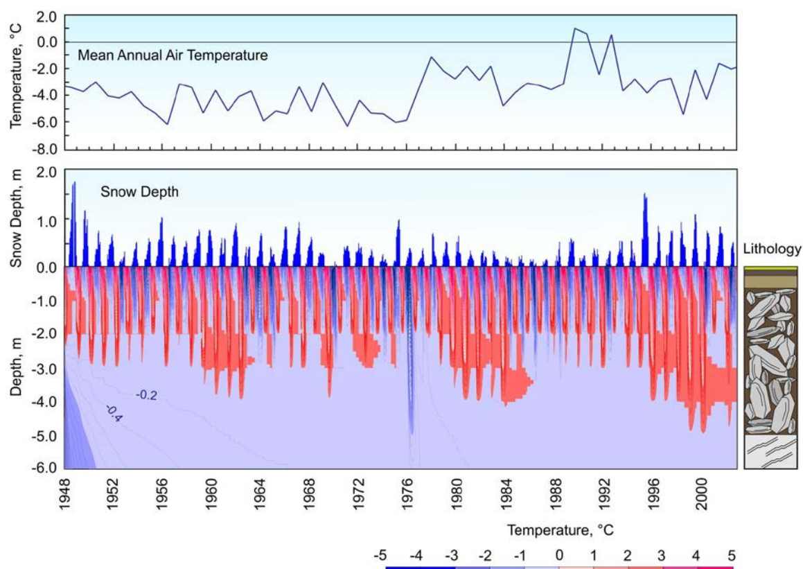
Figure 45. A reconstruction of ground thermal properties (permafrost evolution) from 1948 to 2005 at a shrubland site.
