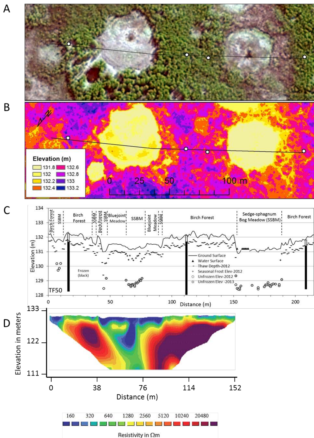
Figure 31. A: An aerial image of the 1988 fire scar. B: airborne LiDAR imagery, shaded by elevation, for the same region presented in the upper panel. The bold line indicates the location and length of the transect at the site while circles denote locations where SIPRE cores were collected. C: A detailed cross section of the vegetation, ground elevation, SIPRE core depths, seasonal thaw depths, and elevations of unfrozen material across the transect. D: electrical resistivity tomography survey results across the transect.
