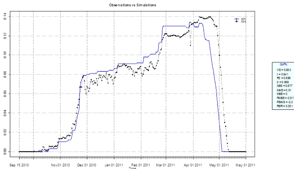
Figure 52. Simulated snow pack (blue line) at CPCRW compared with observed (black line) snow accumulation and snowmelt from 2011. The y-axis is snow water equivalent in centimeters.
