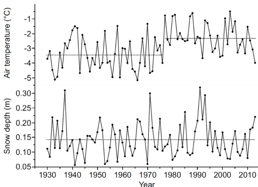
Figure 12. Mean annual air temperatures and snow depths at the Fairbanks International Airport, computed by hydrological year (October 1 – September 30) from 1930-2013 (Alaska Climate Research Center, 2014). Dotted lines indicate mean values over the specified time period.
