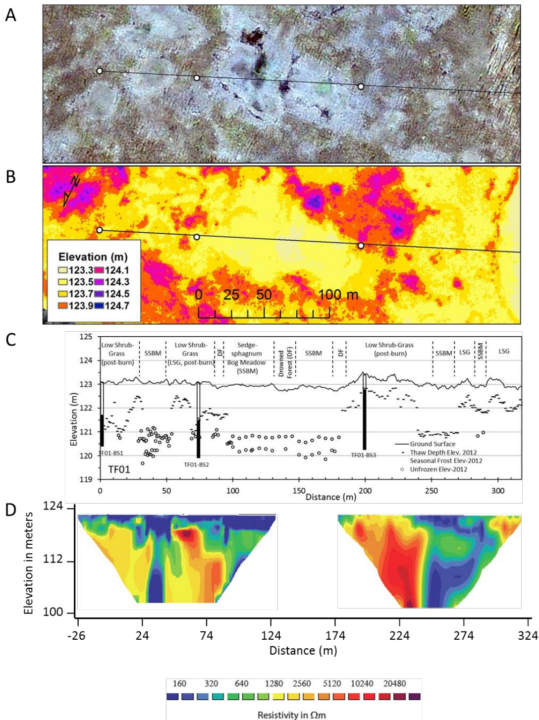
Figure 32. A: An aerial image of the 2001 fire scar. B: airborne LiDAR imagery, shaded by elevation, for the same region presented in the upper panel. The bold line indicates the location and length of the transect at the site while circles denote locations where SIPRE cores were collected. C: A detailed cross section of the vegetation, ground elevation, SIPRE core depths, seasonal thaw depths, and elevations of unfrozen material across the transect. D: electrical resistivity tomography survey results across the transect.
