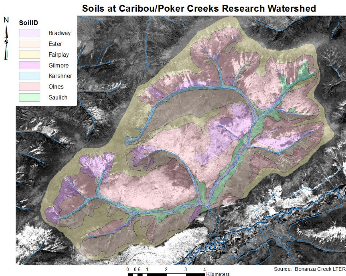
Figure 48. A soil map based on Reiger (1972) at the Caribou/Poker Creek Research Watershed.
