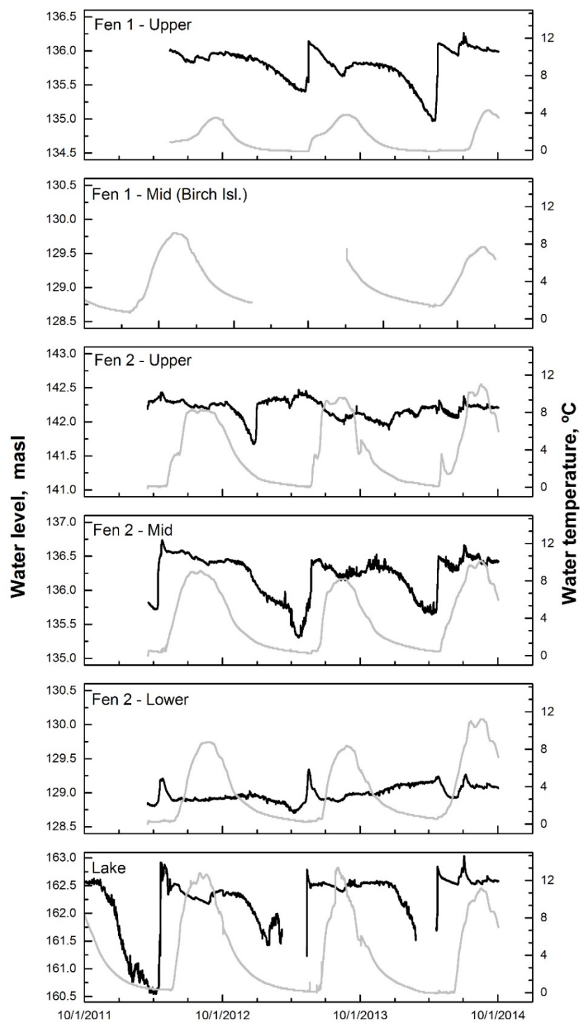
Figure 17. Measured (hourly) water levels (black) and water temperature (gray) in two parallel fens (Fen 1 and Fen 2) and at a groundwater-fed lake ~15 km south of the two fens. Each of the two fens had a sensor located at the head of the fen (upper) and further downstream. Apart from the bottom Lake graph, the y-axis represents an elevation range of 2 m.
