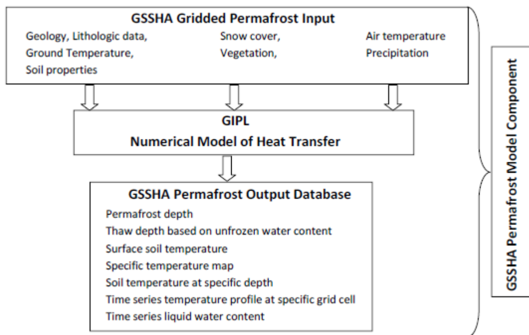
Figure 54. GIPL as a permafrost component in GSSHA.
