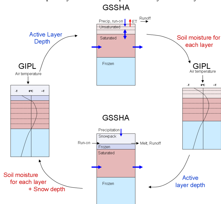
Figure 14. A flow chart identifying the interactions between major components in the coupled GSSHA and GIPL model.
