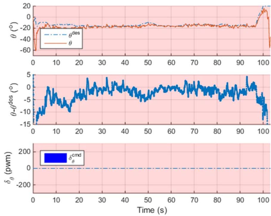
Figure 55. Sparrow Final Flight: Pitch, Desired Pitch and PWM Time Histories
