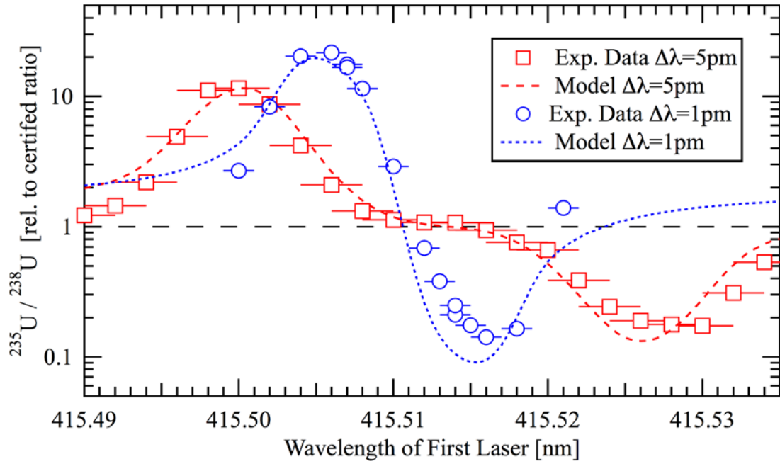
Figure 7. Measured and Predicted ^{235}\text{U}/^{238}\text{U} Ratio. Source: [6].
