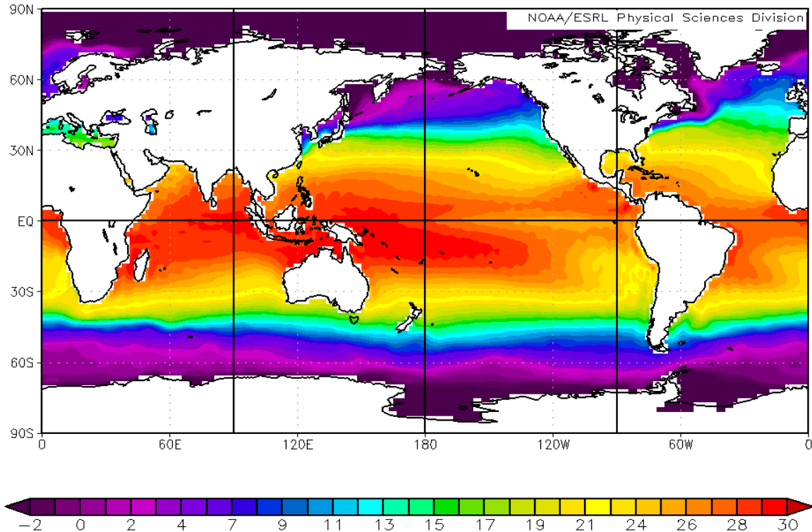
Figure 8. LTM Sea Surface Temperature (SST; °C) for JFM.
