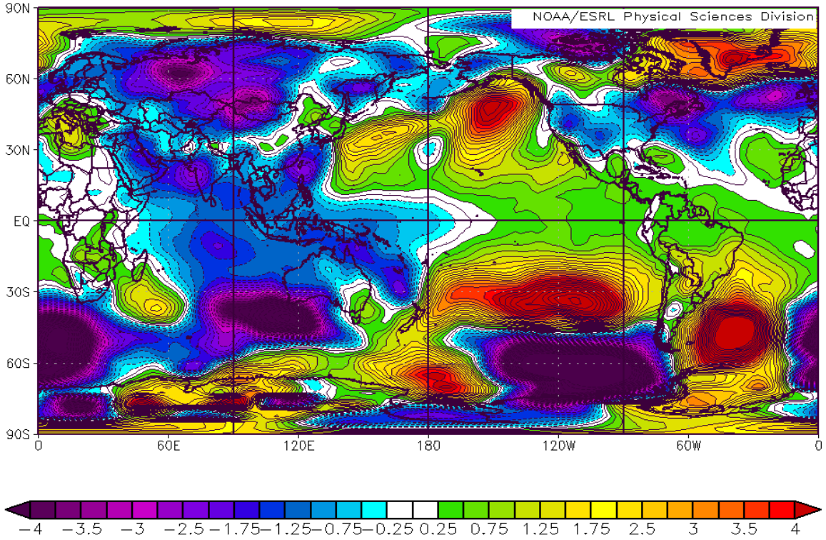
Figure 99. SLP Anomalies (mb) for MJO Phase 4 and LN Years during JAS.
