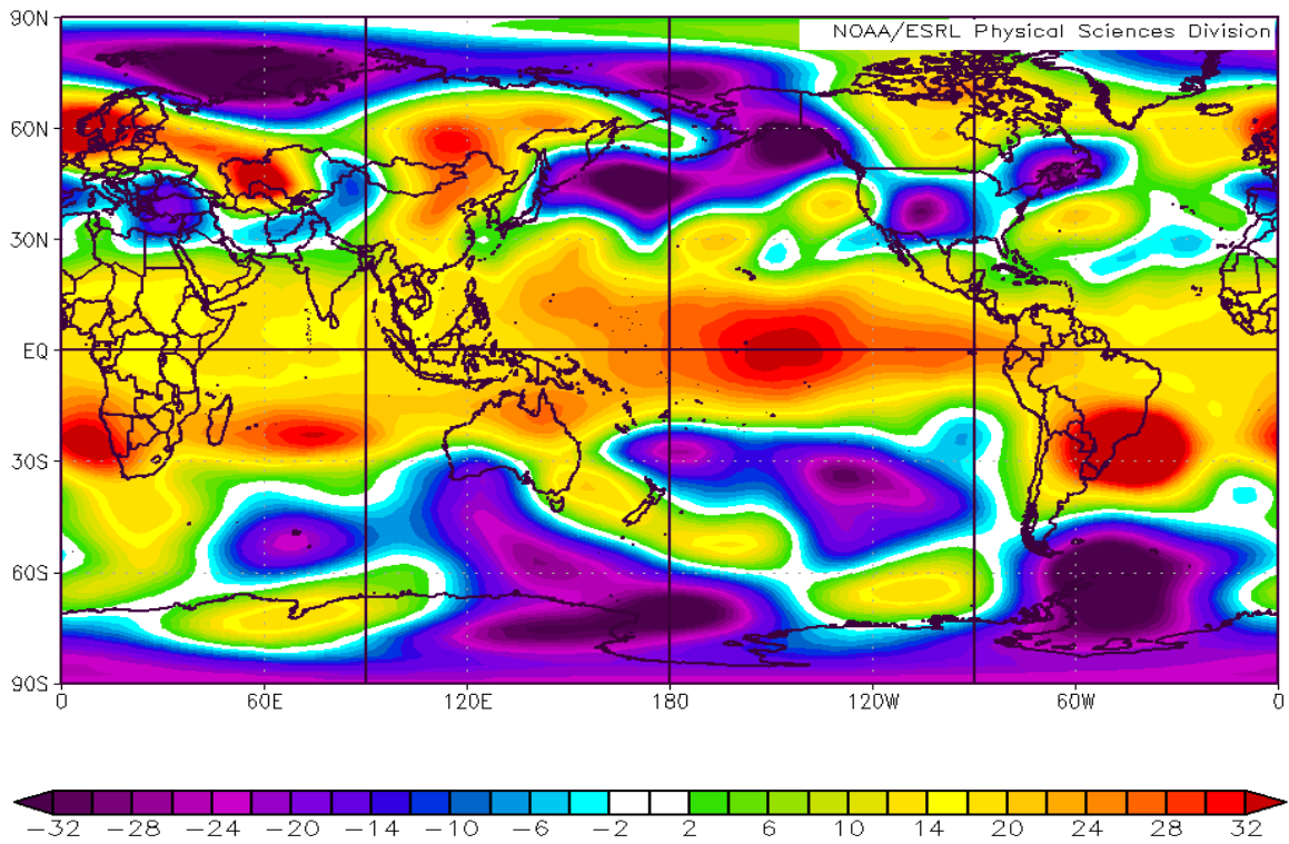
Figure 95. Z200 Anomalies (mb) for MJO Phase 4 and EN Years during JAS.
