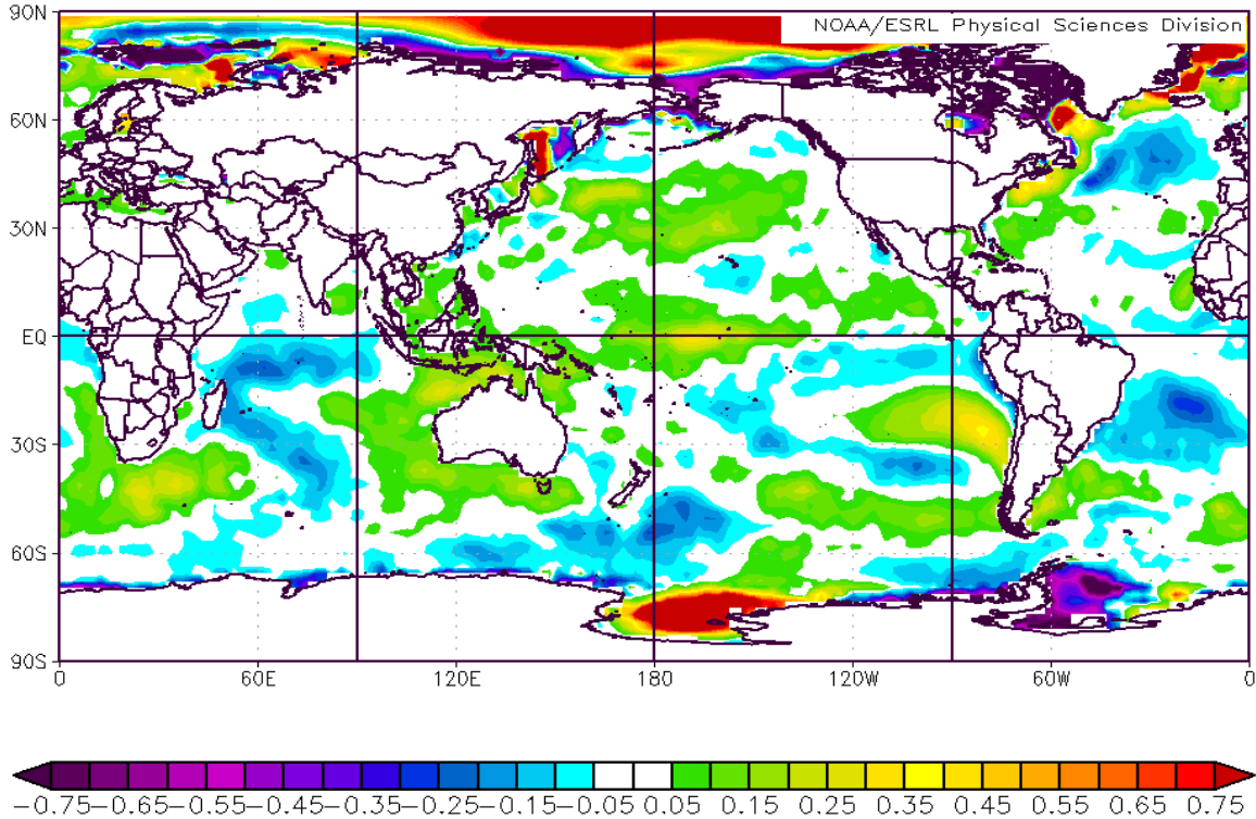
Figure 28. SST Anomalies ( ^{\circ}\text{C} ) for MJO Phase 4 and all EN, LN, and Neutral Years during JFM.
