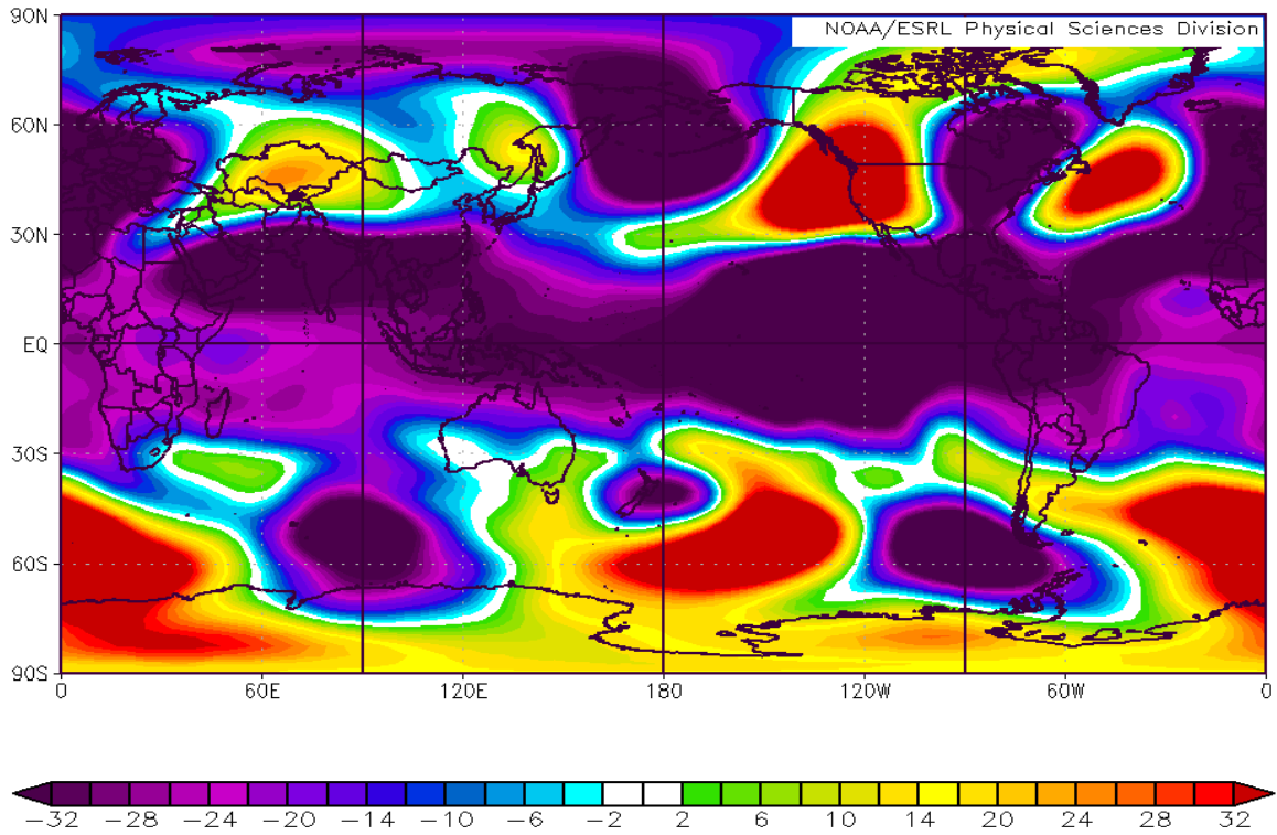
Figure 60. Z200 Anomalies (mb) for MJO Phase 8 and LN Years during JFM.
