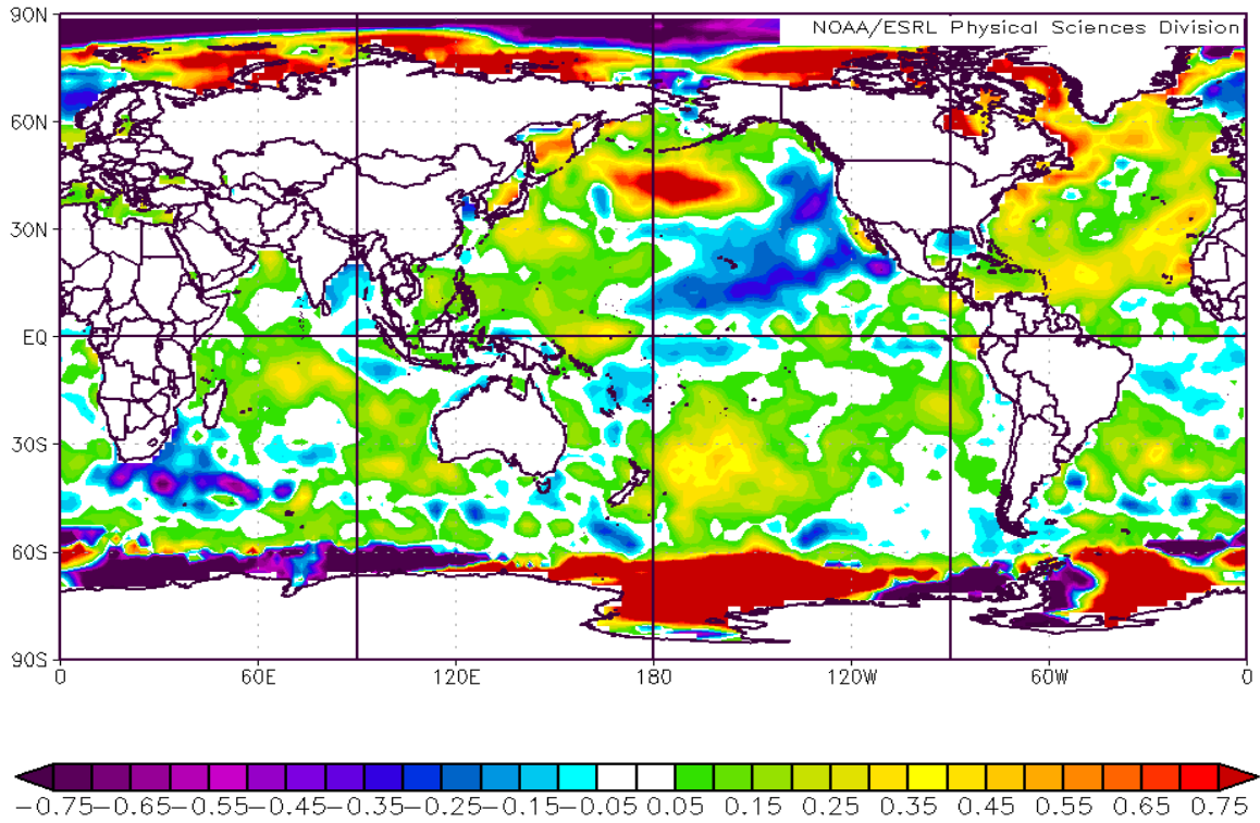
Figure 103. SST Anomalies (°C) for MJO Phase 4 and Neutral Years during JAS.
