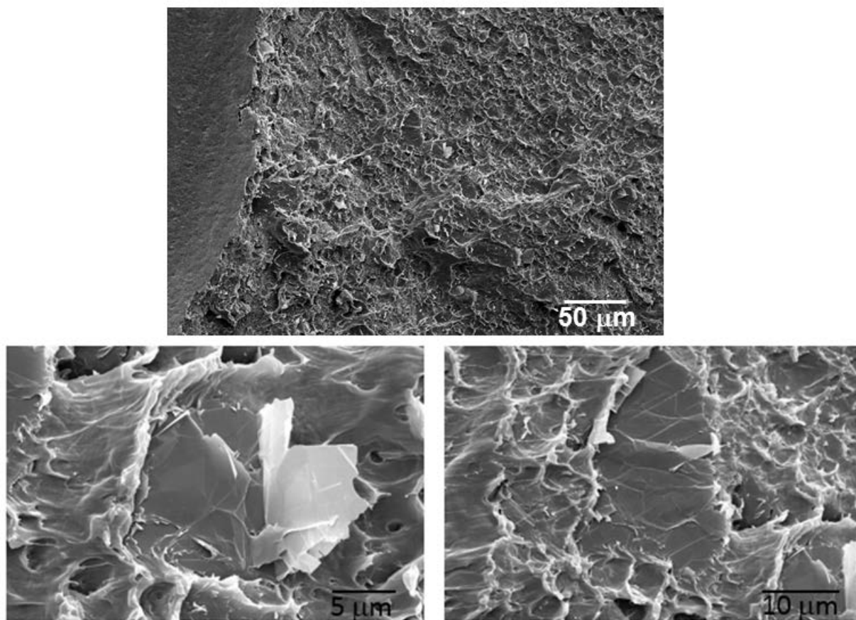
Figure 8. SEM images of the cohesive failure region with clearly visible graphene nanoplatelets.
