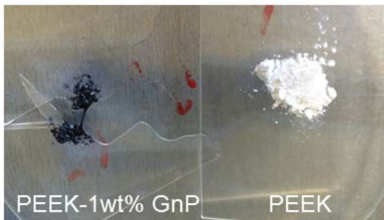
Figure 5. 1wt% GnP-PEEK and Pure PEEK powder (white) exposed to microwaves. The GnP composite absorbs the radiation and melts, while the pure PEEK powder does not melt due to low absorption.
