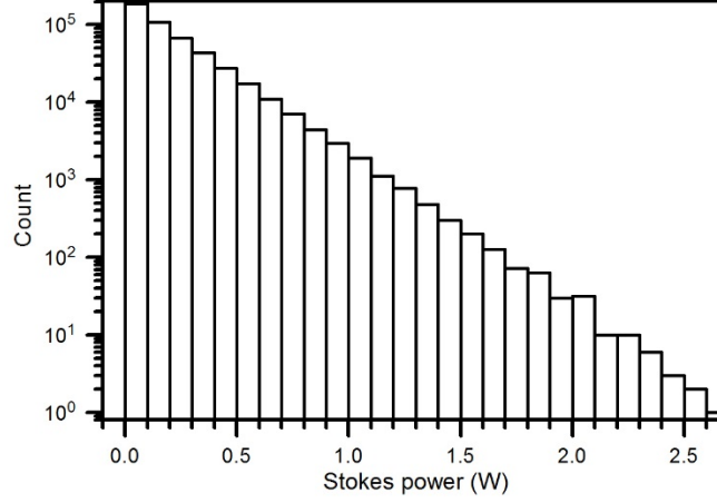
Fig. 11 Histogram of P_S(z = 0, t) sampled at the grid spacing of 2 ps for 8 transits. The average power is 0.2 W.
