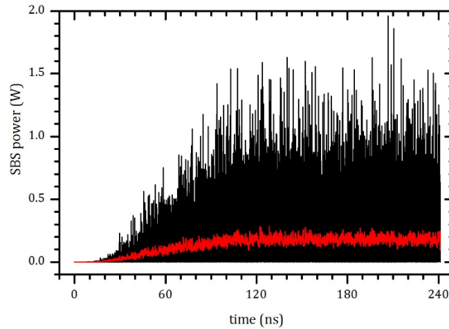
Fig. 10 SBS power at z = 0 vs. time, for 2 transits, and a sliding average taken over 0.24 ns
