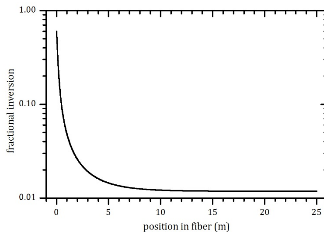
Fig. 5 Fractional inversion vs. position in the fiber at t = 0 , at a pump power of 1.8 kW
