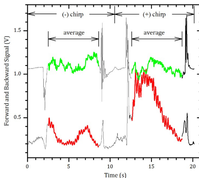
Fig. 2 Oscilloscope traces representing the output power (upper trace) and backward power (lower trace), taken at an output power of 1.6 kW. The data points in Fig. 3 are averages of the bold portions of the traces.
