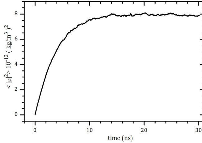
Fig. 9 Magnitude squared density fluctuations averaged over z vs. time for one quarter of a transit
