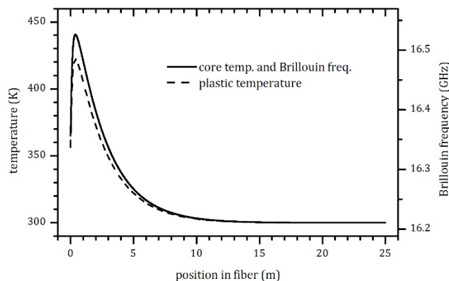
Fig. 6 Simulated conditions inside the fiber at a pump power of 1.8 kW. Temperature at the center of the core (upper curve) and the cladding/coating interface (lower curve). The Brillouin frequency is shown by the solid curve referred to the right hand axis.
