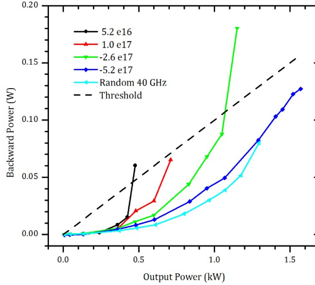
Fig. 3 Backward power vs. output power for various chirps and for a seed with a bandwidth of 40 GHz produced by random phase modulation. The dashed line represents a ratio of 10^{-4} .
