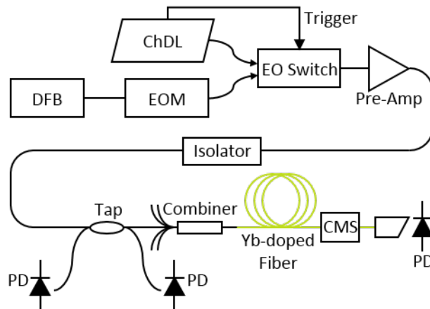
Fig. 1 Experimental setup with chirped diode laser (ChDL), distributed feedback Bragg (DFB) laser, electro-optic modulator (EOM), photodiodes (PDs), cladding mode stripper (CMS), and end cap
