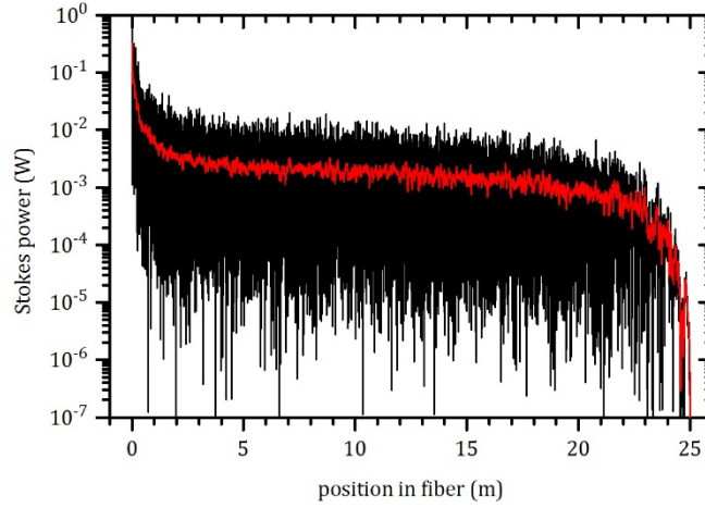
Fig. 7 Stokes power vs. position in the fiber vs. z , after the last transit, and a sliding average taken over 5 cm
