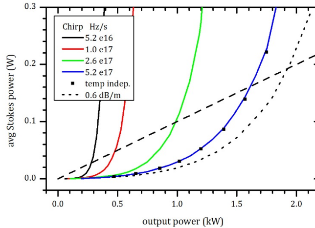
Fig. 12 Average Stokes power vs. output laser power calculated for various chirps. The solid lines are calculated with the full temperature dependence. The symbols are calculated as though the entire fiber were at 300 K. The dotted line is calculated at the fastest chirp with a lower pump attenuation of 0.6 dB/m. The dashed line indicates the SBS threshold.
