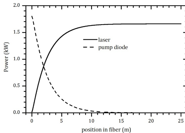
Fig. 4 Pump and laser powers vs. position in the fiber at t = 0
