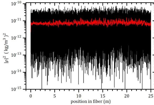
Fig. 8 Magnitude squared density fluctuation vs. z , after the last transit, and a sliding average taken over 5 cm
