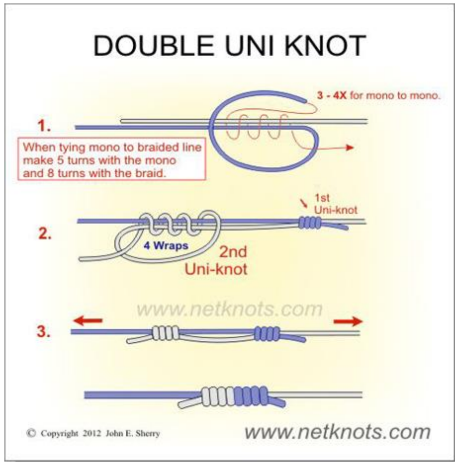
Figure 2: Double Uni Knot http://www.netknots.com/fishing_knots/double-uni-knot/
