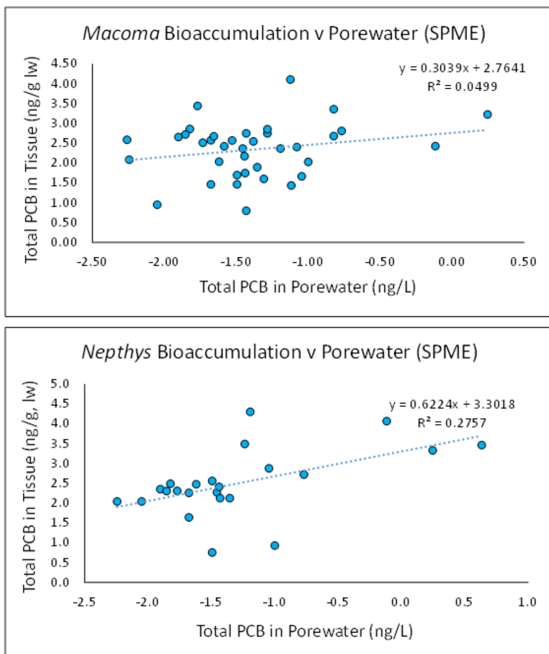
Figure 5-17. Comparison of total PCB concentrations in Macoma (top) and Nephtys (bottom) with that of porewater concentrations derived from SPME. Concentrations are log transformed data from all four monitoring events.
