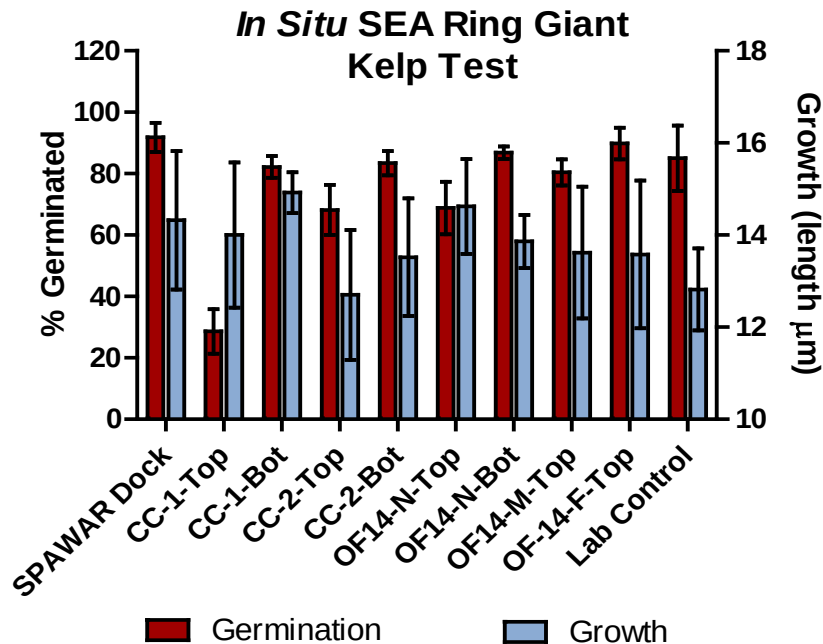
Figure 5-32. Results for in situ exposures for kelp ( Macrocystis pyrifera ) germination and growth (Mean values \pm 95% CI).
