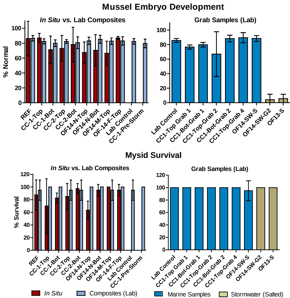
Figure 5-31. Individual species results for in situ and laboratory-based results for bivalve embryos and mysid shrimp, (Mean values \pm 95% CI).
