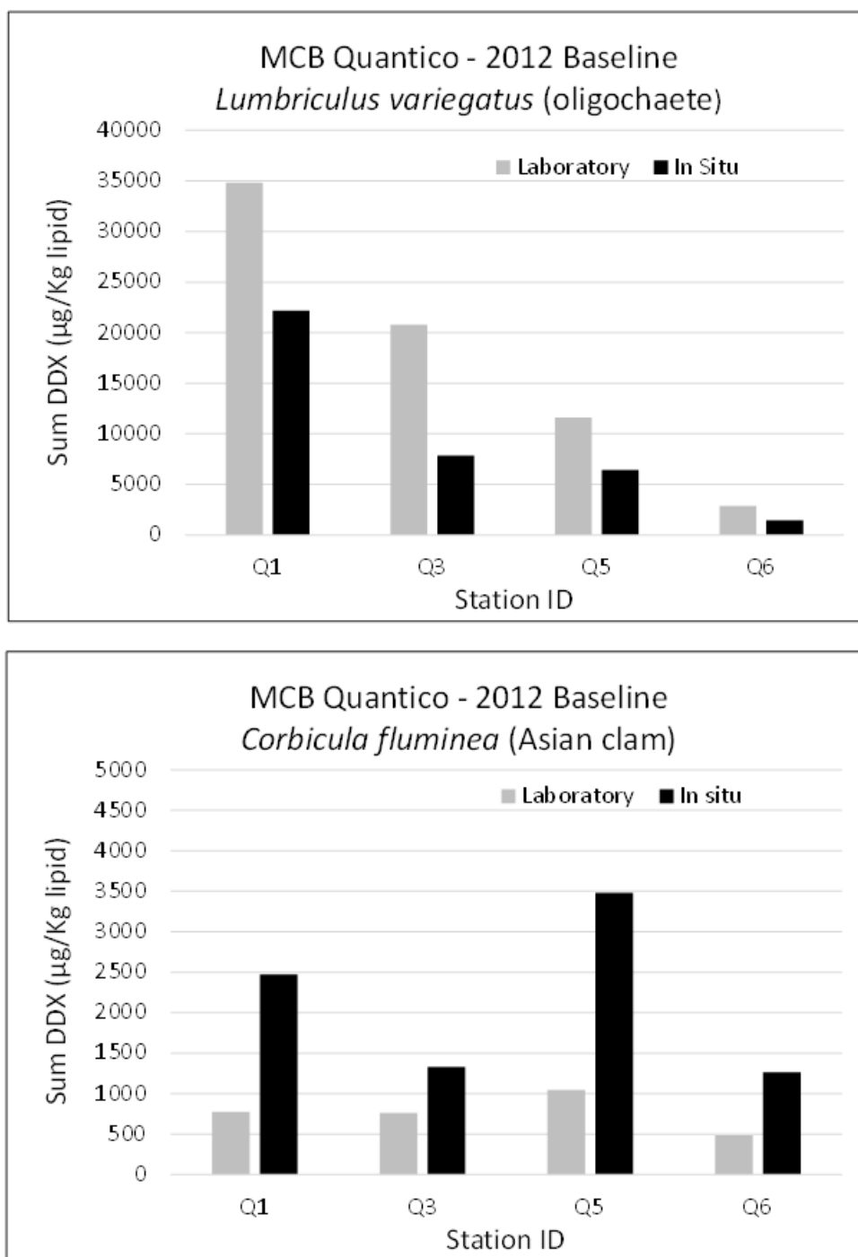
Figure 5-23. Comparison of 14-day bioaccumulation by Lumbriculus variegatus (top) and Corbicula fluminea (bottom) from laboratory and in situ exposures on composites of replicate sediment cores from MCB Quantico 2012 baseline event.
