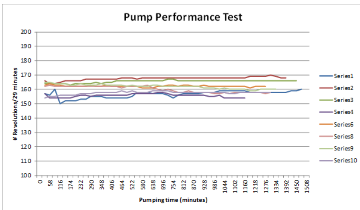
Figure B-2. Pump performance test results.
