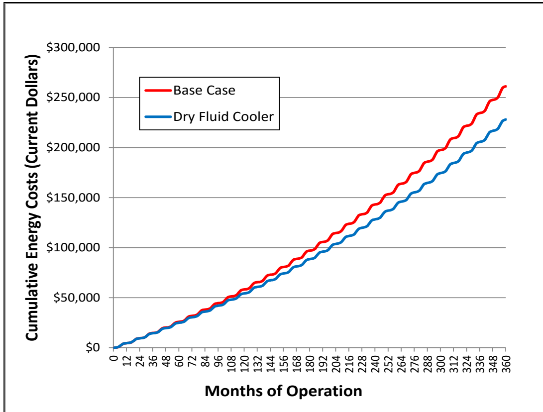
Figure 3.7. Cumulative electrical energy costs for the base case and the case with a dry fluid cooler.
