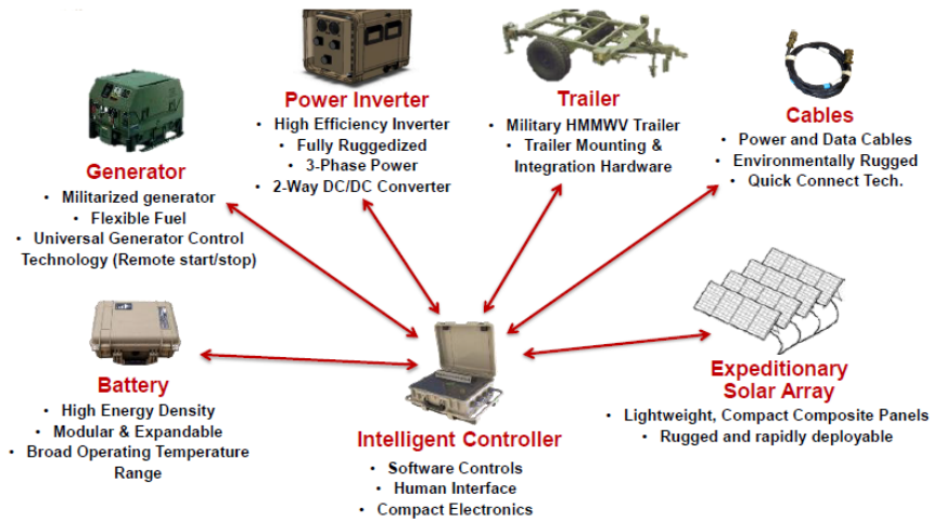
Figure 2.8. Intelligent Power Distribution System, Source [14].
