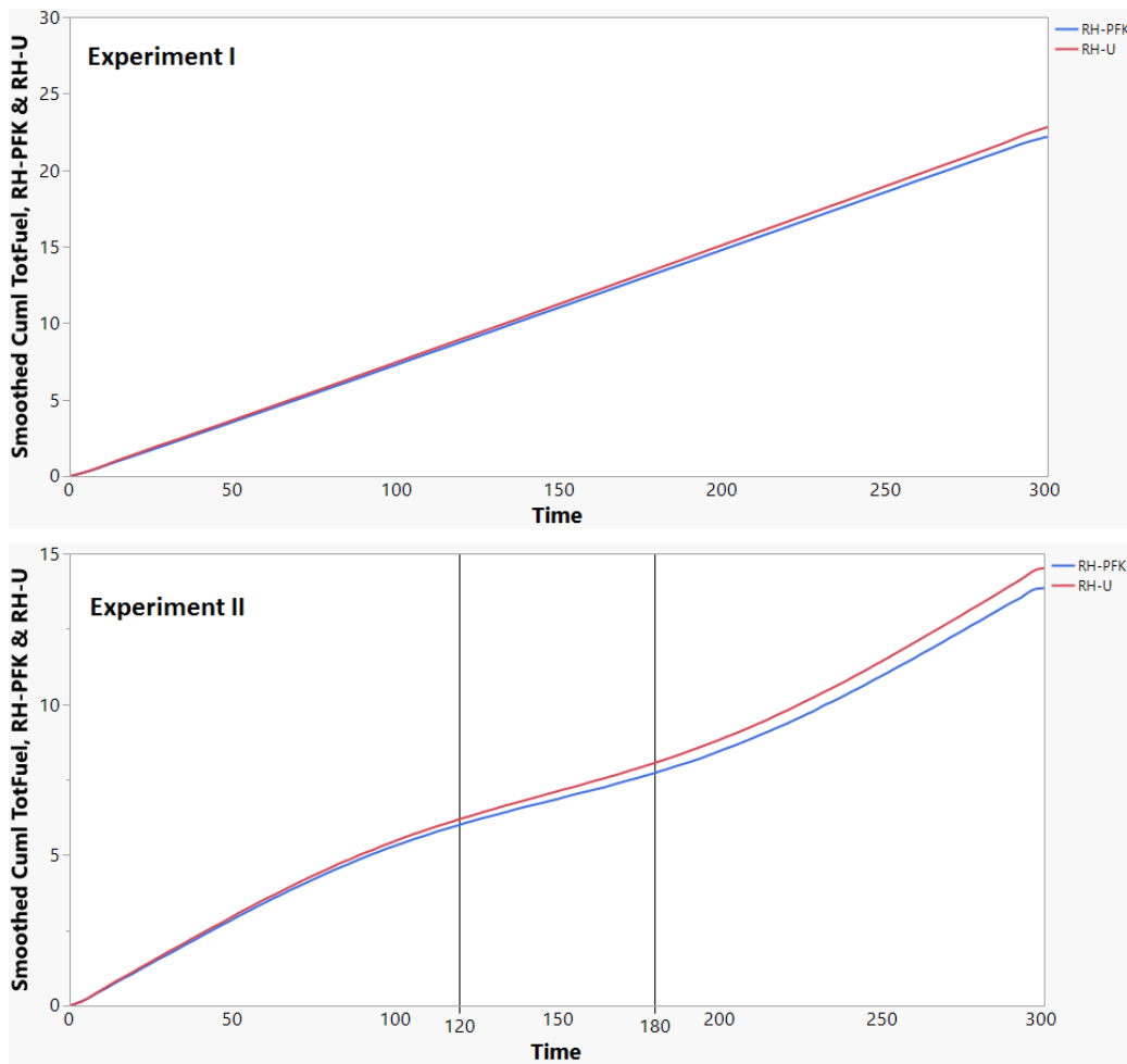
Figure 4.19. Cumulative Total Fuel Consumption, RH-PFK vs. RH-U
