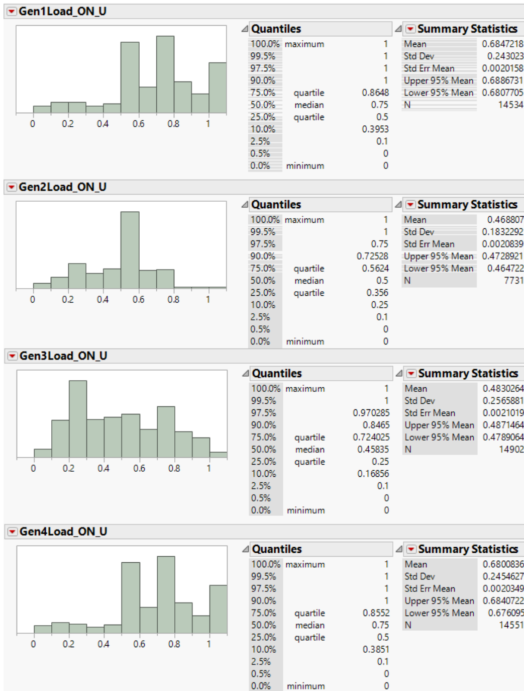
Figure 4.16. Experiment II Distribution of Generators' Load during Operation, RH-U.
