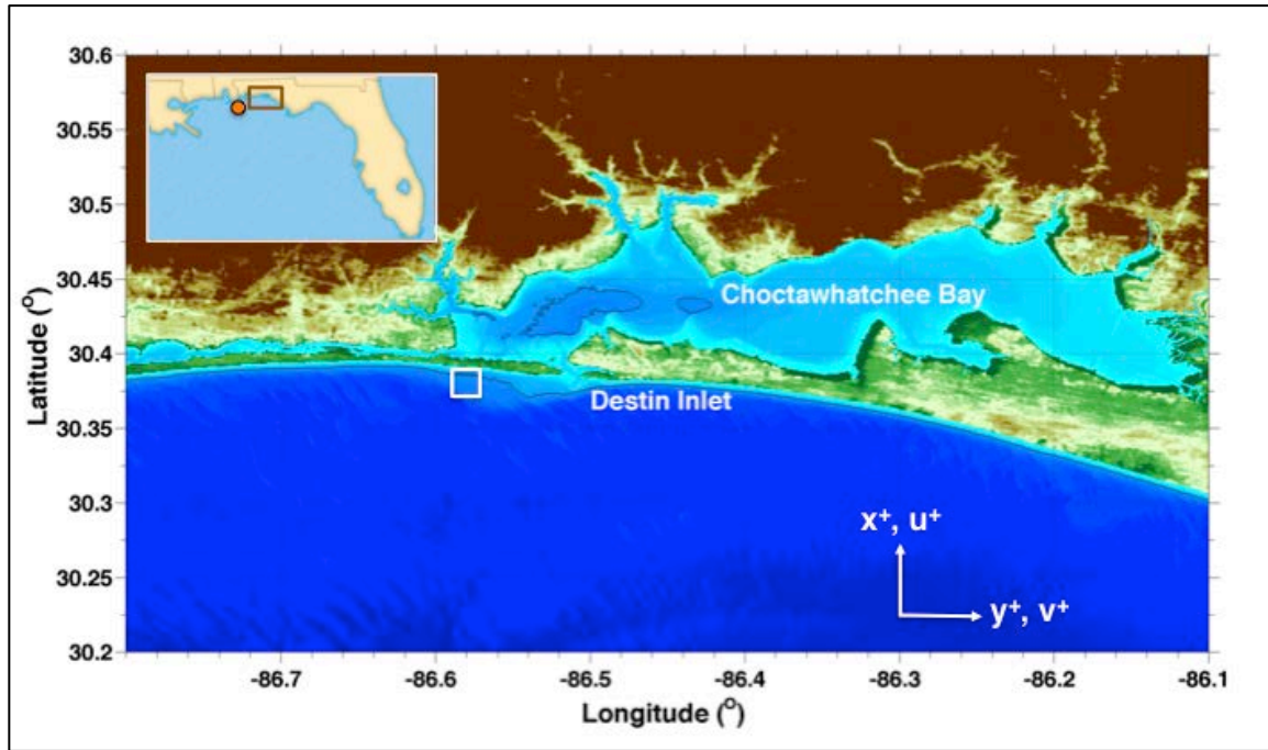
NOAA coastal digital elevation model of Choctawhatchee Bay and the adjacent inner shelf. White square indicates the location of the ADCP on the 10 m isobath. Inset shows the location of the experiment relative to the region. Orange circle represents the Orange Beach NOAA buoy and anemometer.
