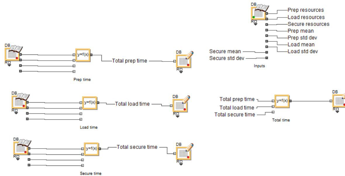
Figure 30. Database Management
