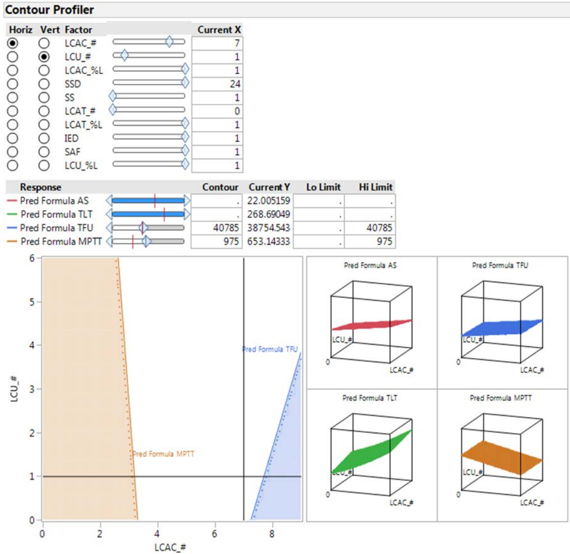
Figure 114. Scenario 11 Solution Space Contour Plot
