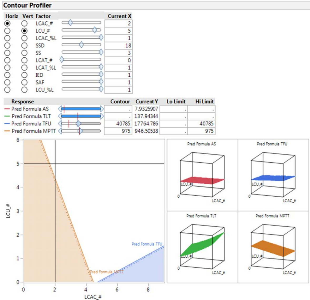
Figure 94. Scenario 4 Solution Space Contour Plot
