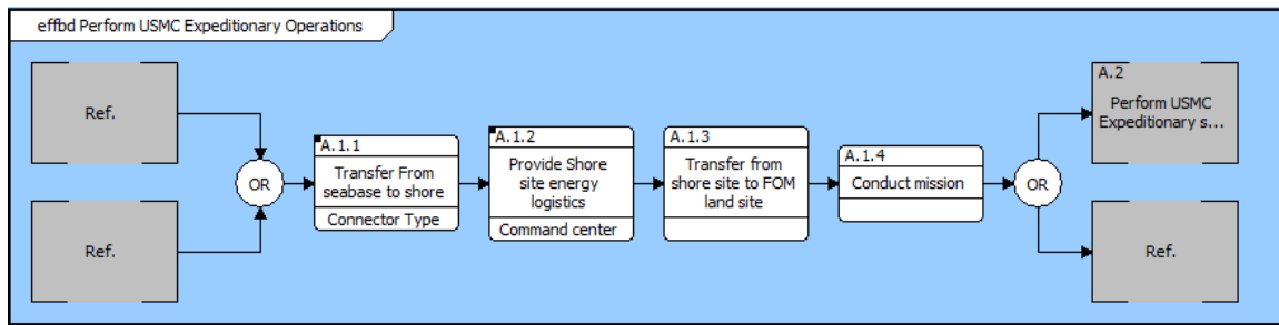
Figure 20. Functional Flow Block Diagram of the Perform USMC Expeditionary Operations Hierarchy
