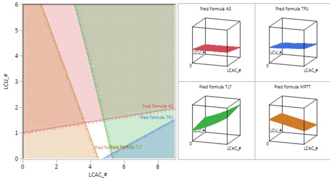
Figure 87. Scenario 1 Limiting Response Contour Plot
