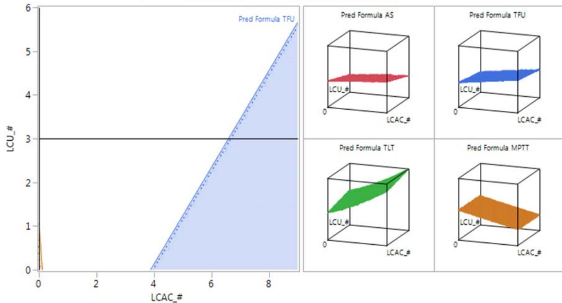
Figure 91. Scenario 3 Solution Space Contour Plot
