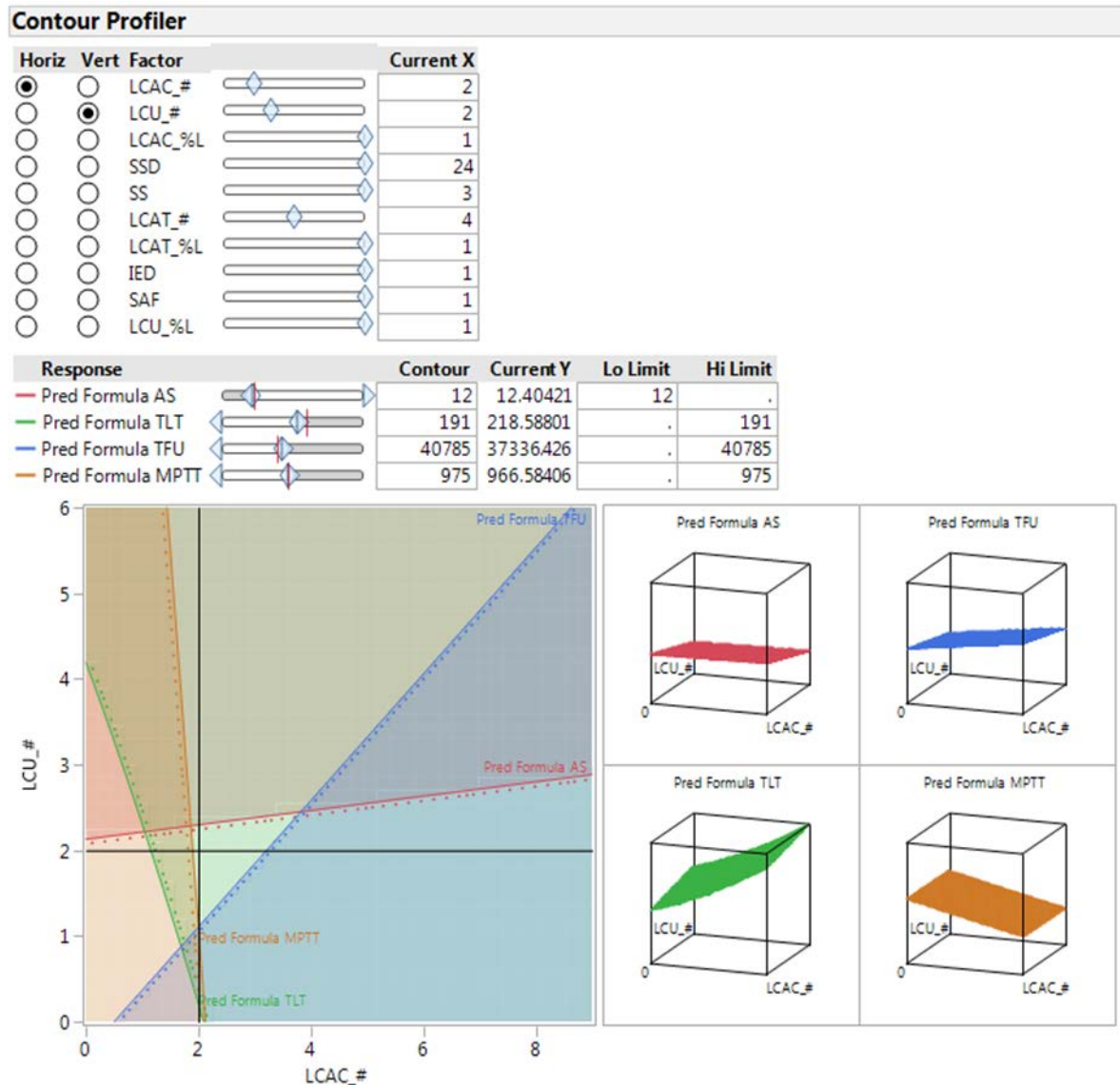
Figure 101. Scenario 6 Solution Space with TLT and AS Contour Plot
