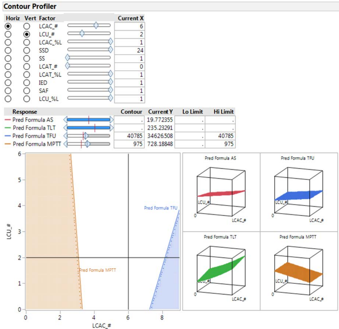
Figure 97. Scenario 5 Solution Space Contour Plot
