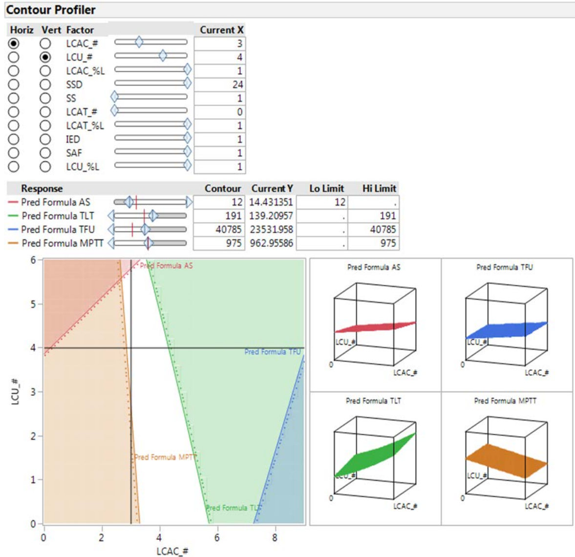
Figure 112. Scenario 10 Solution Space with TLT and AS Contour Plot
