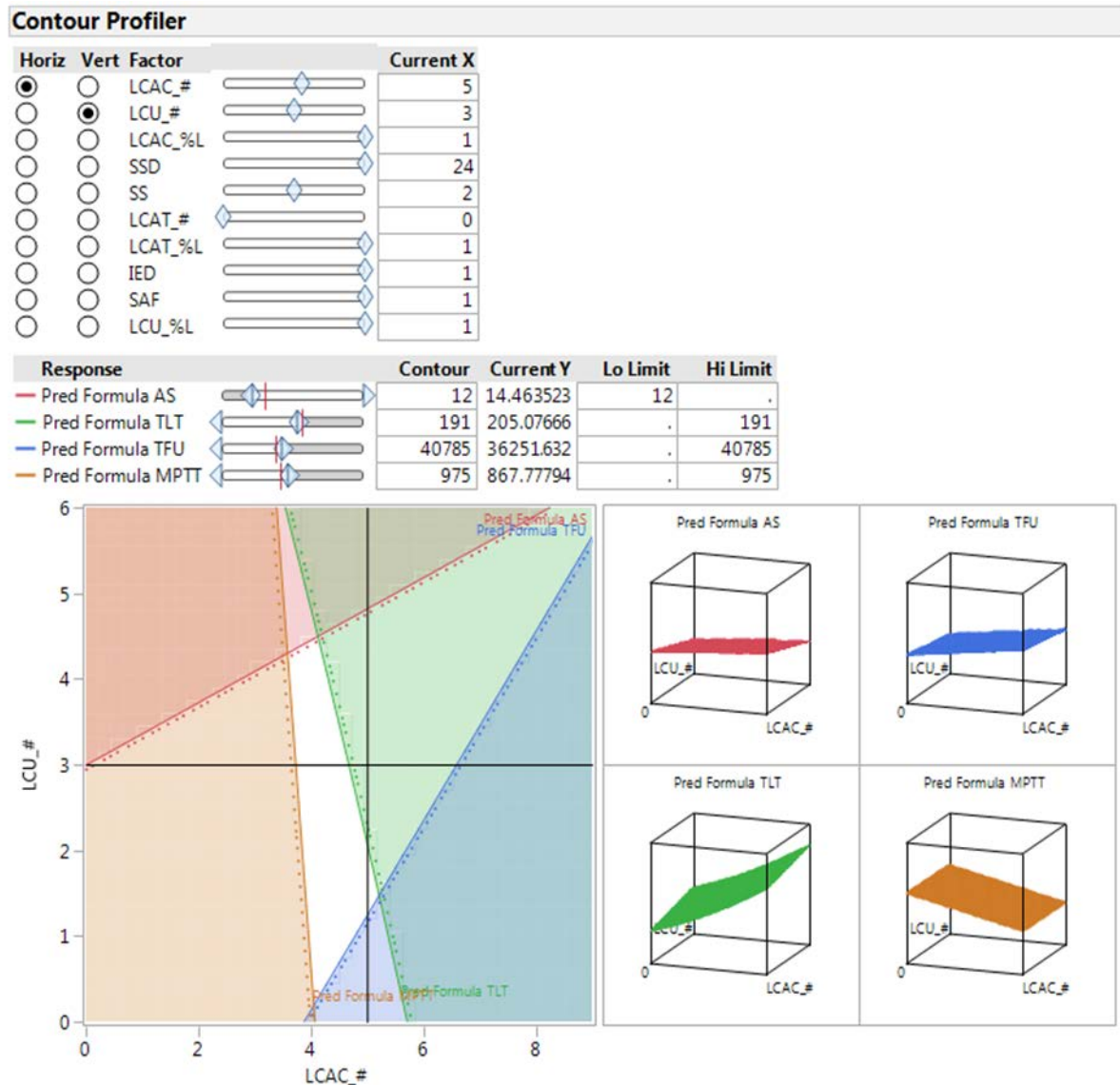
Figure 121. Scenario 13 Solution Space with TLT and AS Contour Plot
