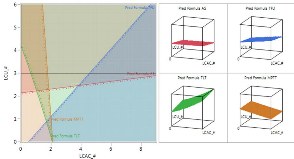
Figure 93. Scenario 3 Limiting Response Contour Plot
