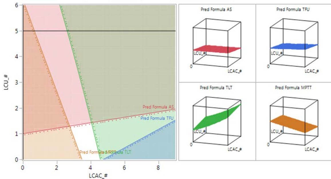
Figure 104. Scenario 7 Limiting Response Contour Plot
