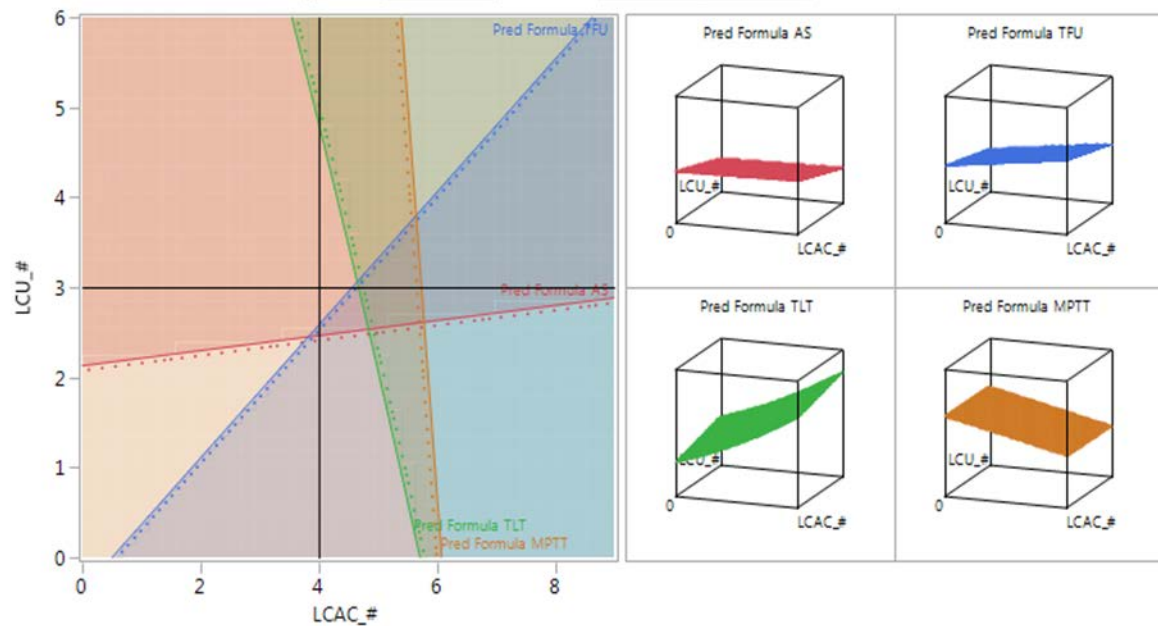
Figure 90. Scenario 2 Limiting Response Contour Plot
