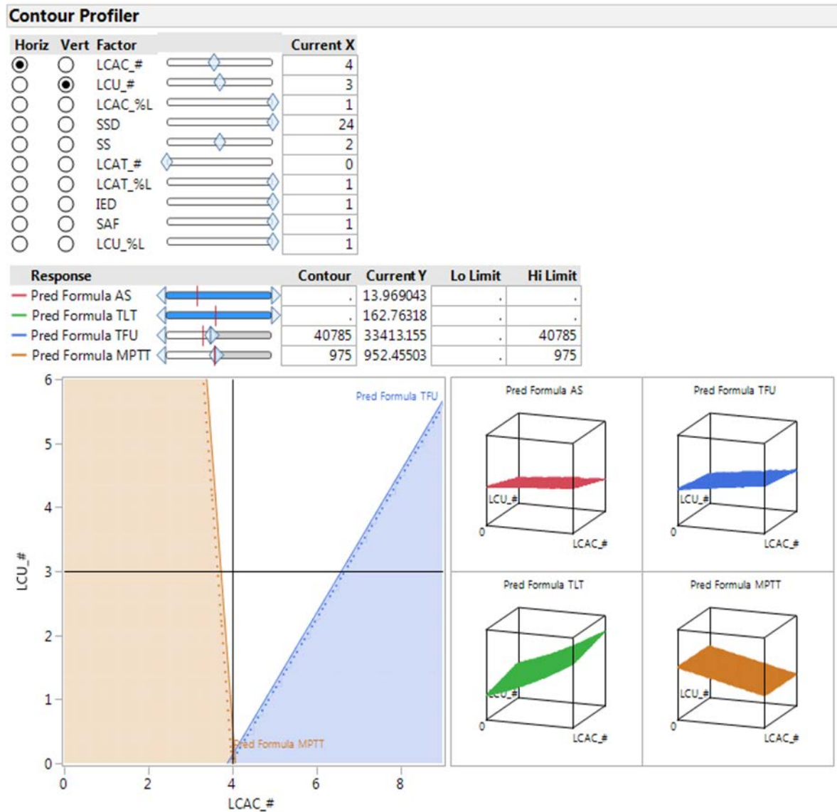
Figure 88. Scenario 2 Solution Space Contour Plot
