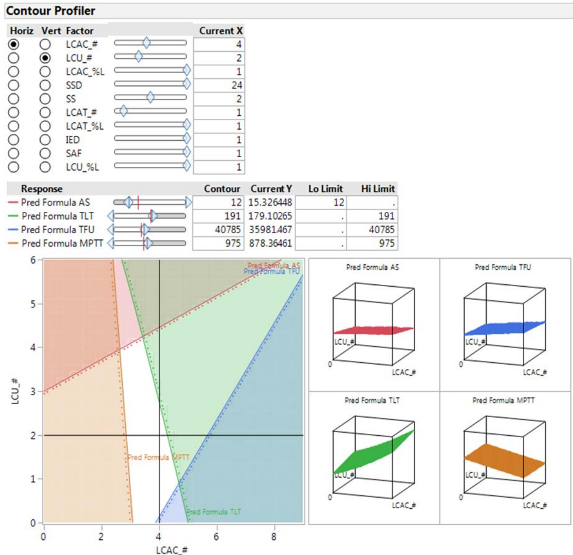
Figure 106. Scenario 8 Solution Space with TLT and AS Contour Plot
