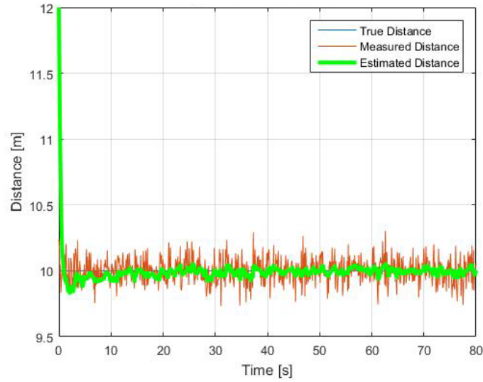
Figure 24. Longitudinal Distance for a KF with Two Inputs
