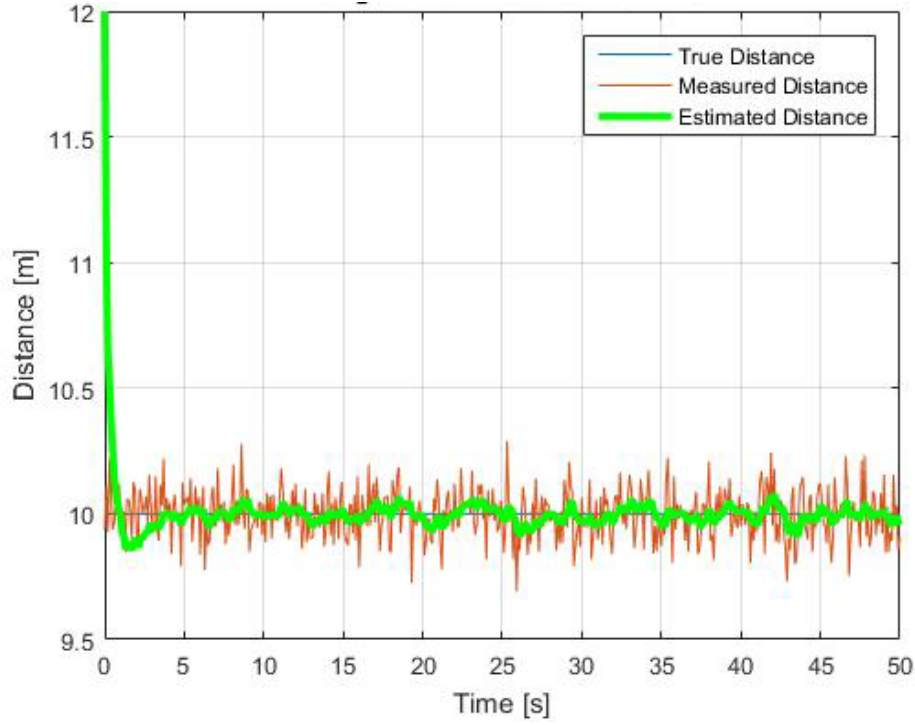
Figure 21. Longitudinal Distance for a KF with One Input
