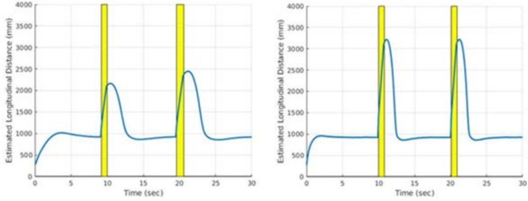
Figure 30. Position Estimation with Occlusions for q=100 (left) & 1000 (right)
