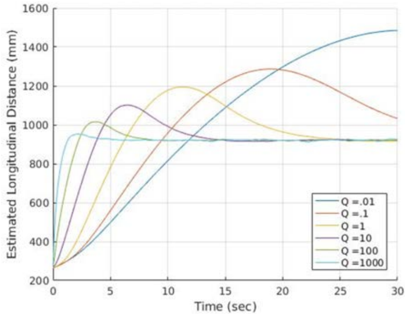
Figure 29. Position Estimation for Varying Q Values
