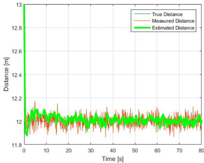
Figure 25. Vertical Distance for a KF with Two Inputs
