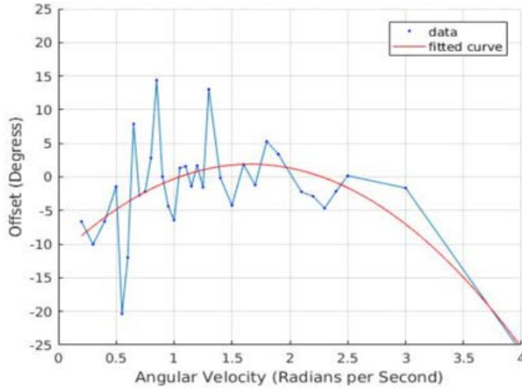
Figure 12. Average Offset for Various Angular Velocities
