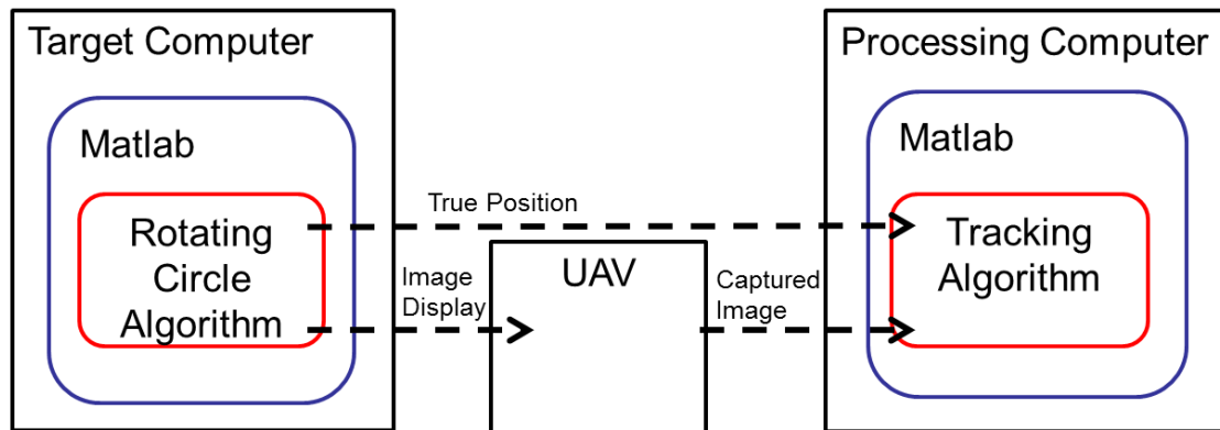
Figure 11. Experimental Architecture
