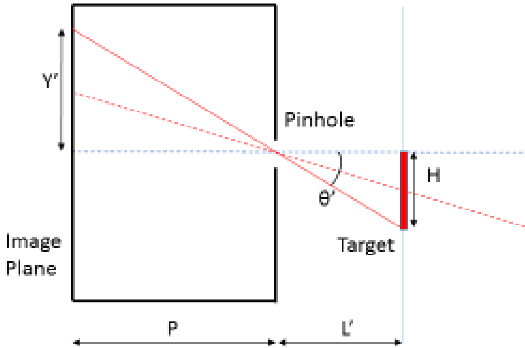
Figure 2. Pinhole Camera with Closer Target
