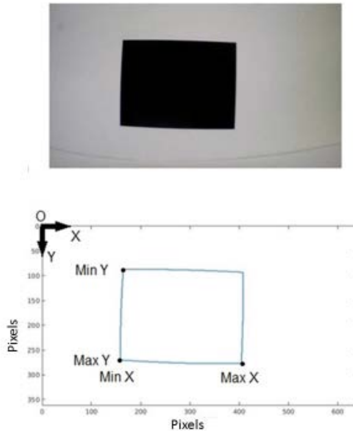
Figure 3. Maximum and Minimum Values of Edge Detection
