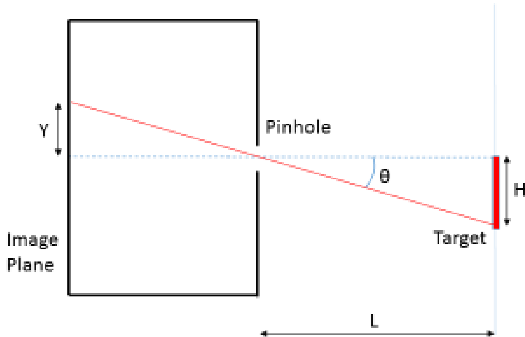
Figure 13. Pixel Size, Y , to Angle, \theta , for Pinhole Camera Model
