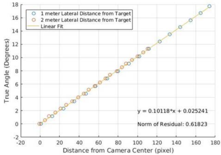
Figure 19. True Angle for Various Pixel Distances from Image Center
