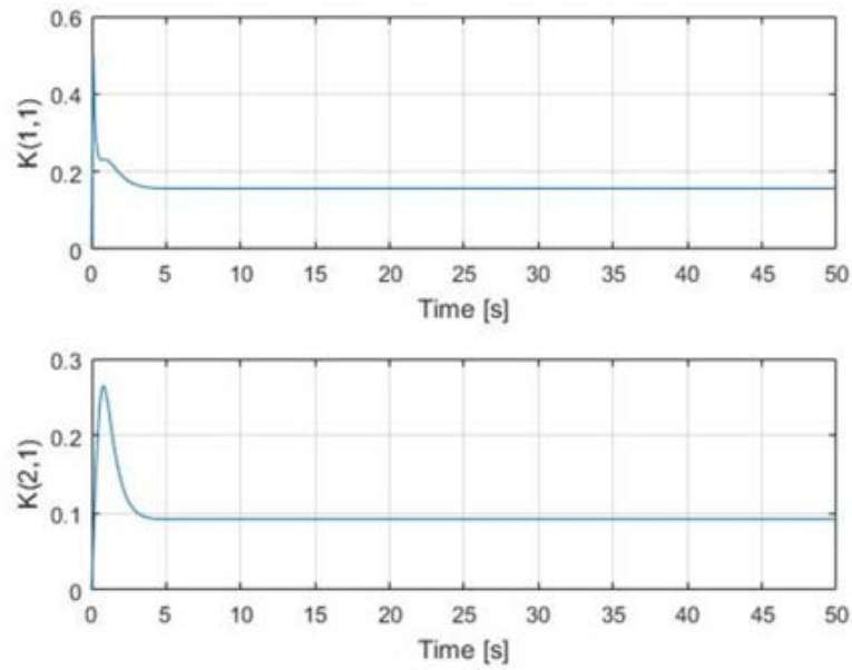
Figure 22. Kalman Gain for a KF with One Input
