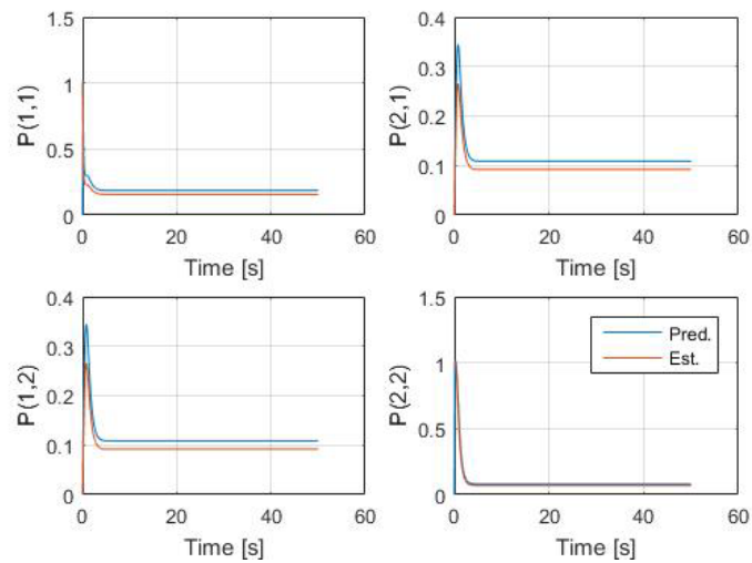
Figure 23. Estimation Error Matrix for a KF with One Input
