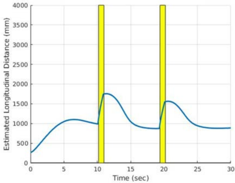
Figure 31. Position Estimation with Occlusions for q=10
