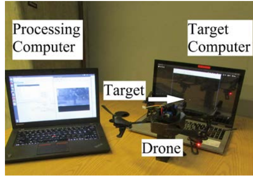
Figure 10. Experimental Setup to Characterize Image Target Acquisition
