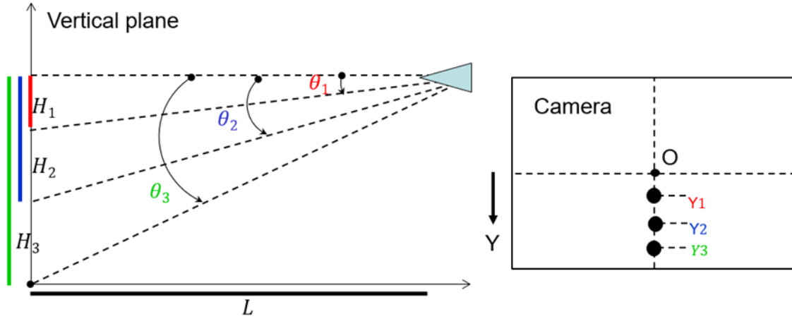
Figure 17. Target Position and Camera Image for Various Heights of Target
