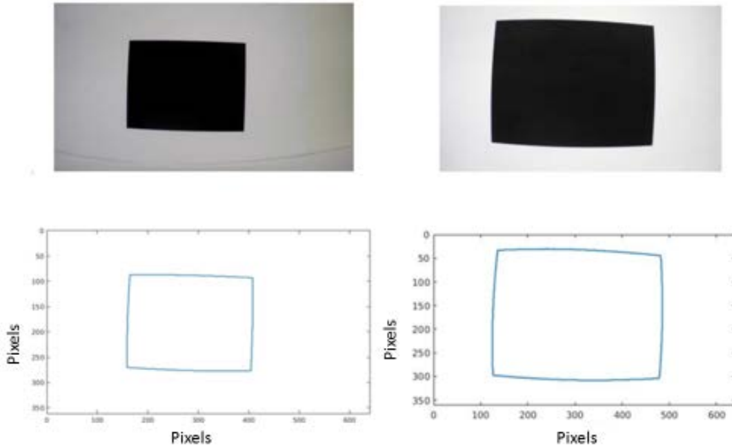
The top frames are the captured images of the target. The upper left frame is the reference image while the upper right frame is the variable image. The bottom frames are the resultant edge detections from the captured images.
