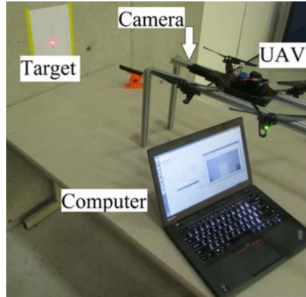
Figure 18. Angle Calibration Experiment Setup
