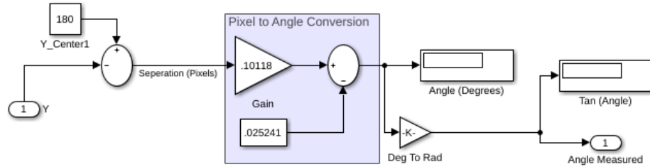
Figure 20. Pixel to Angle Linear Equation Implemented into Simulink
