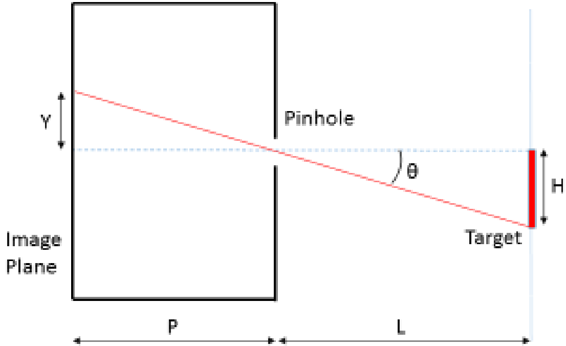
Figure 1. Theoretical Pinhole Camera
