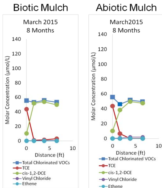
Figure 7. Results from subsurface bioreactors containing mulch after 8 months.
