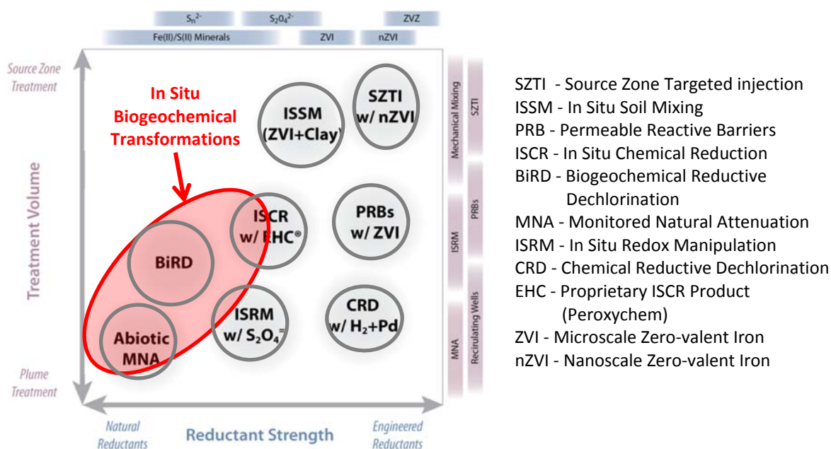
Figure 1. Map of ISCR technologies with range covered by in situ biogeochemical transformation (Modified from Tratnyek et al., 2014).
