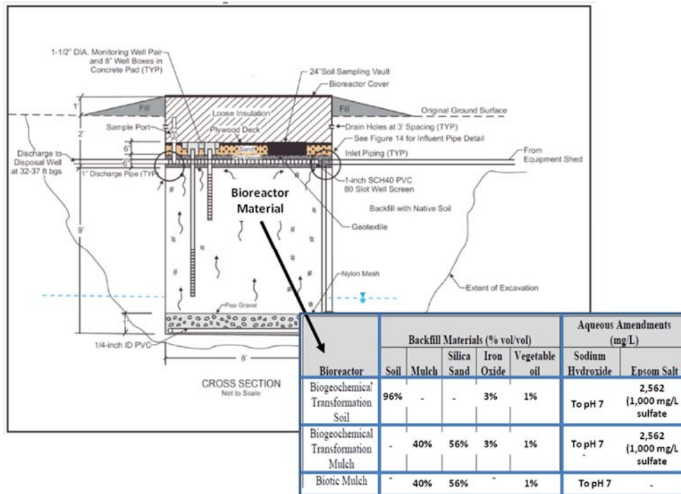
Figure 6. Subsurface bioreactor designs.
