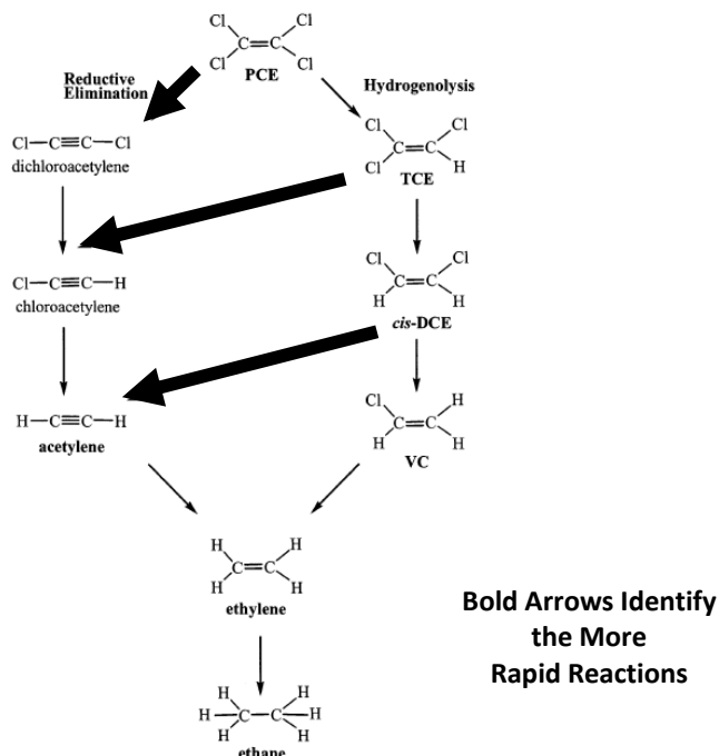
Figure 2. Major abiotic chloroethene degradation pathways and products ( trans -DCE and others occur at lower levels). Modified from Lee and Batchelor (2002) and He et al. (2015).
