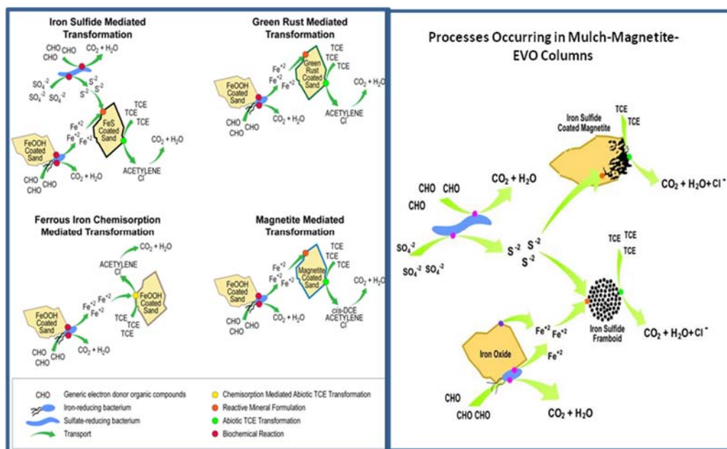
Figure 4. Biogeochemical transformation mechanisms. Left panel - AFCEE et al. (2008). Right panel - Conceptual model of this technology, based on abiotic mulch columns.
