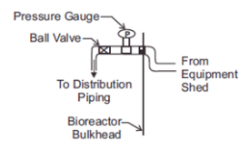
INFLUENT DETAIL
