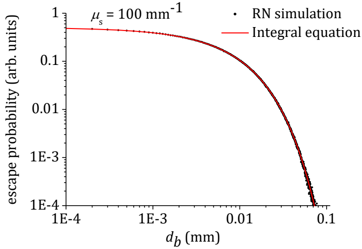
Figure 8. Escape probability P_{esc}(d_b) , computed with random number simulations and with Eq. (10).
