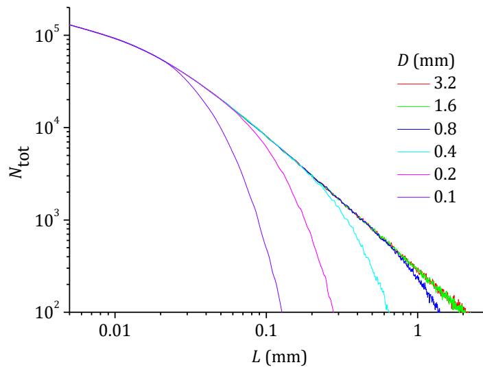
Figure 4. Integrated pathlength distributions for different values of slab thickness D
