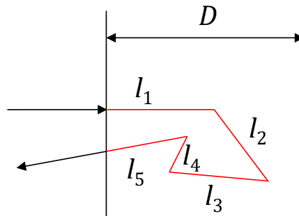
Figure 1. Schematic of multiple scatter events inside a TBC
