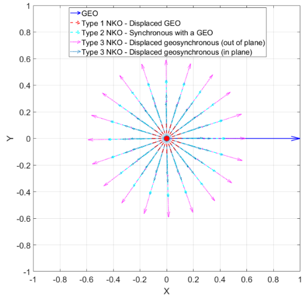
Figure 9. Time evolution of the osculating eccentricity vector. X-Y view.
