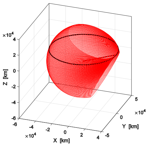
Figure 27. Test case 1. Known NKO (black) and other NKO, which are part of the family (red), are shown.
