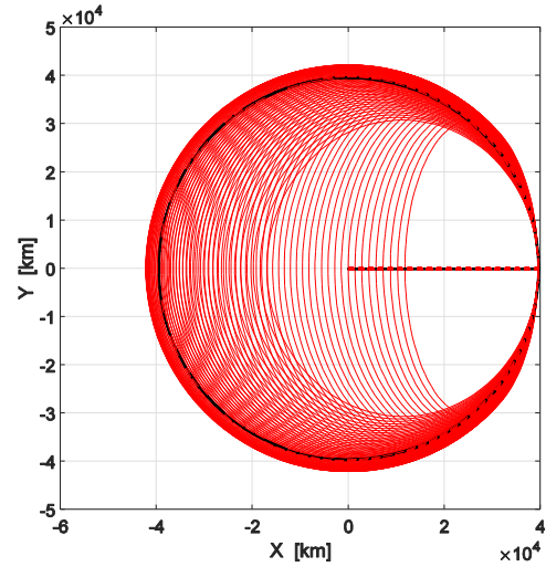
Figure 28. Test case 1. Known NKO (black) and other NKO, which are part of the family (red), are shown. X-Y view.
