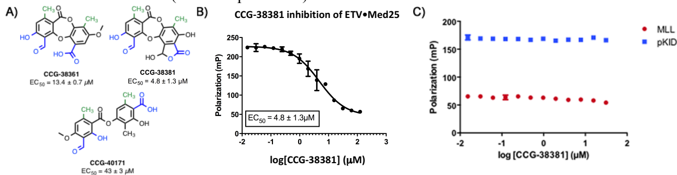
Figure 2. A) Structures of the three first ETV4•Med25 inhibitors along with EC 50 values from full dose-response experiments. Functional groups colored in blue and green are likely to be key for binding and inhibition, when compared to related depside and depsidones. B) Representative curve of CCG-38381 inhibition against the Med25•ETV transcriptional activation domain complex (average of 3 independent experiments). C) Representative experiment with CCG-38381 showing no inhibition against another coactivator motif, CBP KIX, and two of its binding partners, MLL and the phosphorylated KID domain of CREB (pKID).
