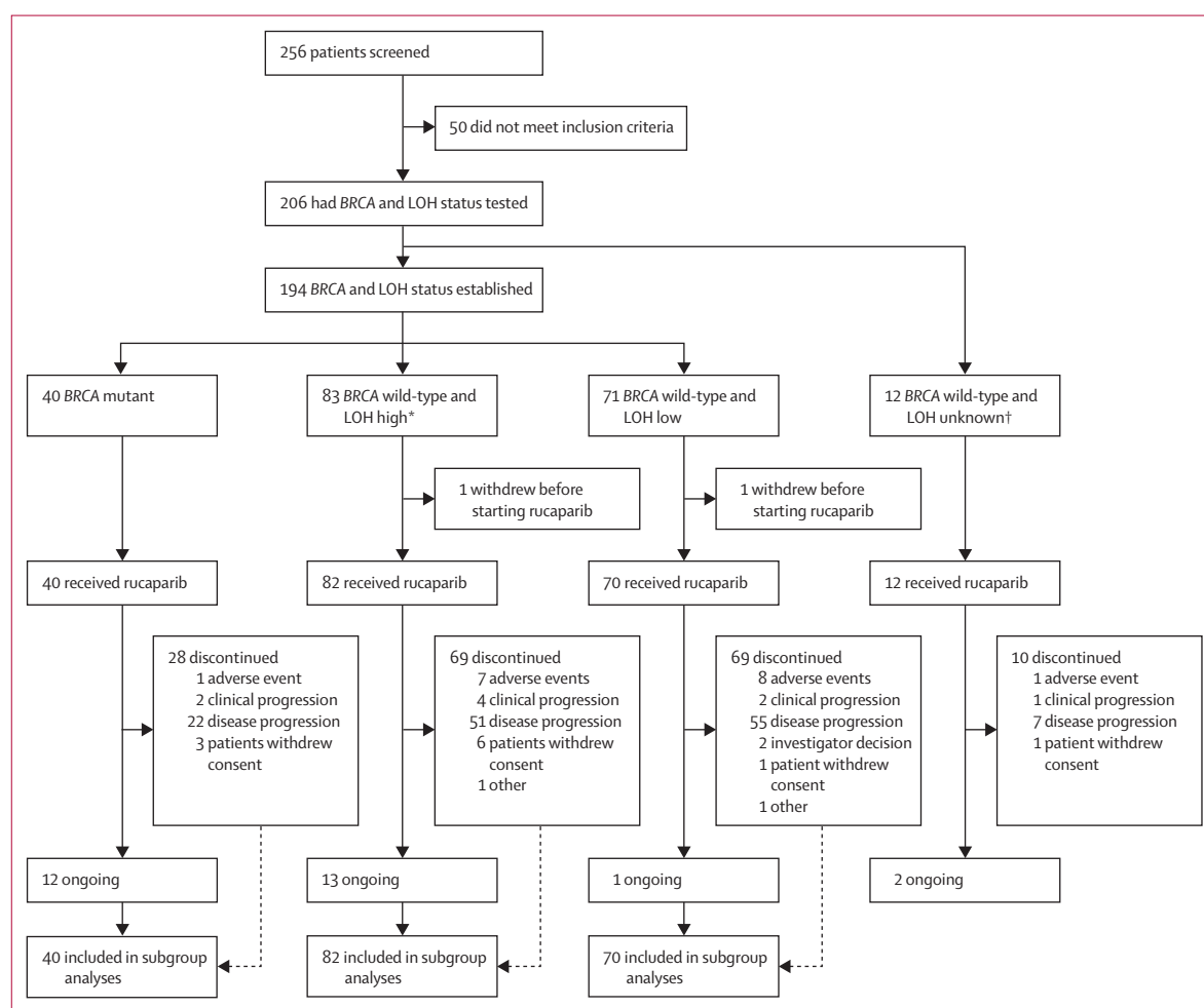
Figure 1: Trial profile
