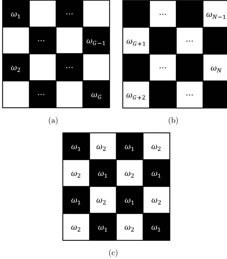
Figure 7. SLM segment diagram for parallel wavefront optimization. (a) Group 1 segments (black) are modulated, each at a distinct frequency, while Group 2 segments (white) are static. (b) Group 2 segments (white) are modulated, each at a distinct frequency, while Group 1 segments (black) are static. (c) All Group 1 segments (black) are modulated at \omega_1 , while all Group 2 segments (white) are modulated at \omega_2 (similar to Figure 2 from reference [17], modified for clarity).
