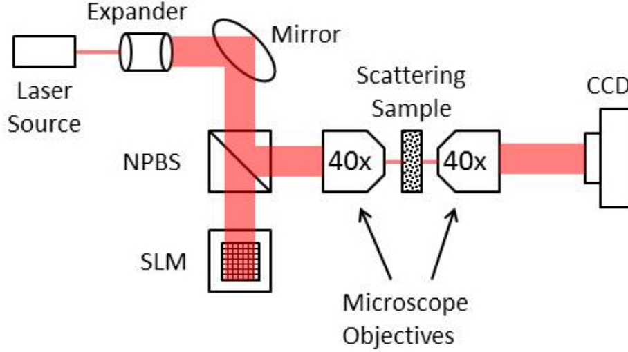
Figure 1. Optical setup for transmissive inverse diffusion. A microscope objective is used to demagnify the modulated beam and image it onto the scattering medium. The transmitted scatter pattern is magnified by a second microscope objective and image onto the feedback CCD.
