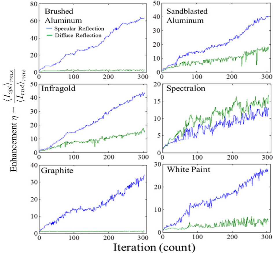
Figure 3. Enhancement comparisons of specular and diffuse regions of reflection. Enhancement is plotted after each optimization with the CCD placed in the specular region at 45^\circ from the reflector surface normal (blue). Specular is defined as a reflection angle of 45^\circ \pm 0.5^\circ from the surface normal. Diffuse is defined as 15^\circ off specular.
