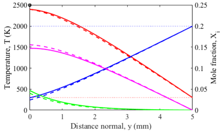
Figure 13. A_3 sensitivity of 1D Flame model with T_s = 2500 K and \delta = 5 mm. A_3 : (-.-) A_3 = 0 , (-) A_3 = A_3^o , (- -) A_3 = 100 x A_3^o . (-) X_{CO} , (-) X_{O_2} , (-) X_{CO_2} , (••) X_{O_2}^o , (-) T_{plume} , (••) T_{plume}^o , (□) T_s
