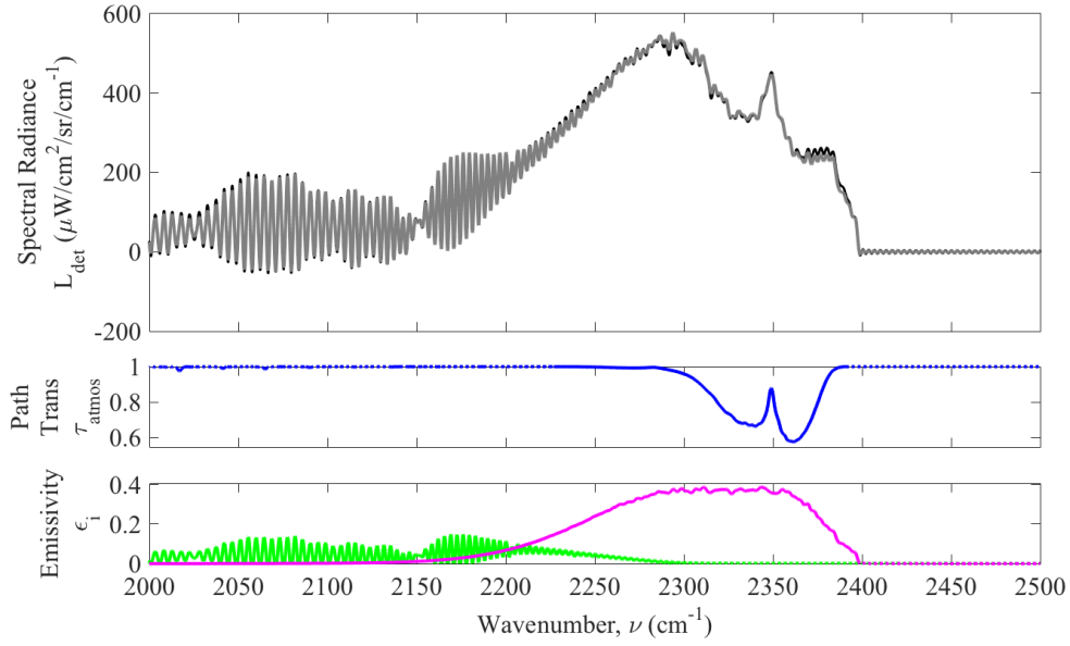
Figure 62. Sample two-layer model fit to simulated line of sight spectra. (---) simulated measured radiance, (—) two-layer RTM radiance, (—) \tau_{atmos} ; (—) \epsilon_{CO} ; (—) \epsilon_{CO_2} . Model fits correspond to q_{CO} = 0.492 \pm 0.002 cm, q_{CO_2} = 0.139 \pm 0.0004 cm, and T_{plume} = 1388 \pm 1 K,
