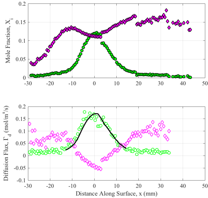
Figure 35. Diffusion flux along surface for isomolded sample irradiated at 1000 \text{ W/cm}^2 . Diffusion flux calculated using Eq. (120): (○) \Gamma_{CO} , (◇) \Gamma_{CO_2} . Diffusion flux approximated using Eq. (128): (—) \Gamma_{CO}
