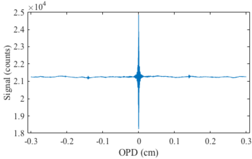
Figure 3. Sample interferogram, MOPD = 0.3 cm, nOPD = 9480
