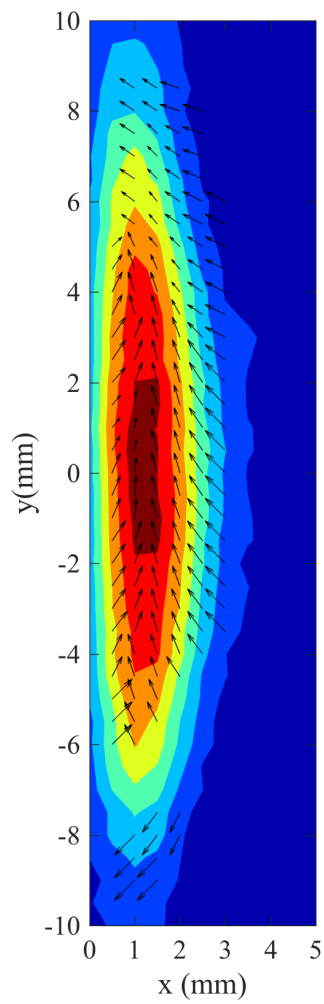
Figure 52. Velocity field for stagnation flow ( v=1.5 \text{ m/s} ) on sample irradiated at 2400 \text{ W/cm}^2 . Broad-band image in background included for spatial reference.
