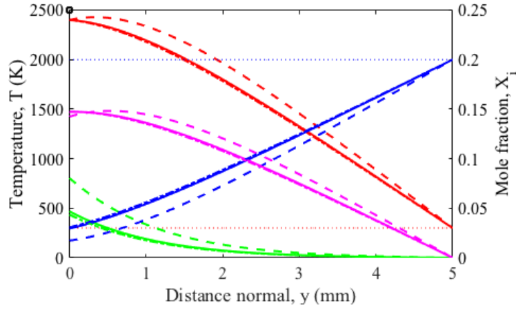
Figure 12. A_2 sensitivity of 1D Flame model with T_s = 2500 K and \delta = 5 mm. A_2 : (-.) A_2 = 0.1 \times A_2^o , (-) A_2 = A_2^o , (- -) A_2 = 10 \times A_2^o . (-) X_{CO} , (-) X_{O_2} , (-) X_{CO_2} , (· ·) X_{O_2}^o , (-) T_{plume} , (· ·) T_{plume}^o , (□) T_s
