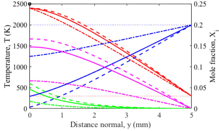
Figure 11. A_1 sensitivity of 1D Flame model with T_s = 2500 K and \delta = 5 mm. A_1 : (-.-) A_1 = 0.1 x A_1^o , (-) A_1 = A_1^o , (- -) A_1 = 10 x A_1^o . (-) X_{CO} , (-) X_{O_2} , (-) X_{CO_2} , (••) X_{O_2}^o , (-) T_{plume} , (••) T_{plume}^o , (□) T_s
