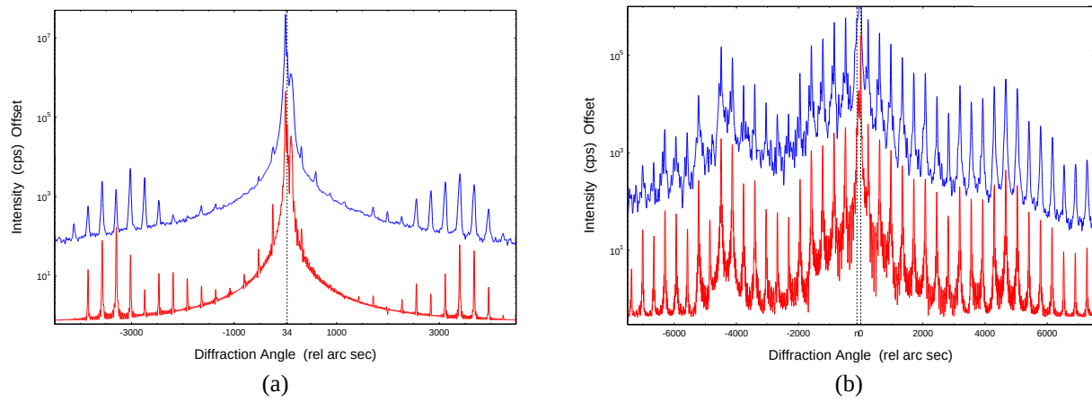
Figure 6. High-resolution x-ray diffraction scans (upper) and simulations (lower) of (a) LM LWIR QCL and (b) SC MWIR QCL.
