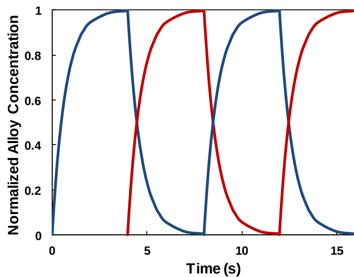
Fig. 3 Schematic precursor concentration profiles at the epilayer surface as a function of time for in MOVPE growth. The grading is due to a fundamental phenomenon of gas phase dispersion operative in this growth process. Reducing the growth rate and the introduction of a growth interrupt between layers will reduce compositional grading at heterointerfaces
