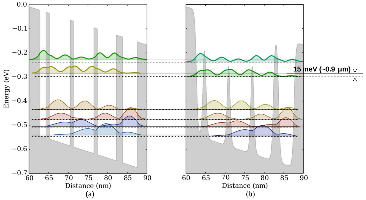
Fig 11. Calculated conduction band diagram and moduli squared of the wave functions for the active region of the QCL with compositionally (a) abrupt interfaces (8.2 \mu\text{m} lasing transition) and (b) graded interfaces (9.1 \mu\text{m} lasing transition). The barrier heights of the three thinner barrier layers are considerably lower and consequently the lasing transition energy is reduced by 15 meV.
