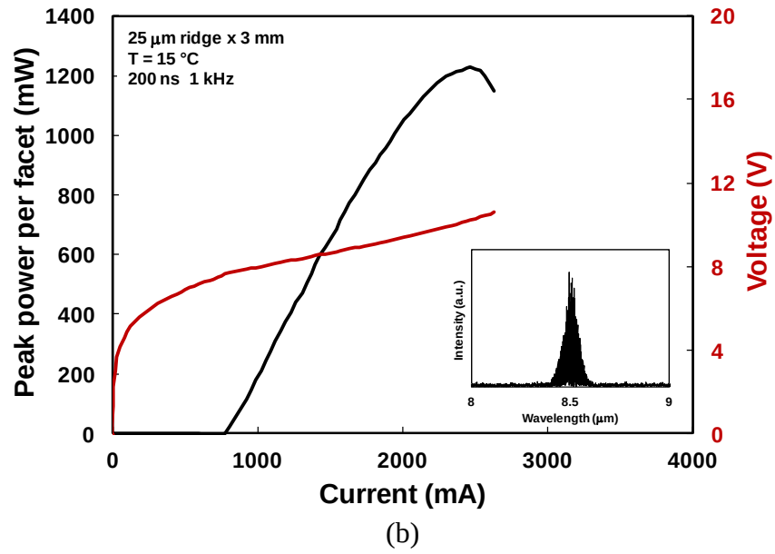
Fig. 13. Pulsed mode power operation of probe-tested uncoated QCLs designed with graded interfaces: (a) 7.5 \mu\text{m} design and (b) 8.5 \mu\text{m} design. The inset shows the emission spectrum measured just above threshold.
