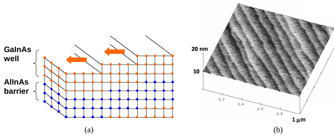
Fig. 2 (a) Schematic of epitaxial surface during growth and (b) atomic force microscope image of InP epilayer surface with monolayer step heights and ‘straight’ step edges.
