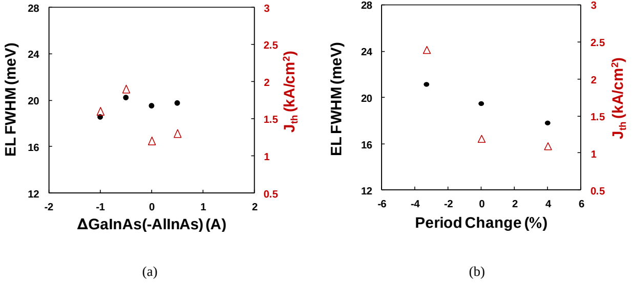
Fig. 9. Electroluminescence spectra full-width at half-maximum (EL FWHM) and threshold current density ( J_{th} ) for (a) complementary thickness changes and (b) period changes.
