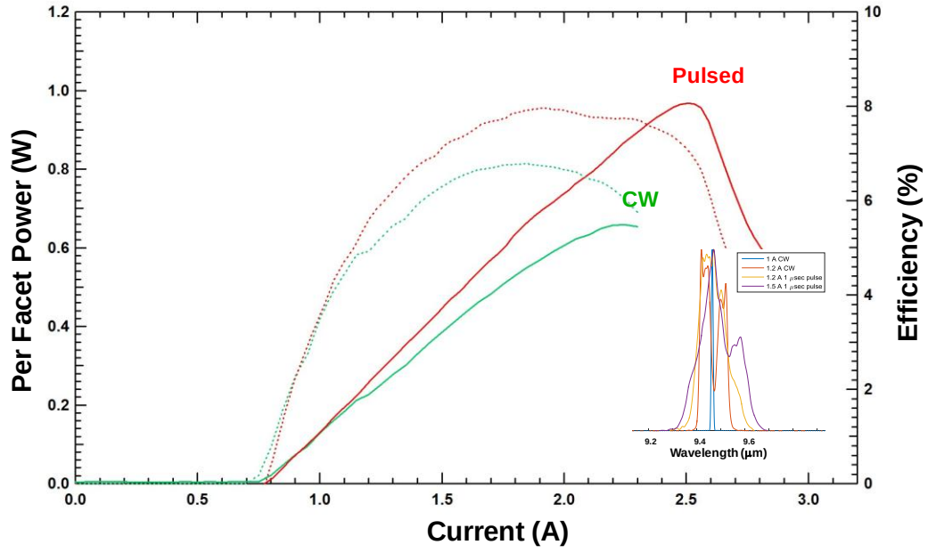
Fig. 14. Room-temperature continuous-wave operation of uncoated 12 \mu\text{m} x 5 mm-long QCL .
