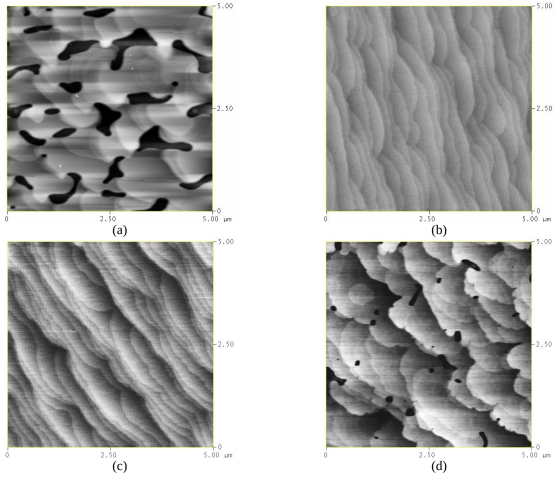
Fig. 4 (a) Atomic force microscopy (AFM) images ( 5 \times 5 \mu\text{m}^2 ) illustrate the high sensitivity of surface morphology to growth conditions. AFM images are for AlInAs grown at 580^\circ\text{C} with tertiarybutylarsine and different growth rates or V/III ratios: (a) growth rate of 0.15 \text{ nm/s} ; (b) growth rate of 0.28 \text{ nm/s} ; (c) \text{V/III} = 2.5 ; and (d) \text{V/III} = 20 . The root-mean-square roughness of the surfaces shown (a) – (d) are 2.3 , 0.175 , 0.276 , and 0.588 \text{ nm} , respectively.
