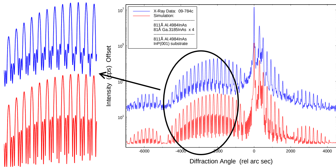
Fig. 5 High-resolution x-ray diffraction scans of a AlInAs/GaInAs MQW. Upper curve is the measured data, and the lower curve is a simulation using Philips X'pert software (PANalytical Inc.). Alloy compositions are determined from angular position and thickness from angular spacing. The full-width at half-maximum of satellite diffraction peaks and interference fringes between satellites are a measure of the consistent periodicity from the initially grown layers to the uppermost surface.
