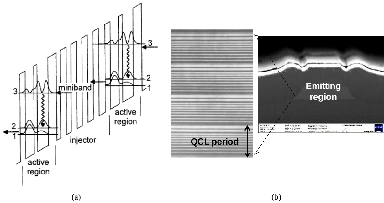
Fig. 1 (a) Schematic of conduction band energy diagram and wavefunctions of a QCL structure. One QCL period consists of the injector and active region, and the period is typically repeated 30-40 times in a full QCL structure. (b) Cross-section of buried heterostructure QCL (right) and transmission electron microscopy cross-section of a portion of a QCL core.
