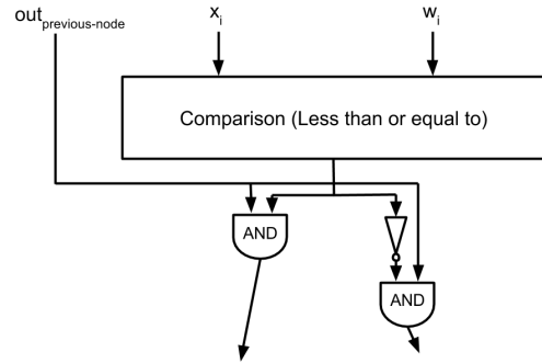
Figure 5: Decision tree classifier node evaluation circuit.
