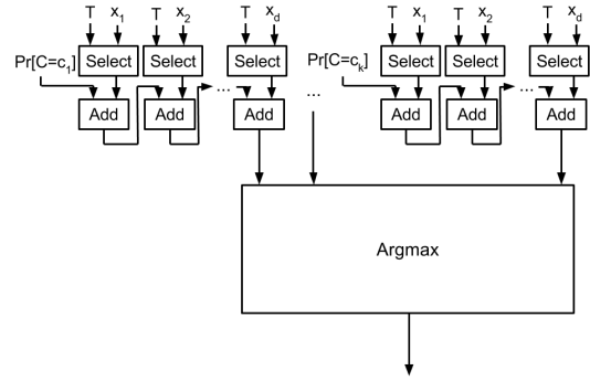
Figure 4: Naive Bayes classifier circuit.
