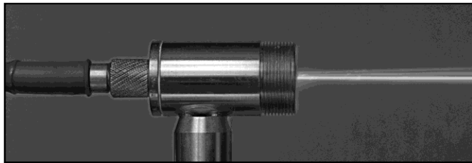
Figure 5. Fiber-coupled 266-nm frequency-quadrupled passively Q-switched microchip laser: (top) schematic and (bottom) photograph of working device mounted on 12.7-mm-dia. post.
