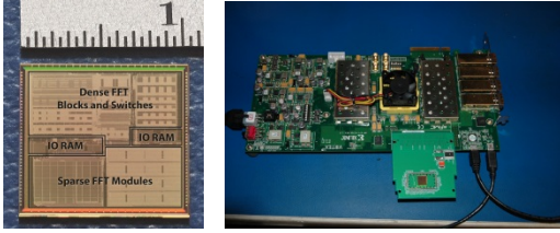
Figure 4: 1M point FFT ASIC kernel (as a standalone 1 cm 2 chip) and its testbed
