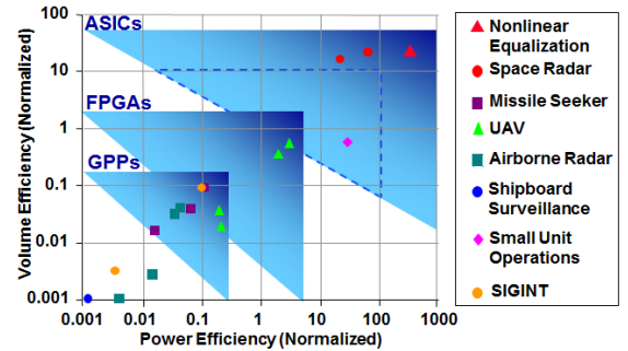
Figure 1: Embedded processing technology capabilities with the efficiency values normalized to account for Moore's Law (UAV: unmanned aerial vehicle; SIGINT: signals intelligence)
