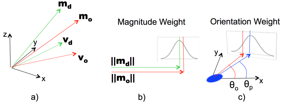
Figure 8: Method for weighting particles based on magnetic observation. a) the observed magnetic vector m_o and the database magnetic vector m_d , and their projections on the xy -plane: v_o and v_d respectively. b) the computation of the magnitude weight of a particle. c) the computation of the orientation weight of the particle. \theta_o is the estimated orientation of the particle computed from v_o and v_d in eq. (12).
