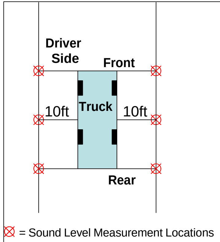
Figure 5-13 Meter Placement for Utility Truck Idle Measurements
