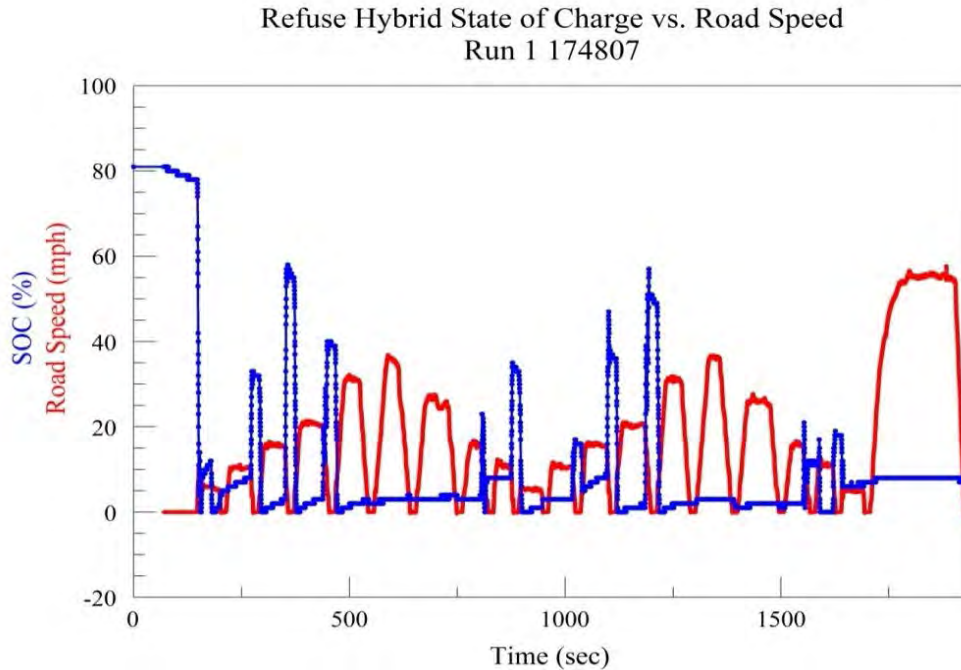
Figure 6-2. HLA SOC Activation during Fuel Economy Testing (US Army ATC Report No. 10546)
