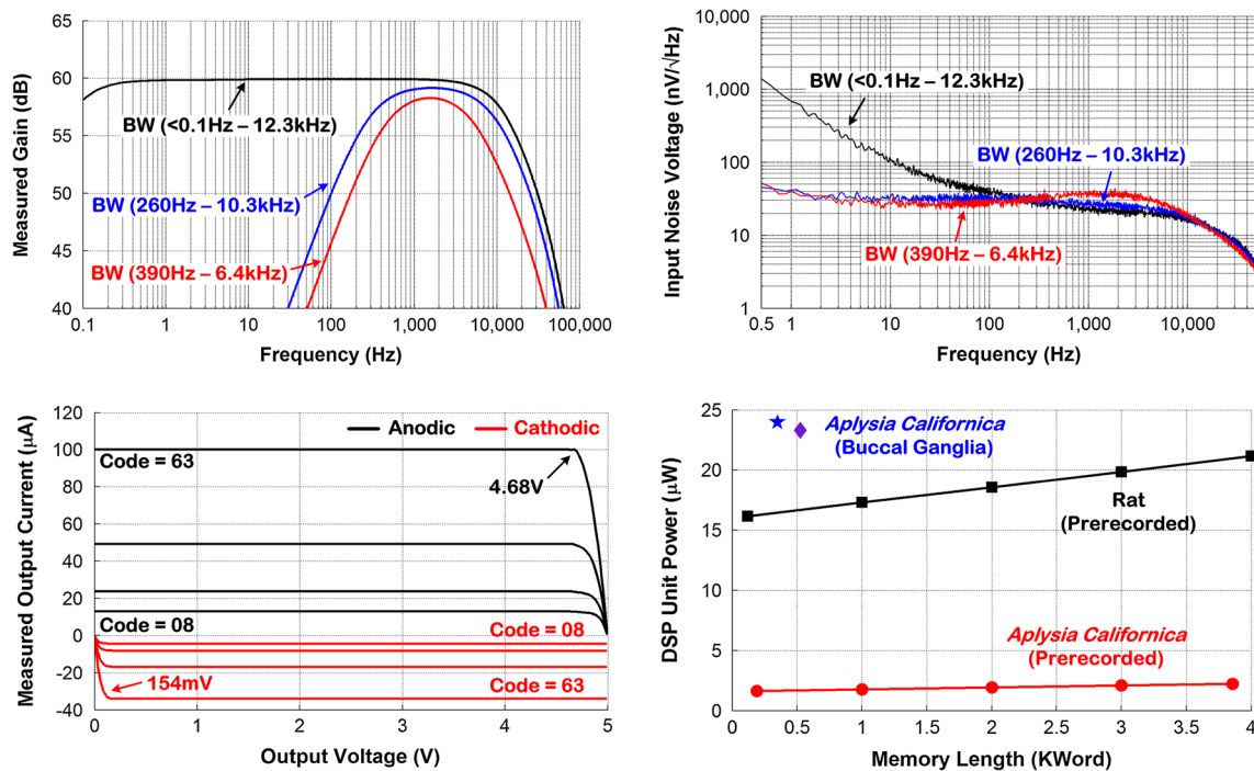
Fig. 7 Top—measured gain (left) and input noise voltage (right) of the analog recording front-end. Bottom—measured microstimulator output current versus output voltage in anodic and cathodic phases
