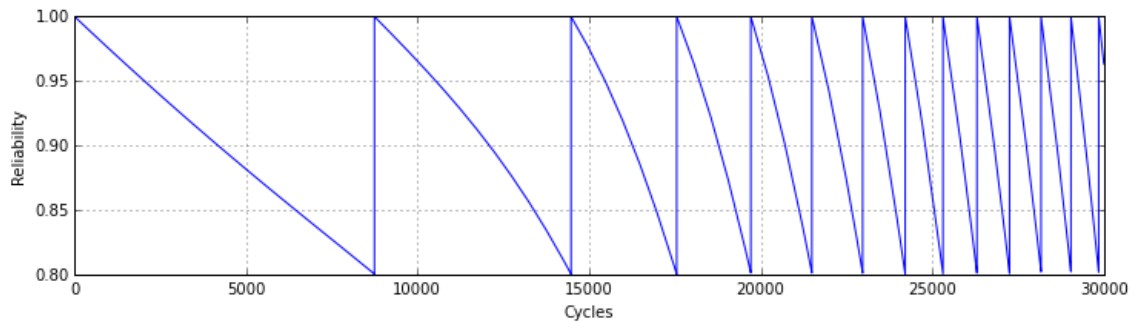
Fig. 3-6 Reliability for the case 3 (uncertain parameter d )
