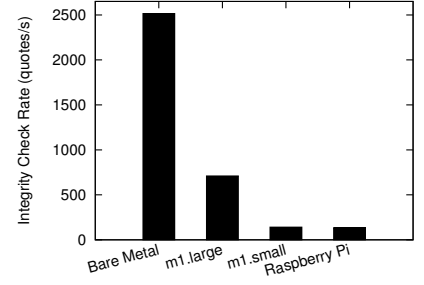
Figure 8: Maximum CV quote checking rate of keylime.
