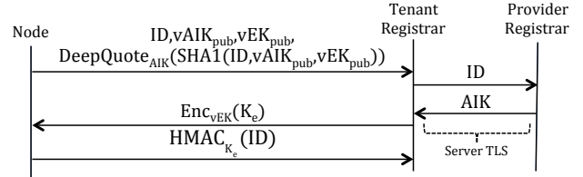
Figure 4: Virtual node registration protocol.
