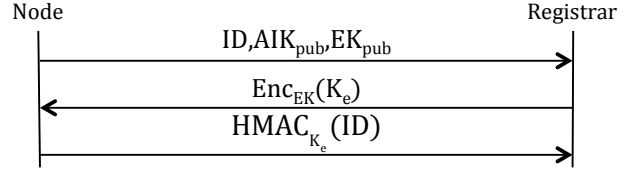
Figure 2: Physical node registration protocol.
