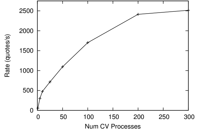
Figure 9: Scaling the CV on bare metal
