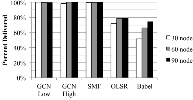
Fig. 4: Percentage of Packets Delivered, One-to-Many
