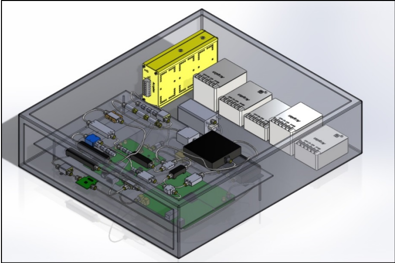
Figure 13: CAD model.
