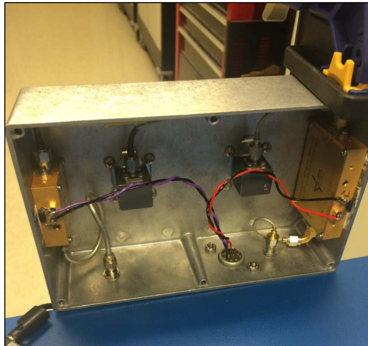
Figure 16: PA and LNA housing.
