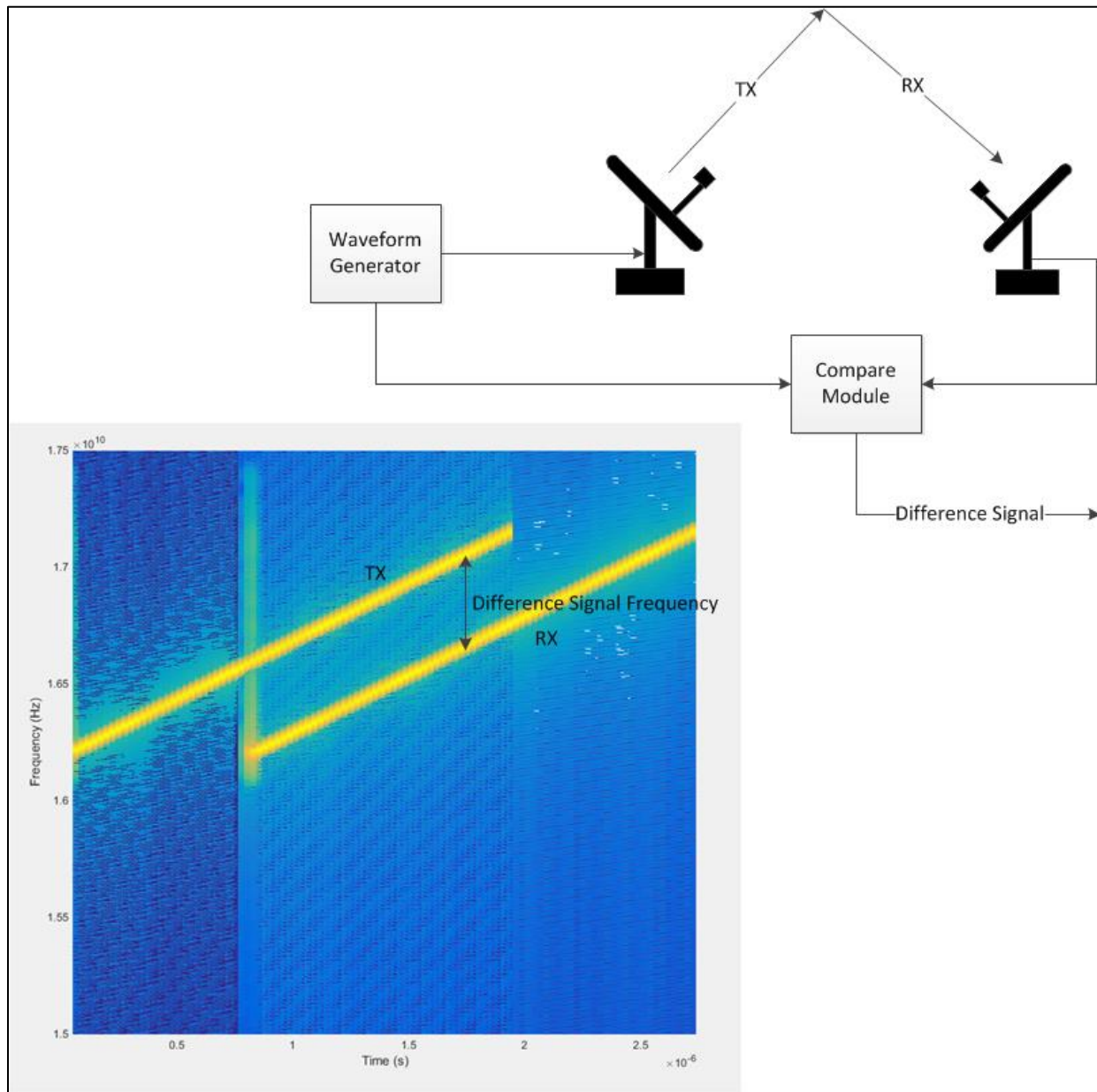
Figure 3: Stretch processing.
