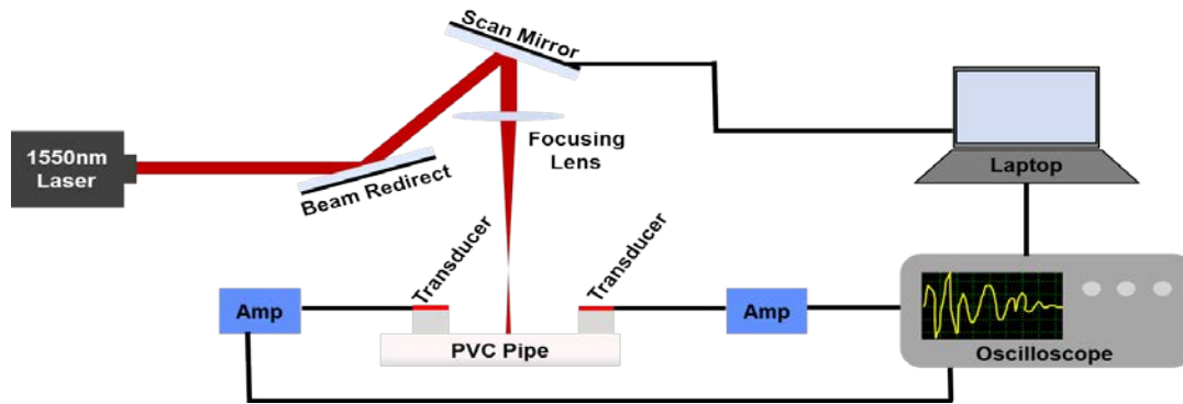
FIG. 1: The pulsed laser is directed to and focused near the surface of the PVC pipe, where elastic waves are generated and then picked up by the two Olympus V153 transducers. The signal is amplified by an Olympus 5072PR before being readout at a Tektronix TDS 2024B oscilloscope which is then recorded into a laptop using a Labview program. The scan mirror is for future experiments where we may vary the laser spot position.
