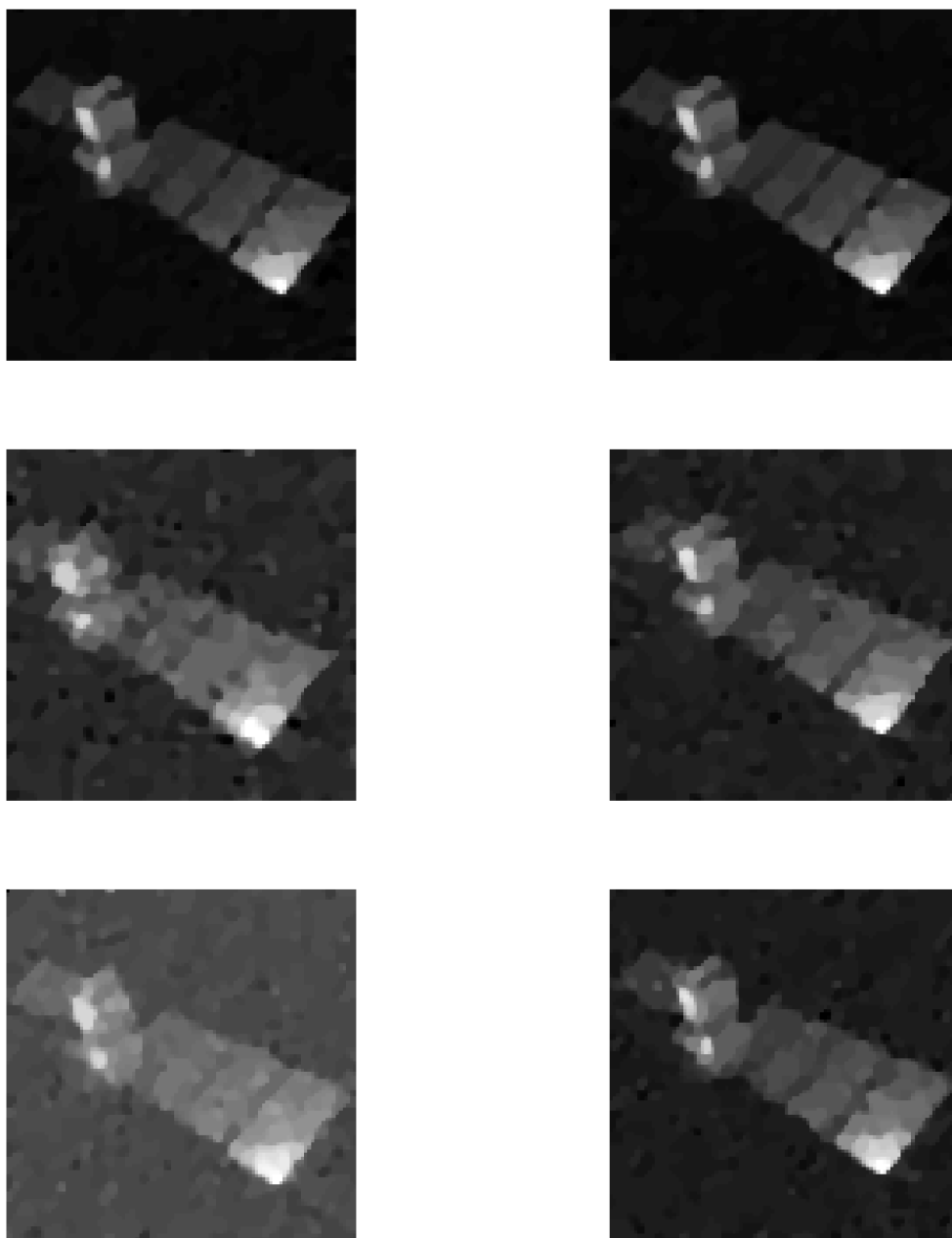
Figure 4.13: Fizeau Image Reconstruction Results. The reconstructions in the left column used traditional, three-baseline observables, whereas those in the right column used generalized closures selected according to Algorithm 3. (top row) n = 2e3 photoelectrons/aperture/frame (pe/ap/frame), 5e4 frames, (middle row) n = 2e3 pe/ap/frame, 1e3 frames, (bottom row) n = 5e2 pe/ap/frame, 5e4 frames.
