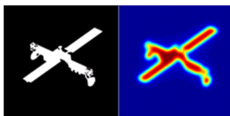
Figure 2.4: Target chrome mask (left) and corresponding truth image at diffraction-limited resolution (right)
