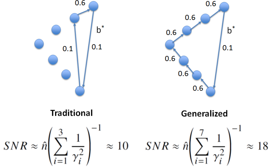
Figure 4.1: Generalizing the phase closure concept . SNRs given assume each aperture contributes \hat{n} = 2e3 photoelectrons to each fringe in pairwise combination.
