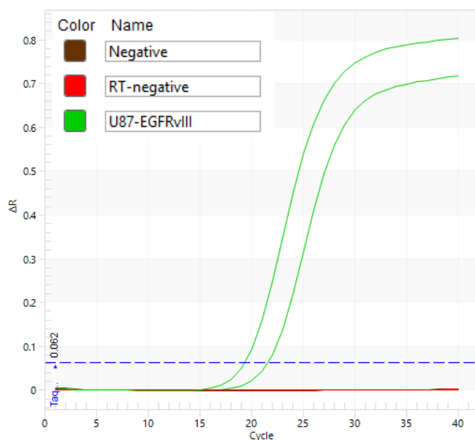
Figure 6 - Amplification of miR-16 TaqMan qPCR of RNA isolated from a glioblastoma cell line.
