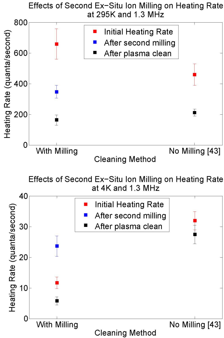
Figure 8-4: This figure compares heating rate reduction a second round of ion milling and plasma cleaning with the reduction from plasma cleaning alone, as seen in [2]. (top) Compares the heating rates at 295K and a secular frequency of 1.3 MHz, (bottom) at 4K and 1.3 MHz
