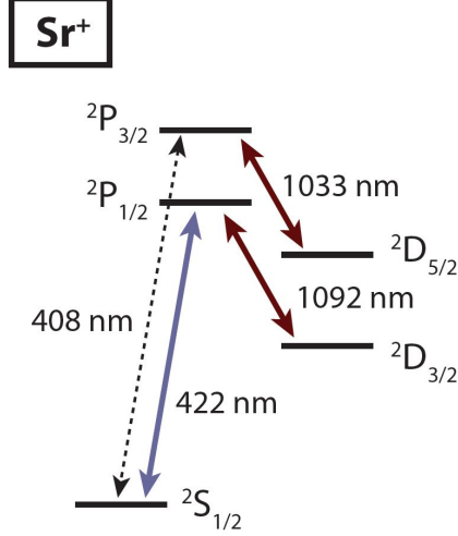
Figure 2-2: Lowest-lying energy levels of \text{Sr}^+
