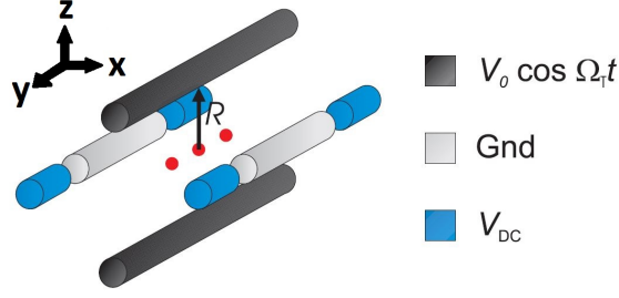
Figure 3-1: Diagram of a 3D Paul trap [29]
