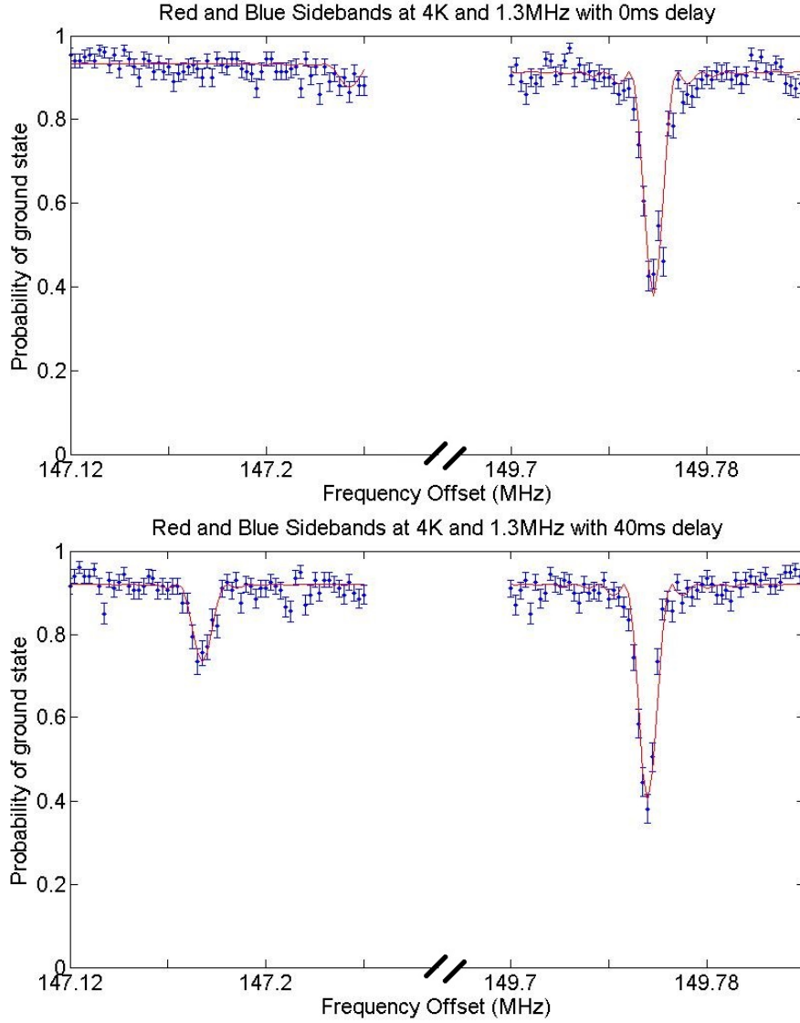
Figure 6-4: This figure displays representative fits for the red and blue sidebands of two different frequency scans. All data was taken at 4K with a trap frequency of 1.3 MHz for a standard 50\text{ }\mu\text{m} trap before any cleaning. The first plot shows the fits of the red and blue sidebands with a 0ms delay. The second shows the fits for the red and blue sidebands after a 40 ms delay. The heating rate fit for this data is shown in Figure 6-5.
