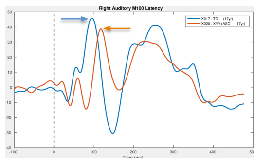
Fig. 1a MEG recorded auditory evoked field source waveforms from right hemisphere Heschl's gyrus in a representative 17-year old with typical development (blue) vs. an XYY participant on the autism spectrum (XYY+ASD), who exhibits a profound delay in the M100 peak (arrows).
