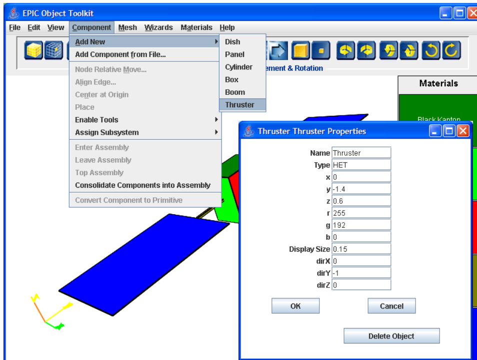
Figure 129. Thruster Definition for EPIC Object. Thruster Is Located at (0.0, -1.4, 0.6) and Is Pointed in the -Y Direction.
