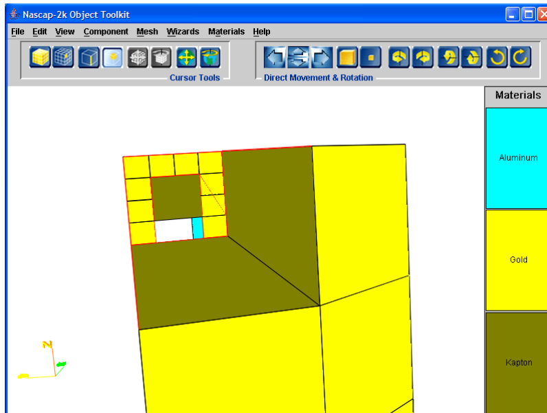
Figure 90. Here, Object Toolkit Misinterpreted the Attempt to Create a New Element Using the Four Corner Nodes.
