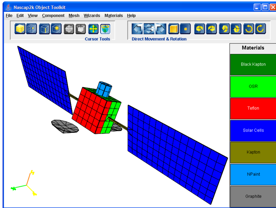
Figure 53. Object Toolkit Model of a Typical Geosynchronous Spacecraft to Be Built in this Example.
