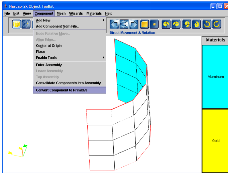
Figure 81. Converting the Outer Surface to a Primitive. The Outlines of Elements with Normals Facing into the Screen Are Seen.
