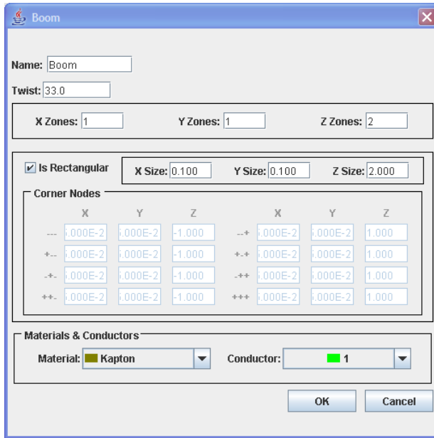
Figure 66. Defining a Boom to Support a Solar Array. The Boom Is 2.0 m Long, Has Two Elements in the Long Direction, and Has a Twist of 33. The Boom Material Is Kapton.
