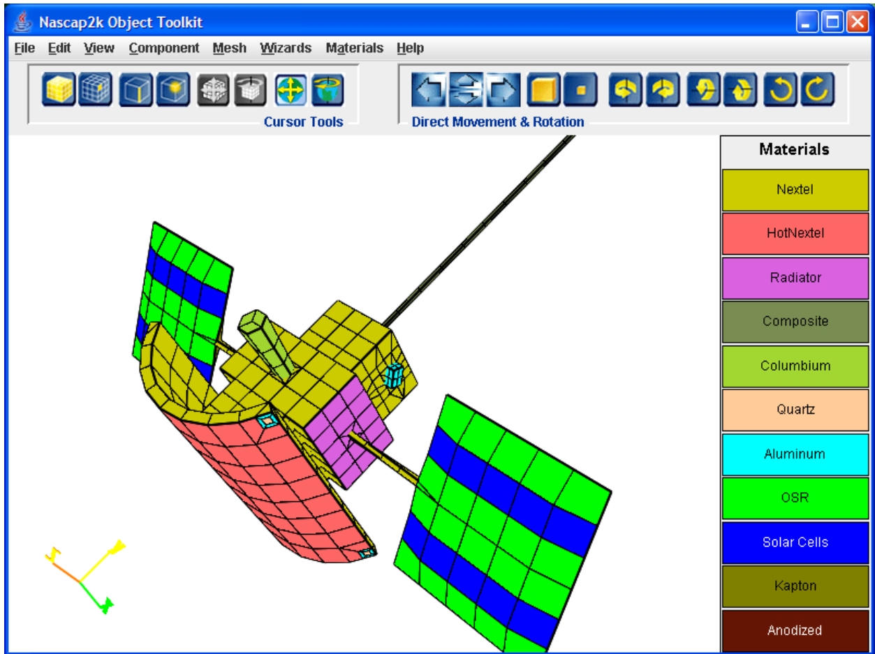
Figure 73. Object Toolkit Model of the MESSENGER Spacecraft.
