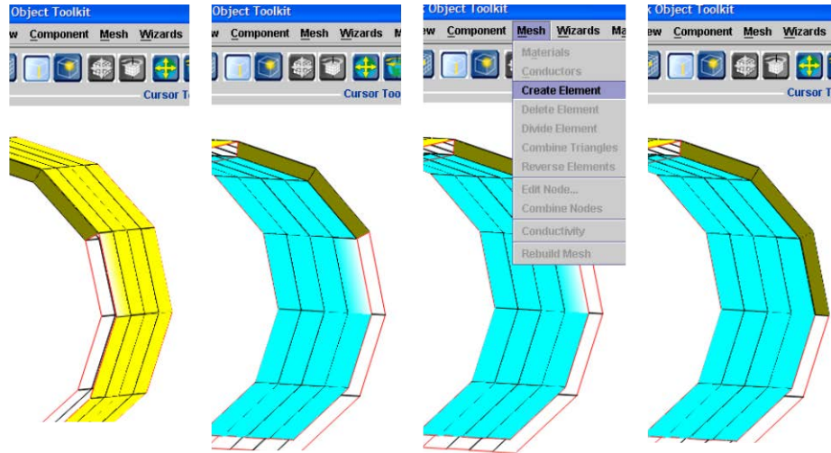
Figure 84. Creating an Element That Joins the Two Sides of the Sunshade. The Outlines of Elements with Normals Facing into the Screen Are Seen.
