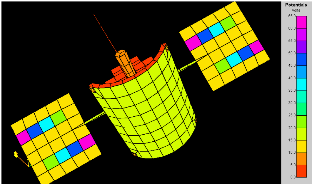
Figure 2. Nascap-2k Model of the MESSENGER Spacecraft, Showing Biased Solar Array Surfaces.
