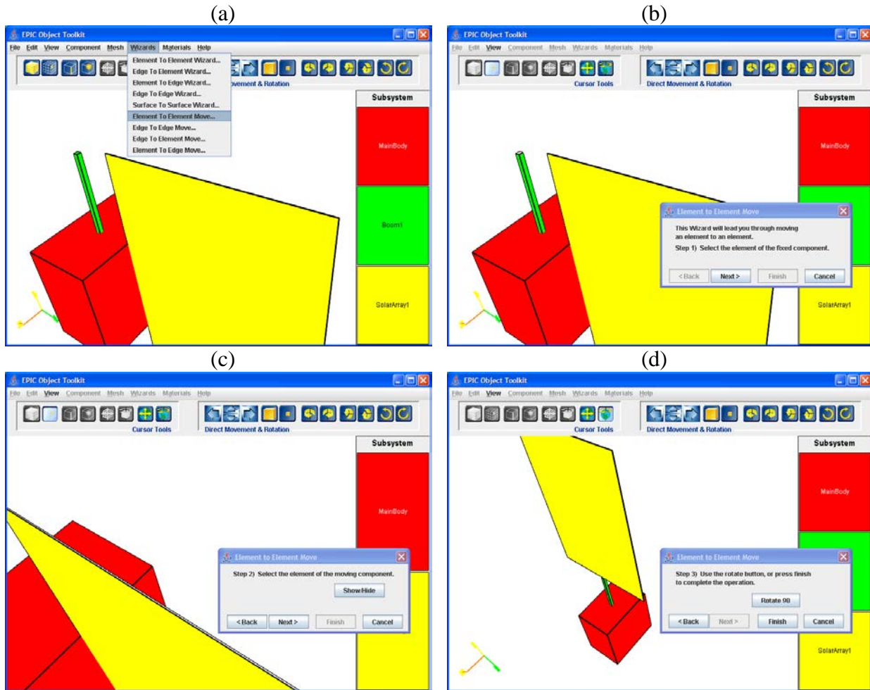
Figure 126. Placing the Solar Array at the End of the Boom Using the “Element to Element Move Wizard.”
