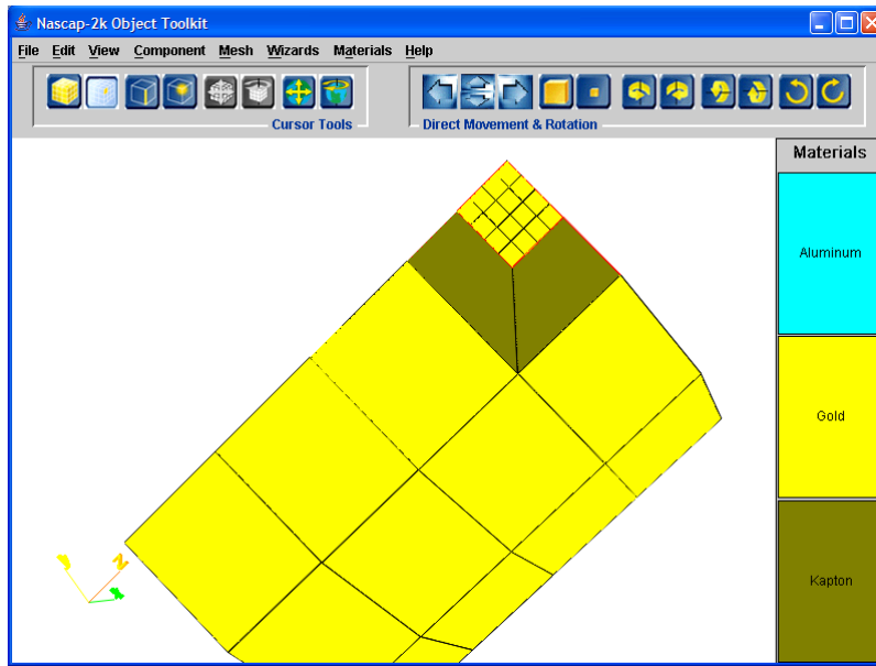
Figure 88. Result after Dividing the Corner Element and Then Dividing Each of the Newly Formed Elements.
