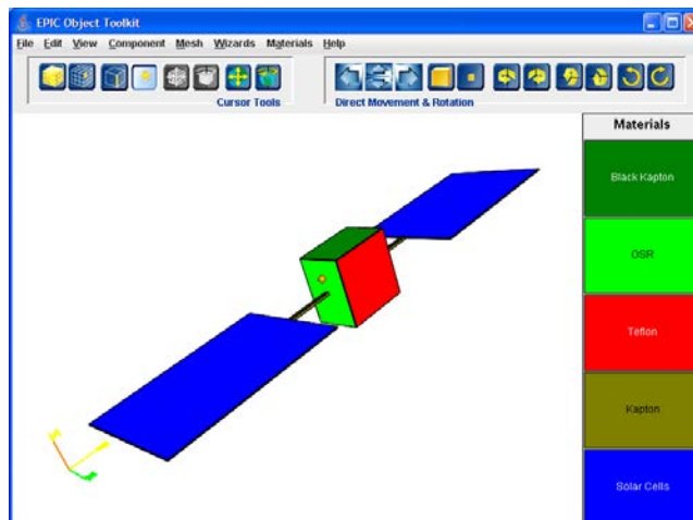
Figure 130. EPIC Object with Thruster. Thruster Is Located at (0.0, -1.4, 0.6) and Is Pointed in the -Y Direction.
