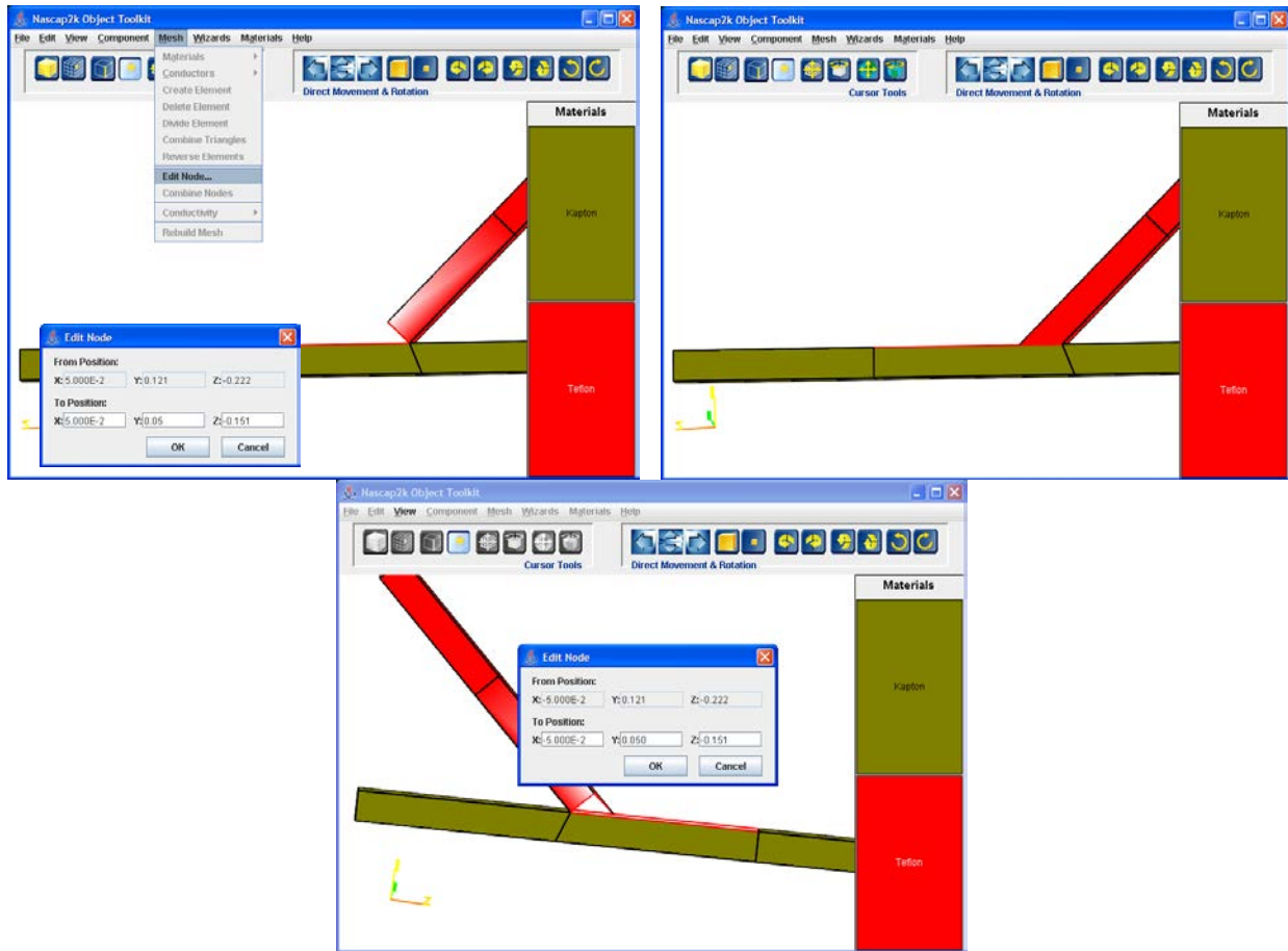
Figure 113. Moving End Nodes of the Short Boom to Be Along Face of the Long Boom. In These Figures, Perspective Is Turned Off.
