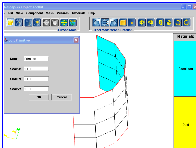
Figure 82. Scaling the Outer Edge by Expanding It in the X and Y Directions by 10%. The Outlines of Elements with Normals Facing into the Screen Are Seen.
