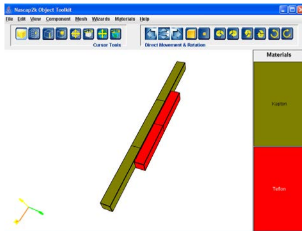
Figure 108. Booms to Be Connected into a Y Shape.
