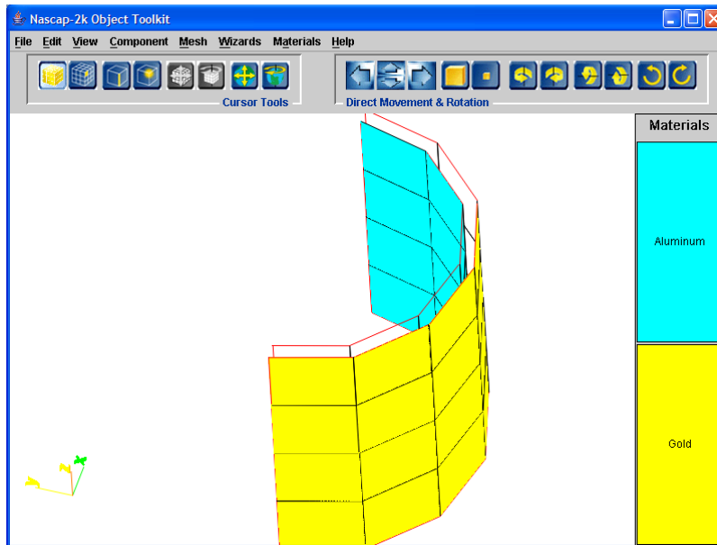
Figure 83. Resulting Inner and Outer Surfaces of the Sunshade. The Outlines of Elements with Normals Facing into the Screen Are Seen.
