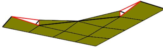
Figure 102. Filling in the Edge with Additional Triangular Elements, While Making Sure That the Two Sides Remain Separate. The Outlines of Elements with Normals Facing into the Screen Are Seen.
