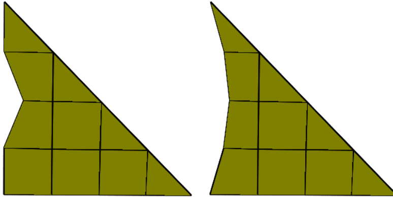
Figure 105. Moving Each Node to Form the Curved Edge by Going to the Mesh Menu and Choosing “Move Node.”
