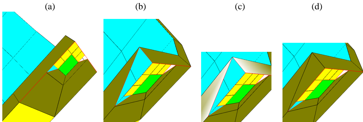
Figure 93. Replacing the Existing Side Element with Two New Elements, a Quadrilateral and a Triangle. The Outlines of Elements with Normals Facing into the Screen Are Seen.
