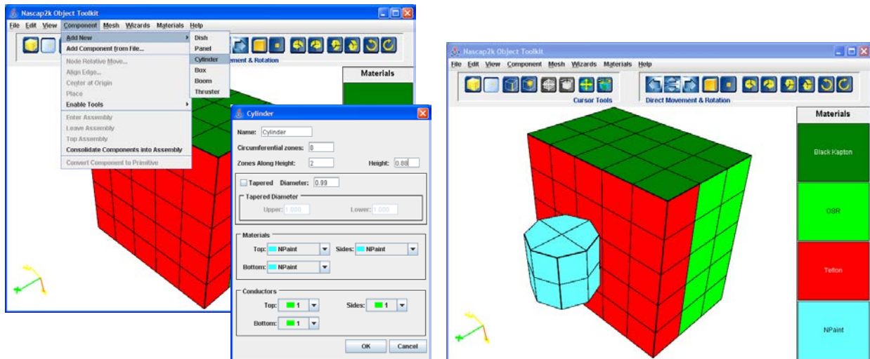
Figure 57. Defining a Cylinder to Represent the Omni-antenna. The Cylinder is 0.88 m in Height, 0.99 m in Diameter, Two Elements High, and Eight Elements in Circumference. All the Elements Are of the Newly Defined Material NPaint.
