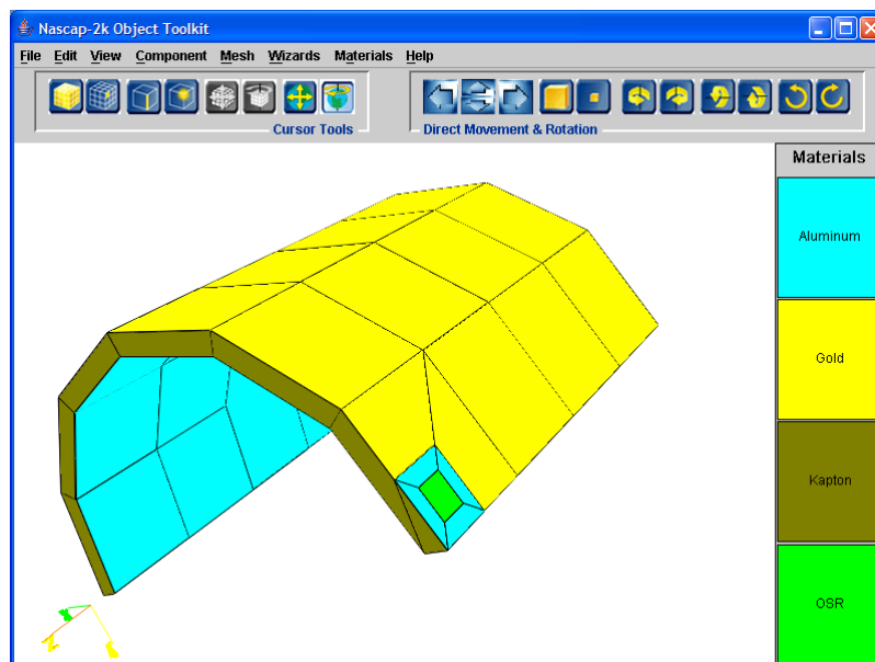
Figure 74. Simplified MESSENGER Sunshade, Including DSAD Instrument, to Be Built in this Example.
