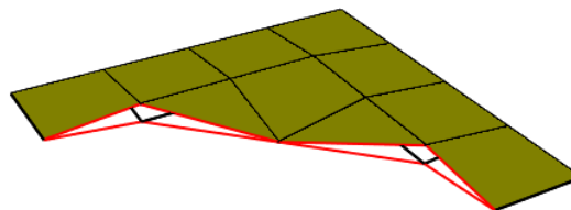
Figure 101. Closing the Open Edge in the Center By Going to the Mesh Menu and Choosing “Combine Nodes.” The Outlines of Elements with Normals Facing into the Screen Are Seen.
