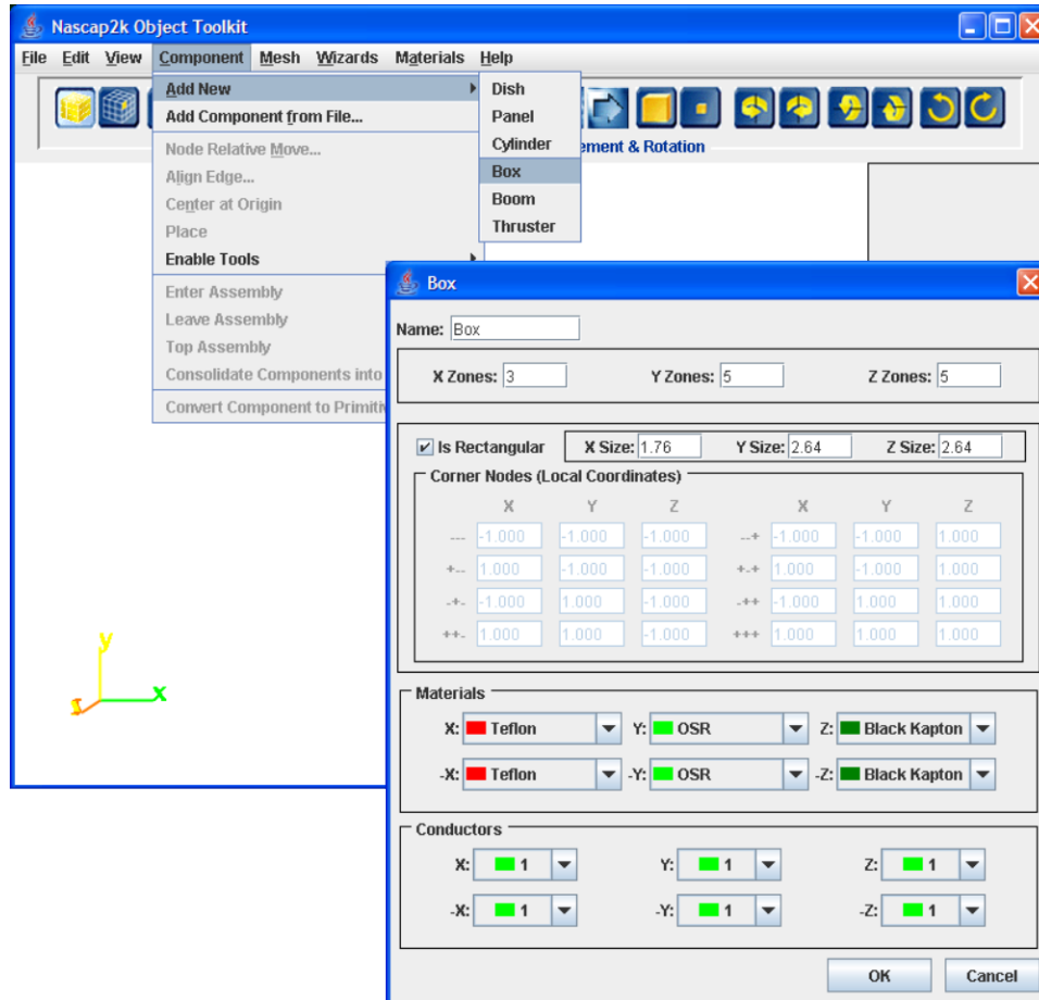
Figure 54. Defining a Box to Form the Body of the Spacecraft. The Box is 1.76 m by 2.64 m by 2.64 m in Size. Three Elements in the X Direction, and Five Elements in Each of the Other Two Directions. The \pm X Sides Are Teflon. The \pm Y Sides Are OSR. The \pm Z Sides Are Black Kapton.
