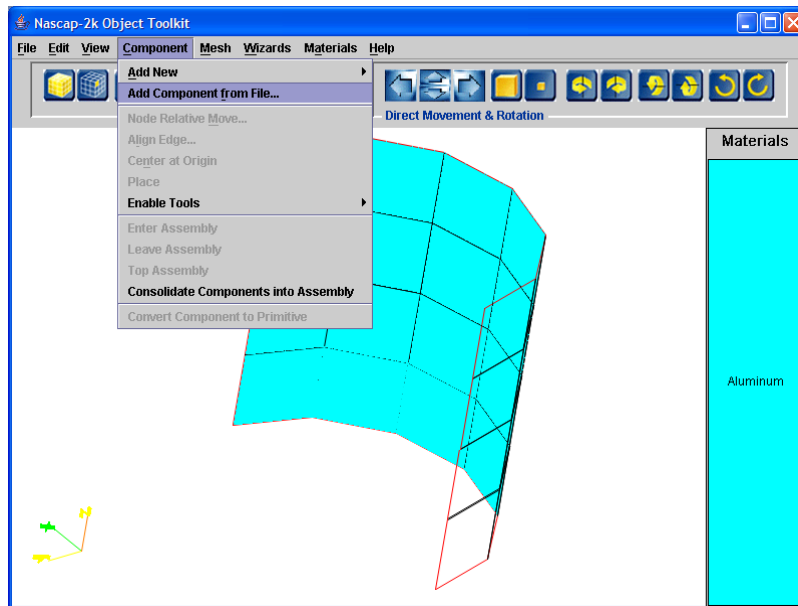
Figure 80. Adding the Outer Surface of the Sunshade from the Previously Saved File. The Outlines of Elements with Normals Facing into the Screen Are Seen.
