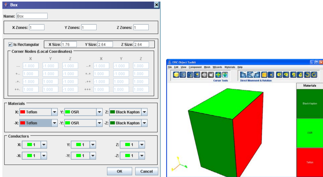
Figure 118. Specifying a Box to Represent the Main Body.
