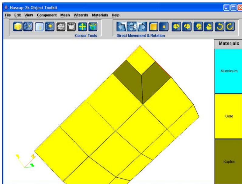
Figure 87. Result after Deleting Three Elements and Replacing Them with Two to Eliminate the Incompatibility along the Face of the Sunshade. Incompatible Elements Remain along the Edge.
