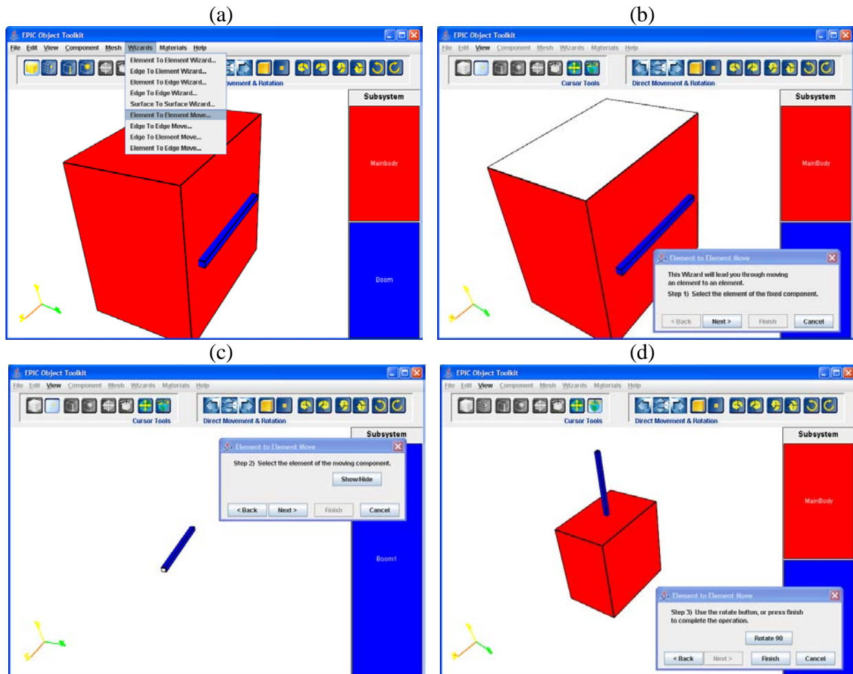
Figure 123. Placing the Boom Next to the Box Using the “Element to Element Move Wizard.”
