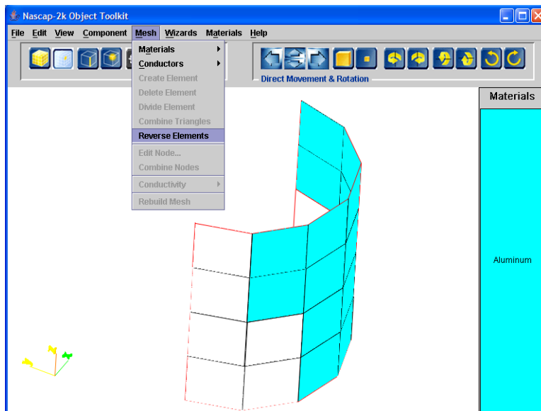
Figure 79. Reversing the Normal of the Elements. In the Figure, Some of the Distant Elements Have Already Been Reversed and Some of the Near Ones Have Been Selected and Are About to Be Reversed. The Outlines of Elements with Normals Facing into the Screen Are Seen.
