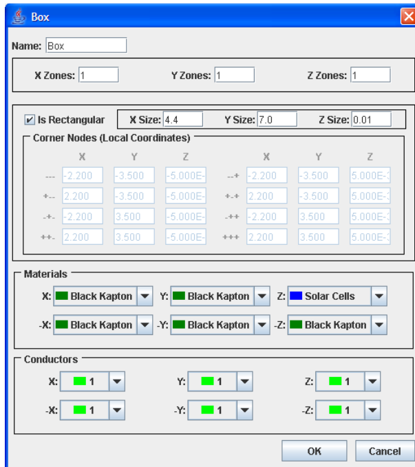
Figure 124. Solar Array for EPIC Object.
