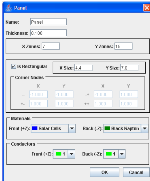
Figure 67. Defining a Panel to Represent a Solar Array Wing. The Panel Is 4.4 m in Width and 7 m in Length. It Is Seven Elements Wide and Fifteen Elements Long. The Front Side Is Material Solar Cells and the Back Is Black Kapton.
