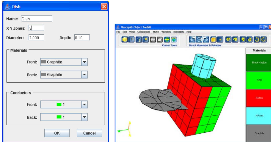
Figure 64. Defining Graphite Dishes to Represent the Dish Antennas. The Antenna Diameter Is 2 m, the Depth Is 0.1 m, and the Antenna Is Three Elements Across.
