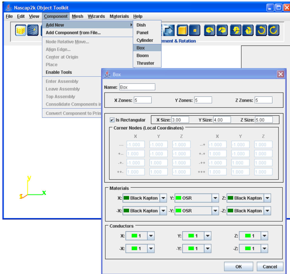
Figure 42. Dialog Box for Creating a Box 3.0 m by 4.0 m by 5.0 m in Size and Five Elements in Each Direction. The \pm Y Sides Are Defined to Be Material OSR and the Other Sides Are Black Kapton.
