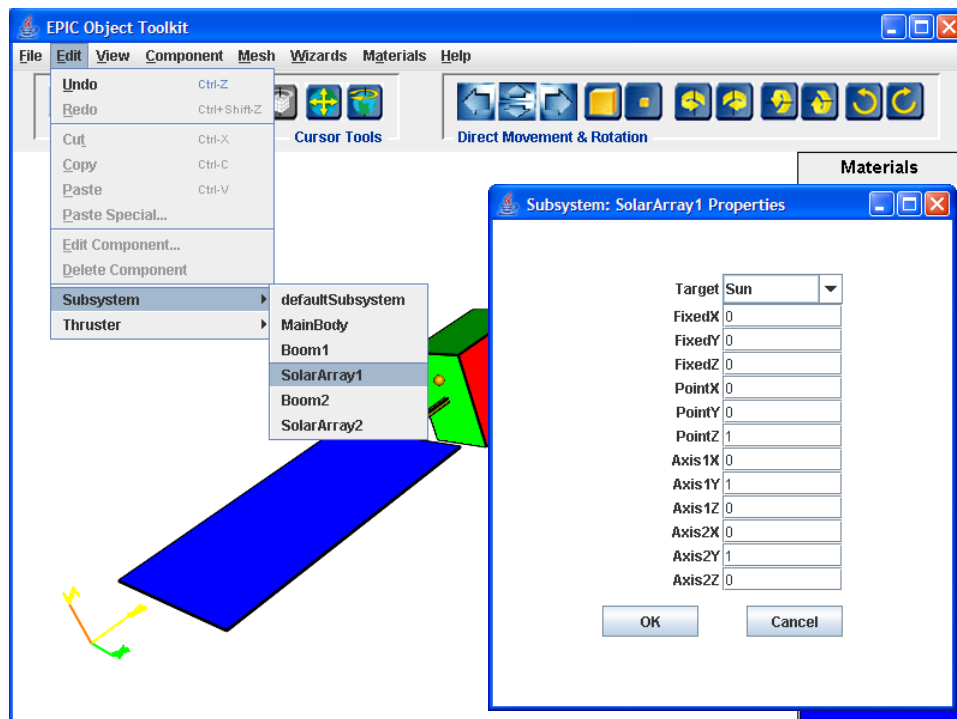
Figure 131. Setting SolarArray1 to Track the Sun. The Fixed Point Is (0.0, 0.0, 0.0). The Pointing Vector Is (0.0, 0.0, 1.0). The First Axis Is (0.0, 1.0, 0.0) and the Second Axis Is the Same.
