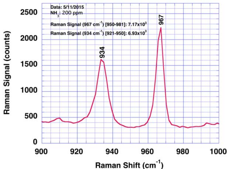
FIG. 3. Raman spectrum (average of 9 scans) for the 934 and 967\text{ cm}^{-1} modes of 200\text{ ppm NH}_3 obtained with 10\text{ W} laser power and 15\text{ s} signal integration time for each scan.
