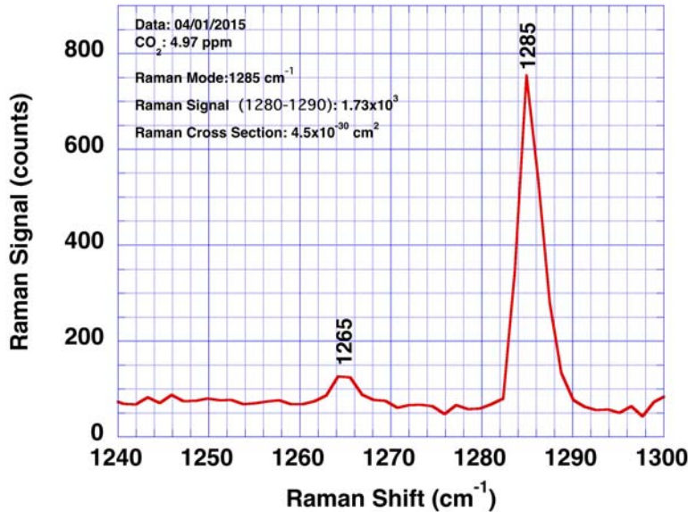
FIG. 2. Raman spectrum (average of 9 scans) for the 1265 and 1285 \text{cm}^{-1} modes of 5 ppm \text{CO}_2 obtained with 10 W laser power and 15 s signal integration time for each scan.
