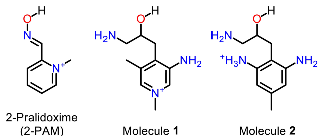
Figure 1. An approved oxime antidote, 2-pralidoxime (2-PAM), and two \beta -aminoalcohol molecules ( molecules 1 and 2 ) considered in the present study as reactivators of the aged sarin-/soman-inhibited acetylcholinesterase (AChE) adduct.
