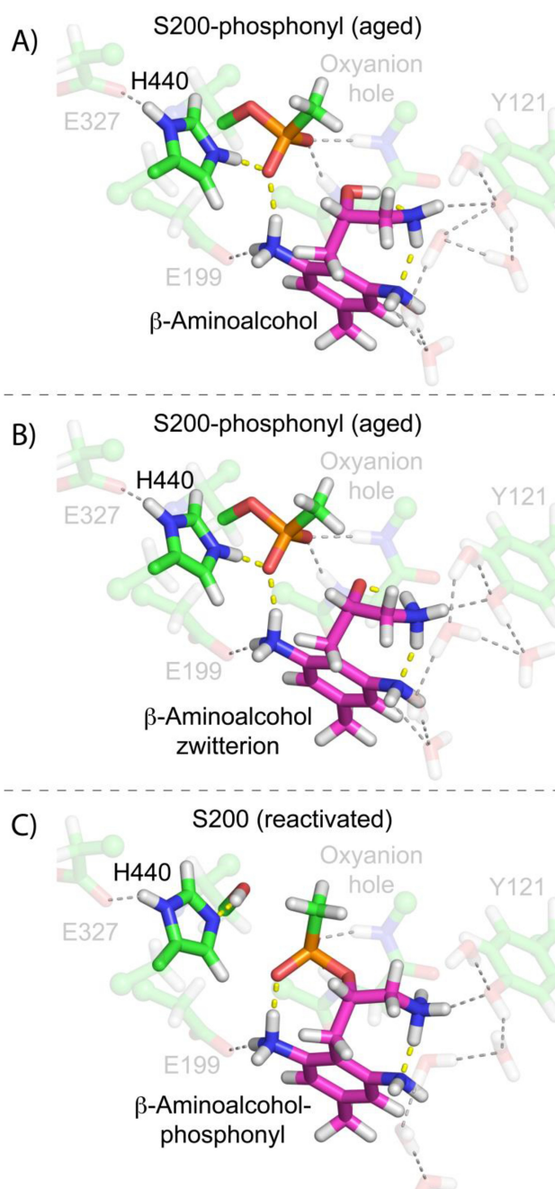
Figure 2. Representative structures along the reaction path for reactivation of aged sarin/soman-inhibited AChE adduct with \beta -aminoalcohol molecule 2 . A) Complex of aged AChE with molecule 2 . B) Metastable zwitterionic intermediate of \beta -aminoalcohol molecule 2 . C) Reactivated AChE bound to the adduct of \beta -aminoalcohol molecule 2 with the aged phosphonyl moiety of sarin/soman. Only atoms that are included in the quantum mechanical (QM) region of the QM/molecular mechanical calculation are shown. Carbon atoms of the aged AChE adduct are depicted in green. Carbon atoms of \beta -aminoalcohol molecule 2 are shown in magenta. Hydrogen, nitrogen, and oxygen atoms are white, blue, and red, respectively. Peripheral hydrogen bonds are shown with dashed gray lines, whereas those of particular relevance for reactivation are shown with yellow dashed lines. Residues of the active site not directly involved in the reaction are shown in faded, transparent colors. Atoms that link the QM region to the rest of the system described by molecular mechanics are depicted with transparent spheres around them. These atoms are substituted for hydrogen atoms, and their bond lengths are adjusted accordingly during QM calculations.
