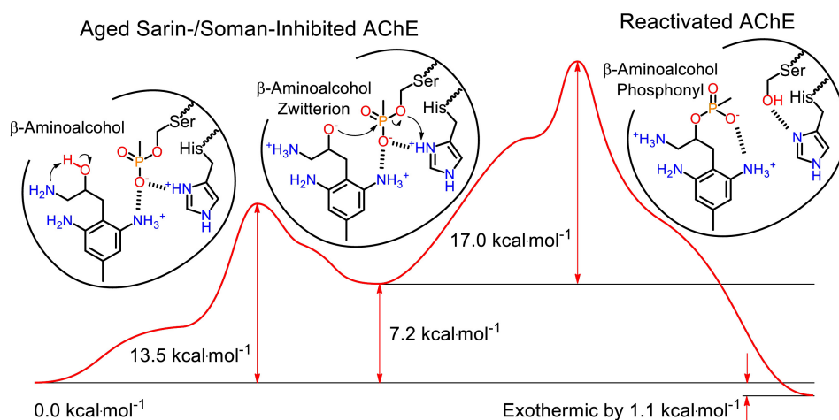
Figure 3. Steps and energetics of aged sarin-/soman-inhibited AChE reactivation with \beta -aminoalcohol molecule 2.
