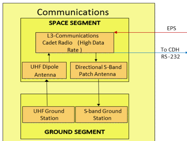
Figure 155: Communications architecture
