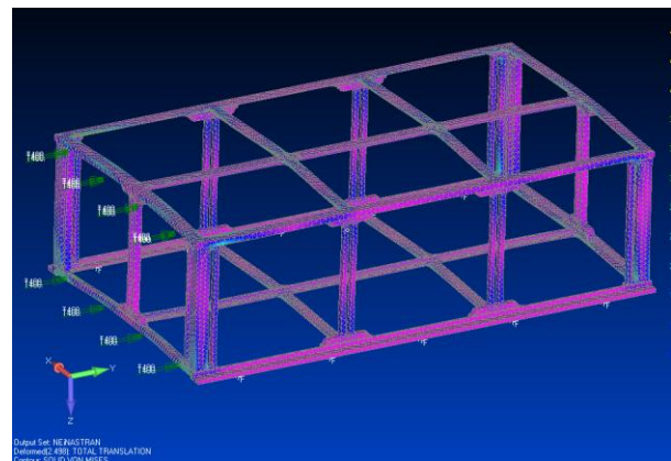
Figure 20: FEA of 400N applied to the -Z face
