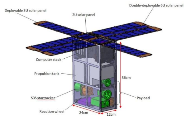
Figure 1: CAD model of the ARAPAIMA Cubesat
