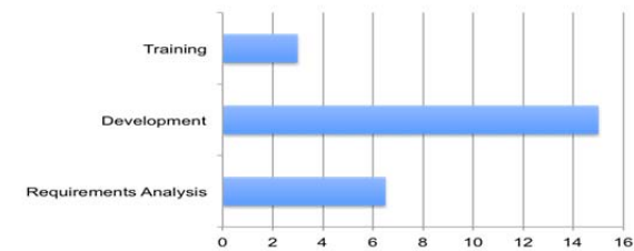
Figure 10: Time Statistics
