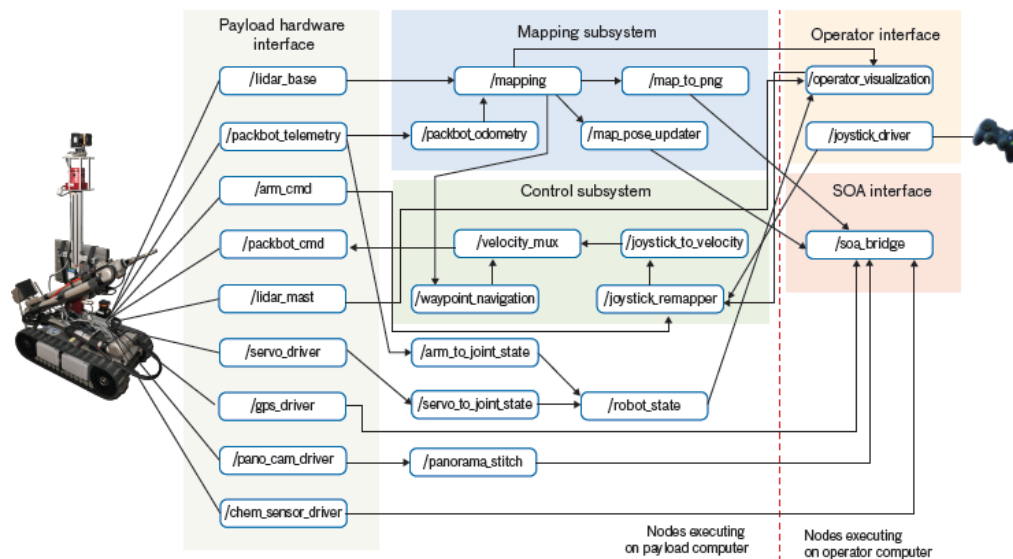
FIGURE 6. The RASR enhanced situational payload computational graph consists of named executing modules, or nodes (rounded boxes), that are connected by data streams, or topics (arrowed lines between boxes). For the sake of clarity, this figure groups related ROS nodes, such as those for the payload hardware interface and the mapping subsystem.
