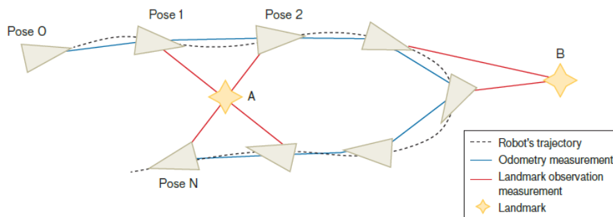
FIGURE 7. A robot navigating an unknown environment can represent its history as a graph.
