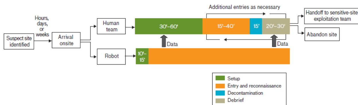
FIGURE 3. A human team and robot operate in parallel to perform reconnaissance of a sensitive site. In contrast to the extensive setup required for manned entry, setup for the unmanned ground vehicle (UGV) is minimal: the UGV has to be unpacked from its case and powered up, and sensors may need to be attached if they are not permanently integrated on the platform. Because of its quick setup, the UGV can begin collecting data in the hot zone soon thereafter the SSA unit arrives onsite. A UGV can provide an early look at the site prior to manned entry and perform persistent reconnaissance when the manned entry team is outside of the hot zone.
