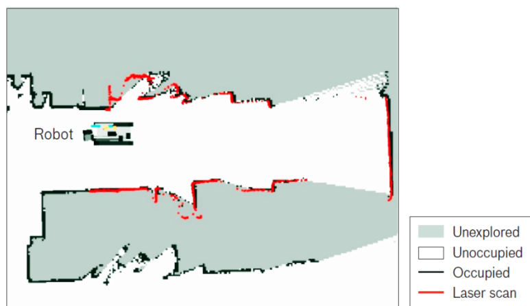
FIGURE 8. A grid map was computed by the Rapid Area Sensitive-Site Reconnaissance mapping subsystem as the robot moved to the right of the figure.
