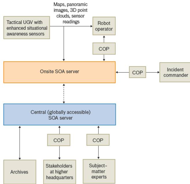
FIGURE 4. The Rapid Area Sensitive-Site Reconnaissance system architecture supports multiple sites and many geographically distributed users with a decentralized design that maintains consistency in information shared between users when interconnecting communication links become available.
