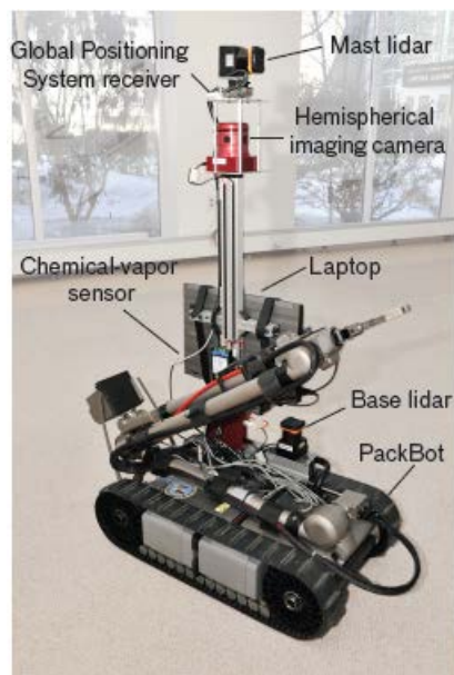
FIGURE 5. The enhanced situational awareness payload prototype includes a vertical mast, two lidars, a camera, and a chemical sensor.
