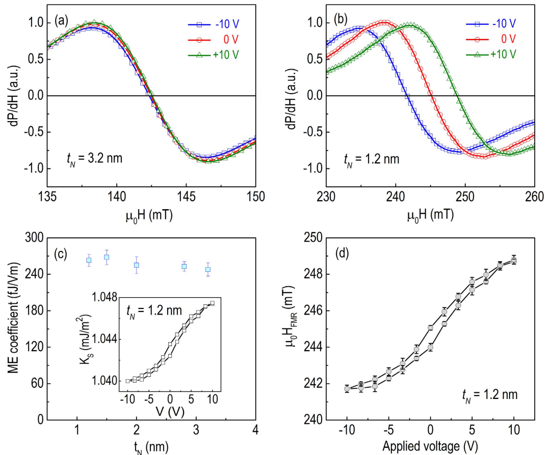
Figure 2. Modification of FMR spectra by constant voltages. (a,b) Voltage-induced shift of FMR spectra for NiFe/PLZT with (a) t_N = 3.2 nm and (b) t_N = 1.2 nm. (c) Dependence of the ME coupling coefficient on NiFe thickness t_N , the inset is the magnetic surface anisotropy K_S as a function of applied voltage. (d) Resonance field as a function of applied voltage for NiFe/PLZT with t_N = 1.2 nm.
