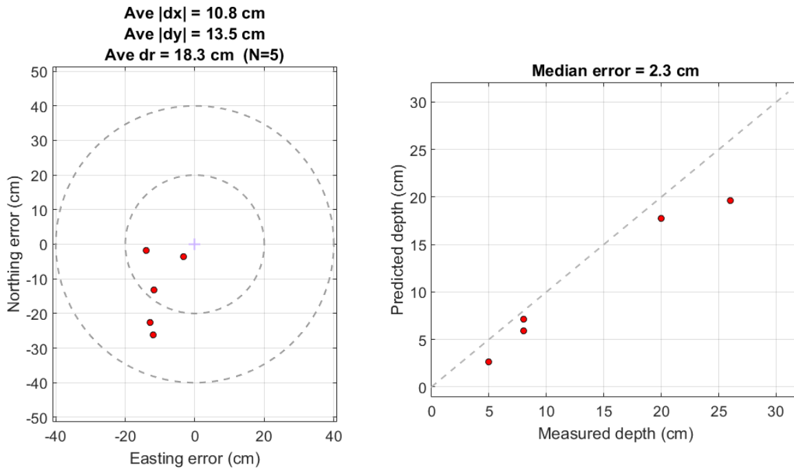
Figure 15: Comparison of source locations and depths predicted by inversions of MPV3D data from the 69-1745 Puako Drive property with the ground truth locations and depths measured during intrusive operations.
