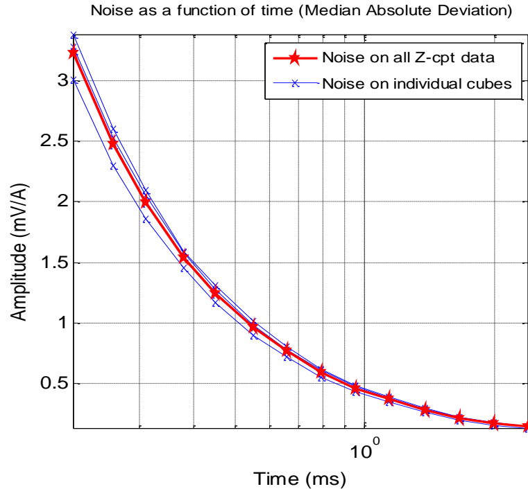
Figure 19: Noise analysis for 69-1765 Puako Drive. The noise is twice as high (2.5mV/A) as 69-1745 Puako Drive (1.2 mV/A).
