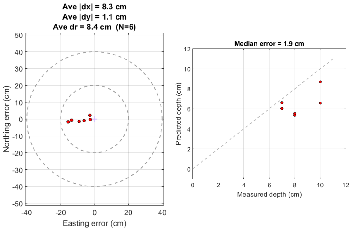
Figure 39: Comparison of source locations and depths predicted by inversion of MPV3D data from the 69-1951 Puako Drive property with the ground truth locations and depths measured during intrusive operations.
