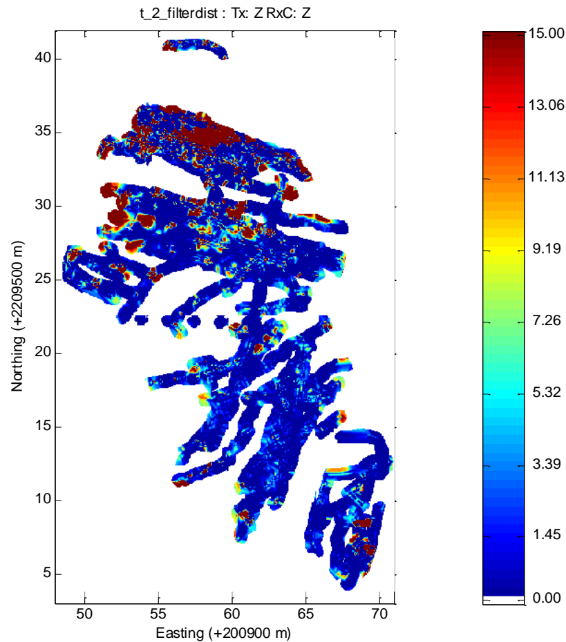
Figure 42: Gridded image of detection channel for 69-1971 Puako Drive when surveying underneath significant tree canopy.
