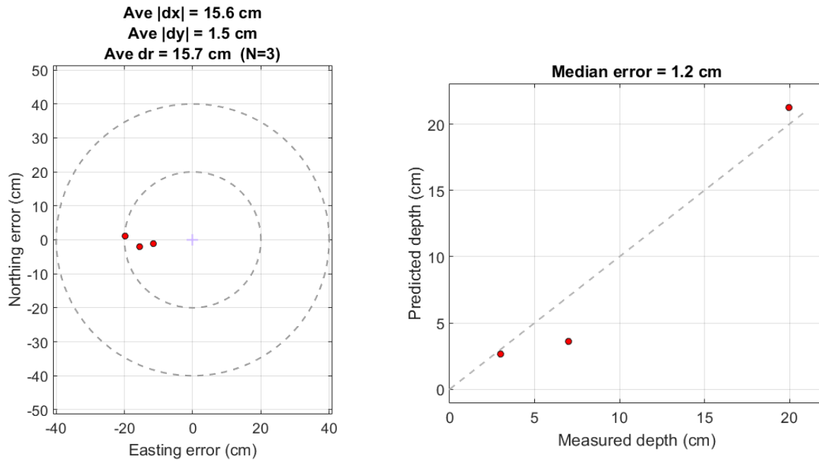
Figure 33: Comparison of source locations and depths predicted by inversions of MPV3D data from the 69-1877 Puako Drive property with the ground truth locations and depths measured during intrusive operations.
